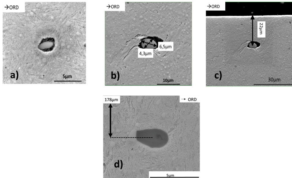
Fig. 2. (a) Example of non-metallic inclusion debonded from the matrix, (b) determination of size, and (c) depth below the surface. (d) Fully bonded inclusion, located 178 µm from the raceway surface.
