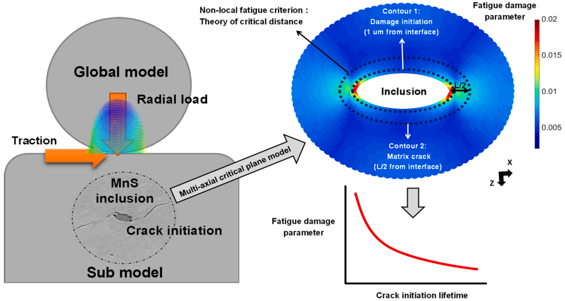
Fig. 4. Numerical RCF driven damage initiation lifetime model (Representation is not to scale).
