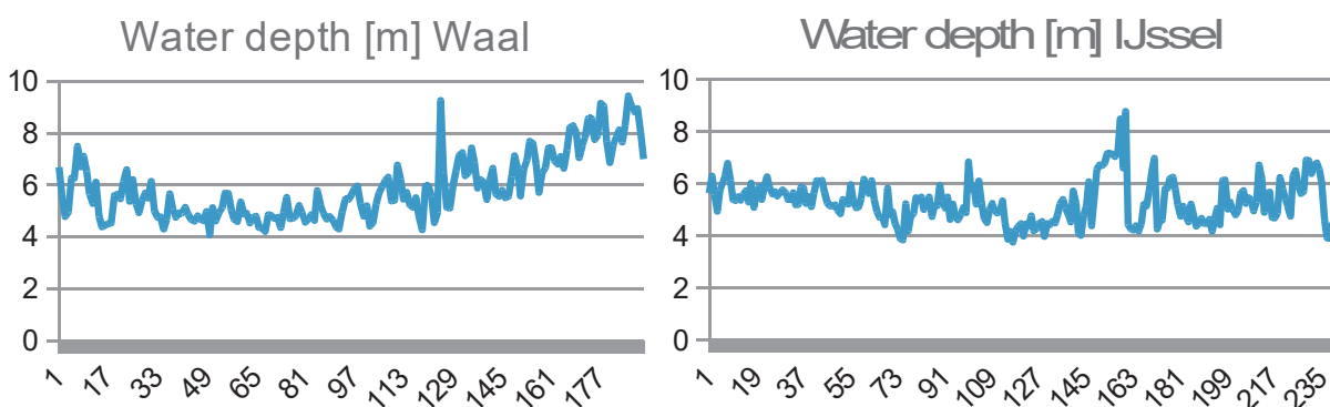
Figuur 3 Water depths along the Waal (16-9-2085) and IJssel (15-9-2085)
