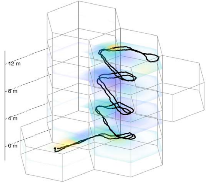
Fig. 4. Example showing the three-dimensional nature of our SLAM algorithm. The path covers a flight of stairs in the University of Cambridge Engineering Department. The complete path length is 125 meters. The cross-sections of the tiles show the magnetic map norm (the color scale is the same as in Fig. 3(f)).
