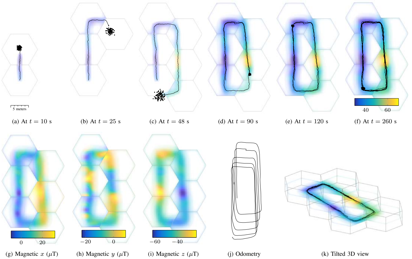
Fig. 3. The SLAM solution for walking in a square for several loops for around 250 meters. Subfigures (a)–(f) show the norm of the magnetic field map for the highest weight particle. The transparency of the maps scales with the marginal variance of the GP map. Subfigures (g)–(i) show the corresponding vector field components for the final map in (f). The odometry trajectory is visualised in (j), and (k) shows the 3D hexagonal tiles with a cross-section of the magnetic field maps.
