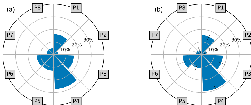
FIG. 3. (a) A fictional example of an individual fingerprint that was computed using eight representatives. Each bar represents the occurrence rate of the corresponding class of profiles that are associated with the representative, and each concentric circle is a 10% interval. (b) A fictional example of an aggregated fingerprint that was computed using eight representatives. Each bar represents the median occurrence rate of the corresponding class of profiles, and each error bar corresponds to the 90% confidence interval for the occurrence rate for points in the cluster. The PX labels in the squares refer to hypothetical representatives of the example.
