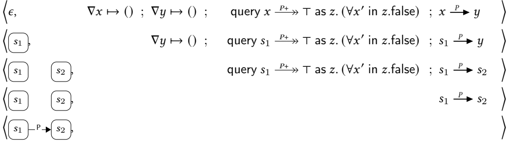
Fig. 9. Trace demonstrating unsoundness of a naive query simplification rule.
