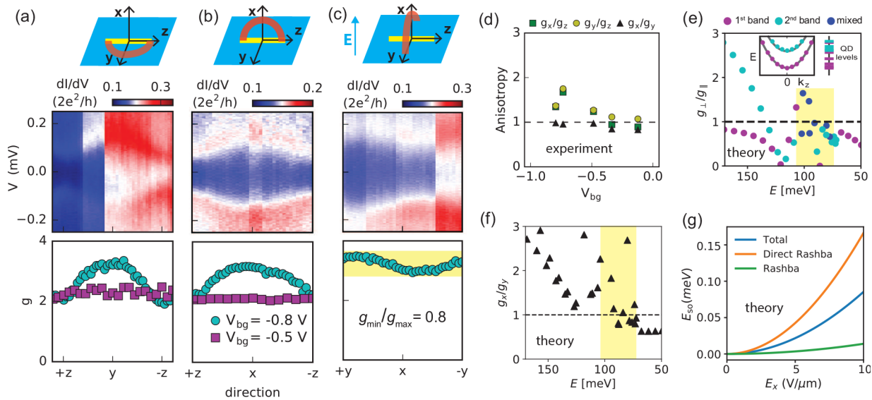
Figure 3. (a–c) Rotations of the magnetic field with a 0.9 T magnitude in the yz-, xz-, and xy-plane, respectively, at V_{bg} = -0.79 V. The upper panel shows the schematic of the device and the magnetic field rotation performed. The differential conductance data is plotted in the center panel, and the splitting of the Kondo peak changes as the angles are swept. The sudden changes in conductance are due to small switches in V_{bg} . The lower panel shows the extracted g of the center panel in cyan and g at V_{bg} = -0.5 V in magenta. For the xy-plane, the anisotropy is highlighted and calculated. (d) Summary of the measured anisotropies of g at a different V_{bg} . (e) Simulation result of the quantum dot. The anisotropy of g_{\parallel} and g_{\perp} changes as the Fermi energy is altered. The colors represent the band from where the quantum dot level predominantly stems. The highlighted part shows a similar behavior in the anisotropy values as the data in part d. The inset depicts a schematic representation of the energy ordering of the quantum dot levels originating from two bands along the NW. (f) Simulation as in part e, now with an applied electric field of 10 V/ \mu m. The SOI causes anisotropy with respect to the electric field direction as g_x is pointed perpendicular and g_y parallel to the electric field. The anisotropy increases as the Fermi level is raised. The same range as in part e is highlighted. (g) Simulated spin-orbit energies for the first band ( k = 0 ) of the infinite wire model as a function of the electric field along the x-direction. The direct Rashba term is the leading contribution.
