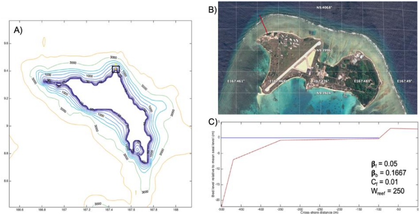
Fig. 3. Morphology of the study area. A) Kwajalein Atoll and bathymetric contours. B) Google Earth image of Roi-Namur, the northernmost part of the atoll, and the location of the cross-shore transect. C) Cross-shore transect (adapted from Quataert et al. , 2015)
