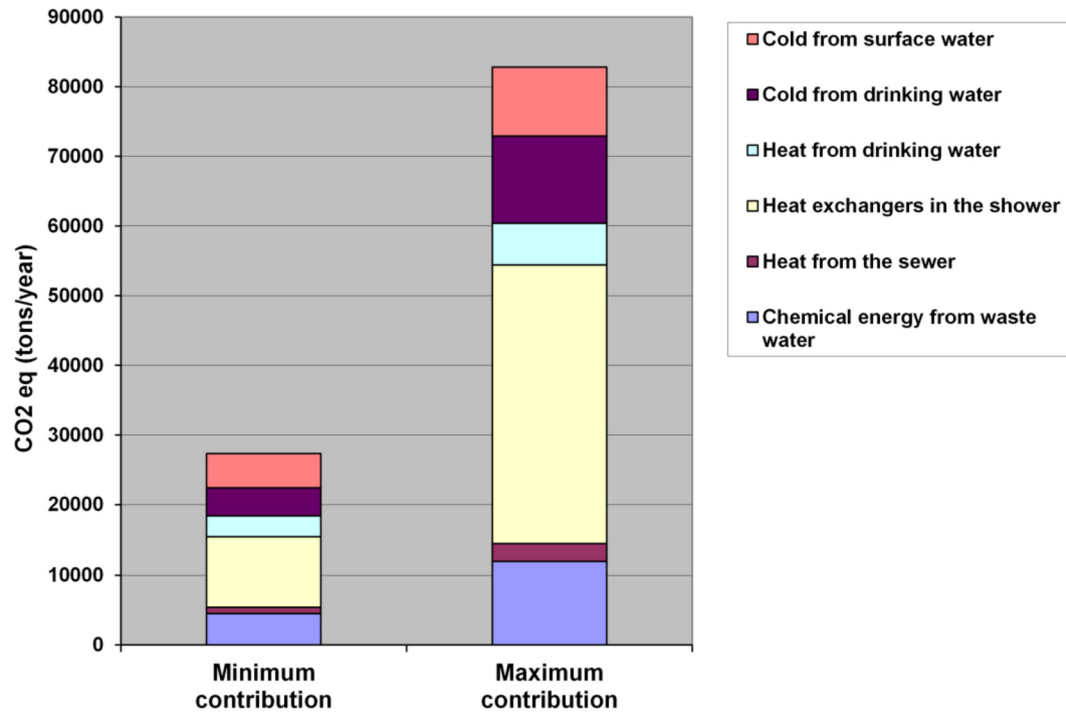
Fig. 3. Energy recovery from the water cycle in Amsterdam, expressed as avoided greenhouse gas emissions (reprinted from Journal of Water and Climate Change, volume 5, Issue 1, pages 61–69, with permission from the copyright holders, IWA Publishing).
