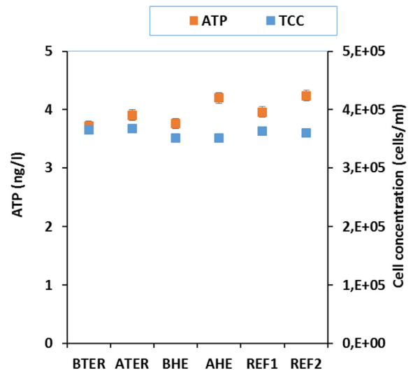
Fig. 7. Microbiological water quality in DWDS 1 (BTER: before thermal energy recovery; ATER: after thermal energy recovery), DWDS 2 (BHE: before heat exchanger; AHE: after heat exchanger) and DWDS 3 (REF1: at start of DWDS; REF2: at end DWDS) (n = 29).
