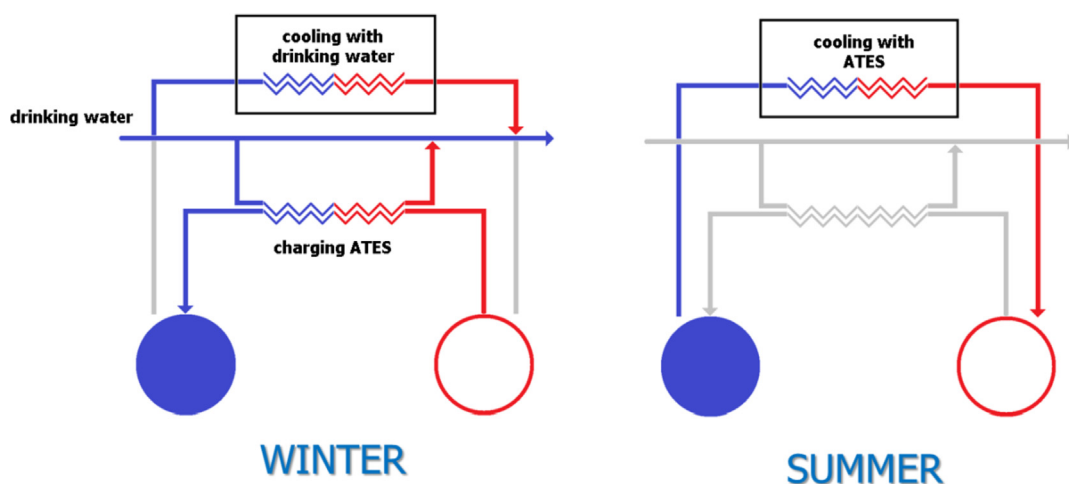
Fig. 6. Process set-up of cooling with drinking water under winter and summer conditions.
