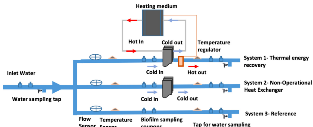
Fig. 4. Laboratory scale drinking water distribution systems.
