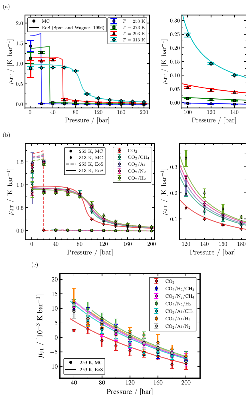
Figure 7. Computed Joule–Thomson coefficients as a function of temperature and pressure. (a) The calculated Joule–Thomson coefficients of pure \text{CO}_2 from MC simulations (closed symbols) and the Span and Wagner EoS 23 (solid lines) for temperatures of 253, 273, 293, and 313 K. (b) Joule–Thomson coefficients of binary mixtures with 95 mol % \text{CO}_2 and 5 mol % impurities ( \text{CH}_4 , Ar, \text{N}_2 , and \text{H}_2 ) computed from MC simulations (closed symbols) and the GERG-2008 EoS 24 (lines) compared with Joule–Thomson coefficients of pure \text{CO}_2 computed from MC simulations and the Span and Wagner EoS 23 for temperatures of 253 and 313 K. (c) Joule–Thomson coefficients of ternary mixtures with 96 mol % \text{CO}_2 and 2 mol % impurities for each of two components ( \text{CH}_4 , Ar, \text{N}_2 , and \text{H}_2 ) computed from MC simulations (closed symbols) and the GERG-2008 EoS 24 (lines) compared with Joule–Thomson coefficients of pure \text{CO}_2 computed from MC simulations and the Span and Wagner EoS 23 at 253 K.
