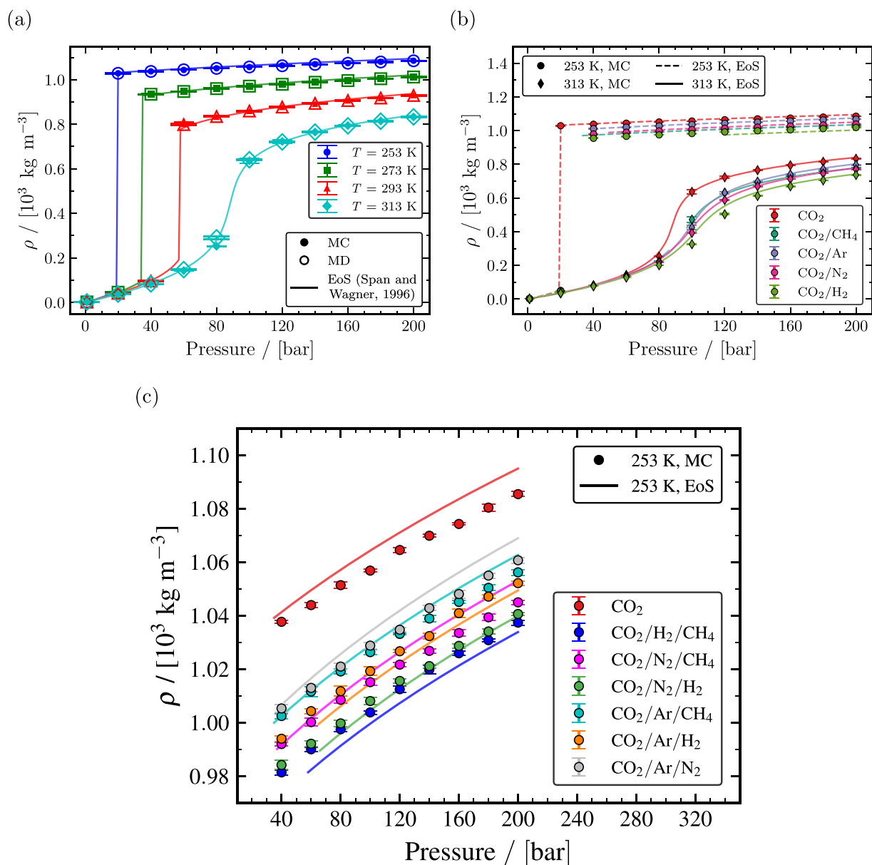
Figure 2. Computed densities as a function of temperature and pressure. (a) The calculated densities of pure \text{CO}_2 from MC simulations (closed symbols), MD simulations (open symbols), and the Span and Wagner EoS 23 (solid lines) for temperatures of 253, 273, 293, and 313 K. (b) Densities of binary mixtures with 95 mol % \text{CO}_2 and 5 mol % impurities ( \text{CH}_4 , Ar, \text{N}_2 , and \text{H}_2 ) computed from MC simulations (closed symbols) and the GERG-2008 EoS 24 (lines) compared with densities of pure \text{CO}_2 computed from MC simulations and the Span and Wagner EoS 23 for temperatures of 253 and 313 K. (c) Densities of ternary mixtures with 96 mol % \text{CO}_2 and 2 mol % impurities for each of two components ( \text{CH}_4 , Ar, \text{N}_2 , and \text{H}_2 ) computed from MC simulations (closed symbols) and the GERG-2008 EoS 24 (lines) compared with densities of pure \text{CO}_2 computed from MC simulations and the Span and Wagner EoS 23 at 253 K.
