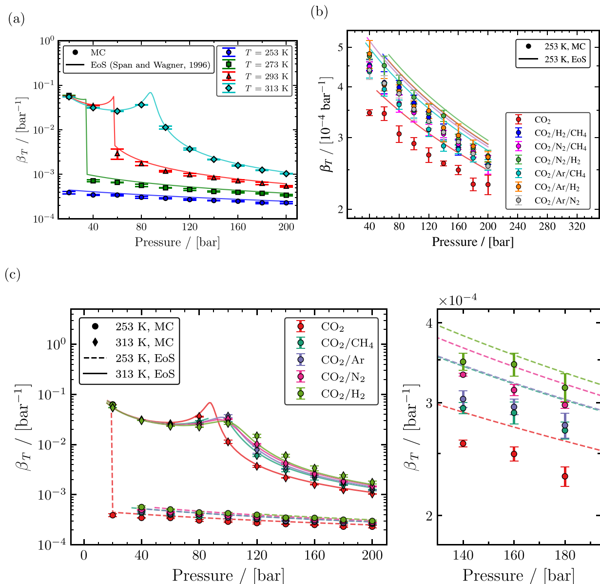
Figure 4. Computed isothermal compressibilities as a function of temperature and pressure. (a) The calculated isothermal compressibilities of pure \text{CO}_2 from MC simulations (closed symbols) and the Span and Wagner EoS 23 (solid lines) for temperatures of 253, 273, 293, and 313 K. (b) Isothermal compressibilities of ternary mixtures with 96 mol % \text{CO}_2 and 2 mol % impurities for each of two components ( \text{CH}_4 , \text{Ar} , \text{N}_2 , and \text{H}_2 ) computed from MC simulations (closed symbols) and the GERG-2008 EoS 24 (lines) compared with isothermal compressibilities of pure \text{CO}_2 computed from MC simulations and the Span and Wagner EoS 23 for temperatures of 253 and 313 K. (c) Isothermal compressibilities of binary mixtures with 95 mol % \text{CO}_2 and 5 mol % impurities ( \text{CH}_4 , \text{Ar} , \text{N}_2 , and \text{H}_2 ) computed from MC simulations (closed symbols) and the GERG-2008 EoS 24 (lines) compared with isothermal compressibilities of pure \text{CO}_2 computed from MC simulations and the Span and Wagner EoS 23 at 253 K.
