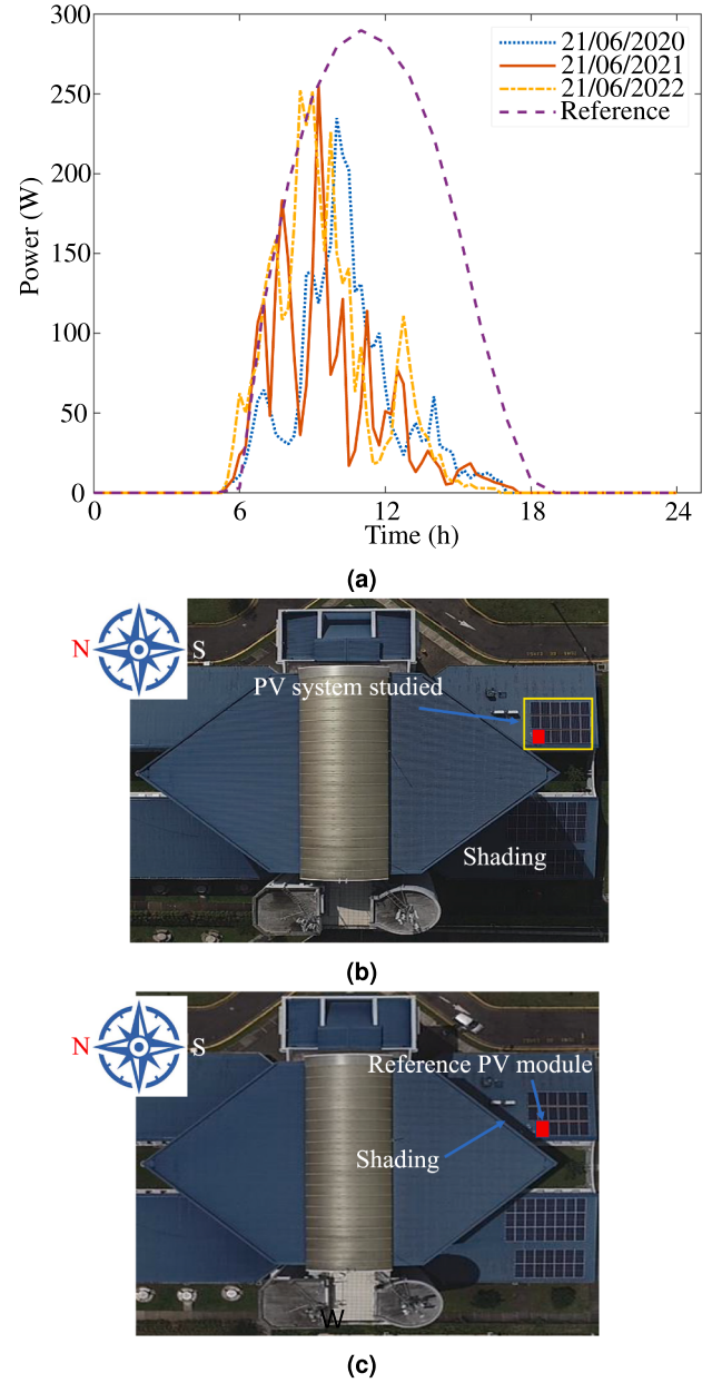
Fig. 7. (a) Power generation of the reference PV module for the 21 st of June (2020, 2021, and 2022), aerial images for the 21 st of June 2022, (b) at 8:00 am, and (c) at 11:30 am.
