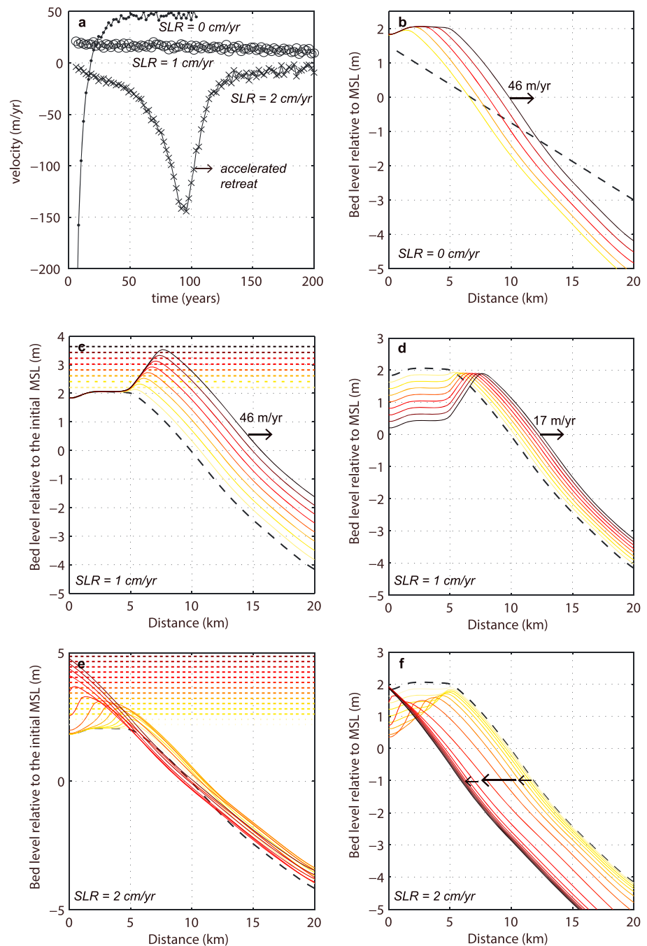
Figure 4. (a) Evolution of the migration speed inside a reference frame that rises vertically with MSL for the simulations in panels (b) (no sea level rise, indicated by dots), (d) (SLR = 1 cm/year, indicated by circles), and (f) (SLR = 2 cm/year, indicated by crosses). c_b = 0.15 g/L. (c–f) Evolution from the equilibrium profile of panel (b) with time steps of 20.4 years over 165 years (panels (c) and (d)) and with steps of 10.2 years over 165 years (panels (e) and (f)). (b, c, and e) The evolution in a static reference frame, from the dashed initial profile via light yellow to dark red. The dotted lines indicate the top of the tidal range. (d and f) The evolution inside a rising reference frame. SLR = sea level rise; MSL = mean sea level.
