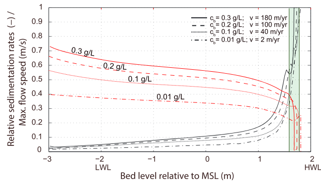
Figure 2. Simulated maximum tidal flow velocities during flood tide (red lines) and relative net sedimentation rates (black lines, i.e., the net vertical flux divided by the gross deposition flux) on a steadily prograding intertidal flat (i.e., after a spin-up) for different (constant) sediment concentrations at the open boundary (at MSL -3 m). In the steadily prograding state, balances are most precise at the open boundary and are increasingly disturbed toward the top of the flat. We here define the “top of the flat” as the elevation just before the flow velocity becomes zero (for the different simulations this occurs within the green marked domain). The numerical model is based on the conservation equations for mass and momentum (capturing the hydrodynamics) and the advection-dispersion equation (capturing the dynamics of the concentration field) and further explained in Maan et al. (2015). MSL = mean sea level; LWL = low water line; HWL = high water line.
