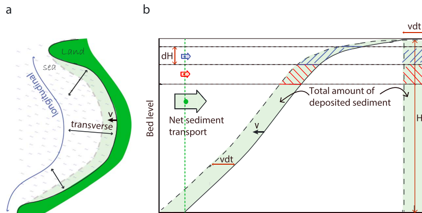
Figure 1. (a) Conceptual sketch of the domain declaring the longitudinal (parallel to the isobaths) and transverse (perpendicular to the isobaths) directions. (b) The principle of conservation of sediments on a prograding intertidal flat. The net landward sediment flux (green arrow) is equal to the amount of net deposited sediment, hence: v \int_0^T H \rho = \int_0^T h(t) u(t) c(t) dt . Because the celerity is uniform, this constraint also holds per (unit) layer dH . Taking H = a - z and h(t) = \eta(t) - z (with a the tidal amplitude, z the bed level and \eta the water level) and differentiate with respect to z gives equation (1).
