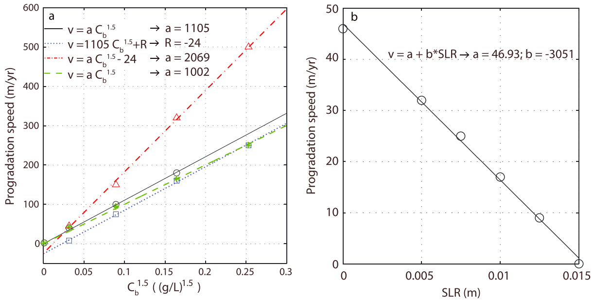
Figure 3. (a) Simulated steady progradation speeds of intertidal flats versus the suspended sediment concentration in the adjacent waters (see Maan et al., 2015, for a description of the model). Data set 1 (black circles) is for tidal currents only, while the other data sets include 20 cm wind waves. Run 2 (blue squares) and Run 3 (red triangles) differ in the fall velocity, w_s = 0.2 \cdot 10^{-3} m/s for set 2 and w_s = 0.5 \cdot 10^{-3} m/s for set 3. Run 2 and Run 4 (green stars) differ in the dispersion coefficient K . K = 100 m 2 /s 2 for set 2 and K = 1 m 2 /s 2 for set 4. Every data set is fitted for one free parameter in the indicated function. Coefficient a in the second fit is obtained from the first fit, while coefficient R in the third is obtained from the second fit, that is, it is assumed that the presence of waves does not affect a , and that w_s does not affect the wave-related R term. For set 4 ( K = 1 m 2 /s 2 ) the data could be fitted without R . (b) Linear relationship between the rate of SLR and the progradation speed based on model simulations (Maan et al., 2015) for c_b = 0.15 g/L. SLR = sea level rise.
