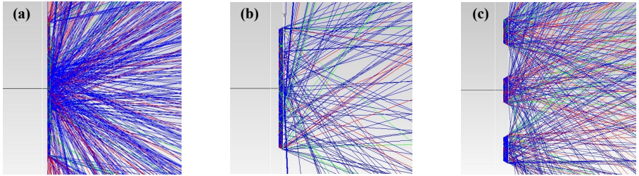
Figure 2.17: Light ray tracing results (side view), (a) planar design, (b) single cavity reflector, and (c) individual cavity reflector.
