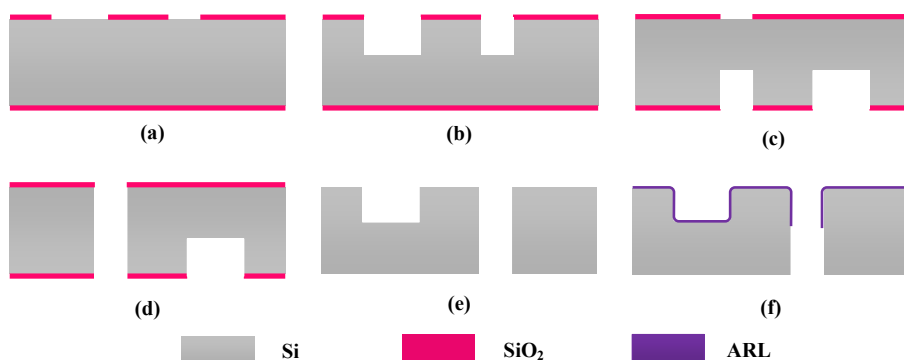
Figure 4.9: Fabrication process flow of top silicon submounts: (a) front side mask layer patterning (b) front side DRIE (c) back side mask layer patterning (d) back side DRIE (e) mask layer removal (f) ARL coating.
