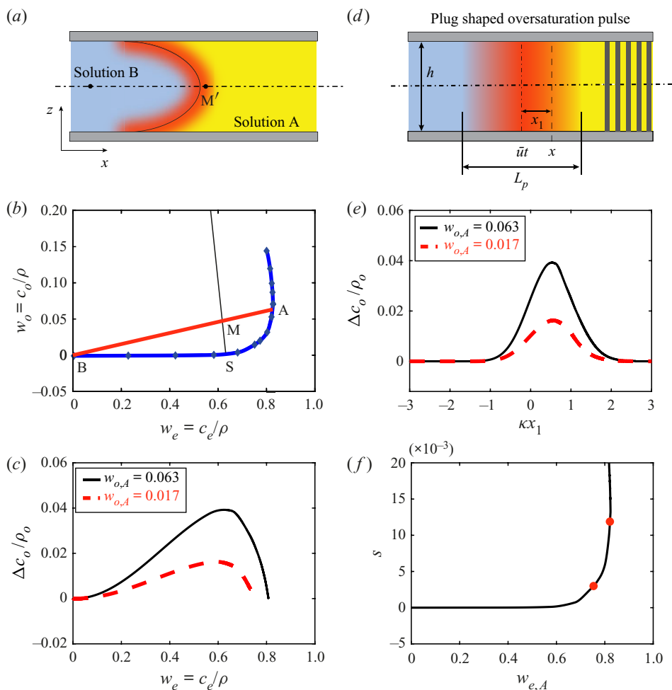
Figure 3. (a) Sketch of the oversaturation pulse (red region) during solvent exchange. Solution A is on the right-hand side, being displaced by solution B. Liquid parcel M' is on the oversaturation pulse. The concentrations of solutions A, B and liquid parcel M' are represented by A, B and M in (b), respectively. (b) Phase diagram of the decane-ethanol-water ternary system. The blue curve is the binodal curve (saturation curve of oil) fitted from the data points (blue diamond) measured as described in Tan et al. (2016). Red line AB is the diffusion path, black line MS is the dilution curve, which is a straight line passing through coordinate (0, 1). (c) Oil oversaturation normalized by the oil density, \Delta c_o/\rho_o , as a function of the normalized ethanol concentration w_e = c_e/\rho , at different initial conditions: black solid line for w_{o,A} = 0.063 , and red dashed line for w_{o,A} = 0.017 . (d) Plug shaped oversaturation pulse because of Taylor-Aris dispersion which happens in a long and thin channel; x_1 = x - \bar{u}t is the distance to the centre of the plug, \bar{u} is the average flow velocity and L_p is the length of the plug. The porous region is represented by the vertical black pillars. (e) The normalized oil oversaturation \Delta c_o/\rho_o as a function of normalized length \kappa x_1 , for w_{o,A} = 0.063 (black solid line), and w_{o,A} = 0.017 (red dashed line), respectively. The normalized length \kappa x_1 is a function of time t and space x . (f) The calculated prefactor s as a function of w_{e,A} . The two different initial conditions with w_{o,A} = 0.063 and 0.017 are indicated by the red dots.
