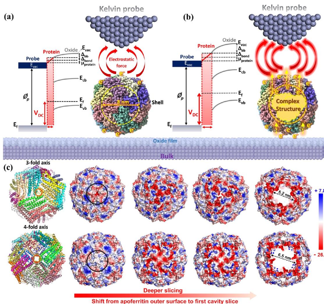
Figure 2. Schematic demonstration of the SKPFM principle along with the energy level diagram during the electrostatic interaction between a highly conductive AFM tip apex and (a) single fresh or (b) filled-apoferritin molecules on the oxide-bulk matrix at the atomic scale. The formation of a complex cluster in the internal cavity of the apoferritin molecule can significantly alter the energy level diagram, electrical surface potential, and intensity of electrostatic forces, and (c) the 3-fold and 4-fold axes of apoferritin molecules and their corresponding surface electrostatic potential in the different slices from the outset surface to closet or last slice to cavity (data generated by PyMoL and ChimeraX (PDB ID: 2W0O)) where positive, neutral, and negative amino acid residues are presented in blue, white, and red, respectively.
