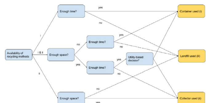
Fig. 3. Representation of Agents decision tree.
