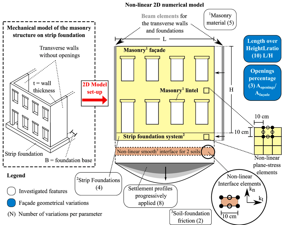
Fig. 2. Illustration of the intended mechanical model and the adopted FE modelling approach, the features included and the variations investigated. Number of variations per parameter indicated in parenthesis (N). The foundation systems adopted in the model are shown in detail in Fig. 4, while the settlement profiles applied at the bottom edge of the interface are shown in Fig. 5.
