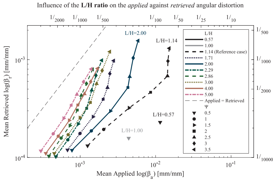
Fig. 9. Influence of the length over height ( L/H ) ratio on the difference between applied vs. retrieved angular distortion. The secondary x- and y- axes (on top and on the right of the plots) show the values of the angular distortion as 1/\beta^{-1} , as typically adopted in the literature. Plot in the logarithmic scale.
