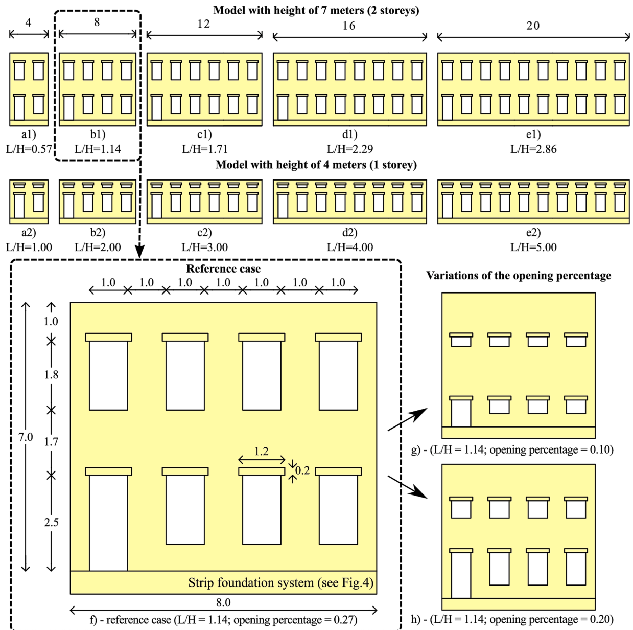
Fig. 3. Reference geometries for the masonry façade. The geometries from a1) to e2) are characterized by an opening ratio ( A_{\text{opening}}/A_{\text{façade}} ) of 0.27. The model f) represents the reference case. The height of the openings of f) is modified arbitrarily for the geometries g) and h) to obtain the two selected opening percentages (i.e. 0.10 and 0.20 respectively). The foundation systems adopted in the model are shown in detail in Fig. 4. Not to scale. Measures in meters.
