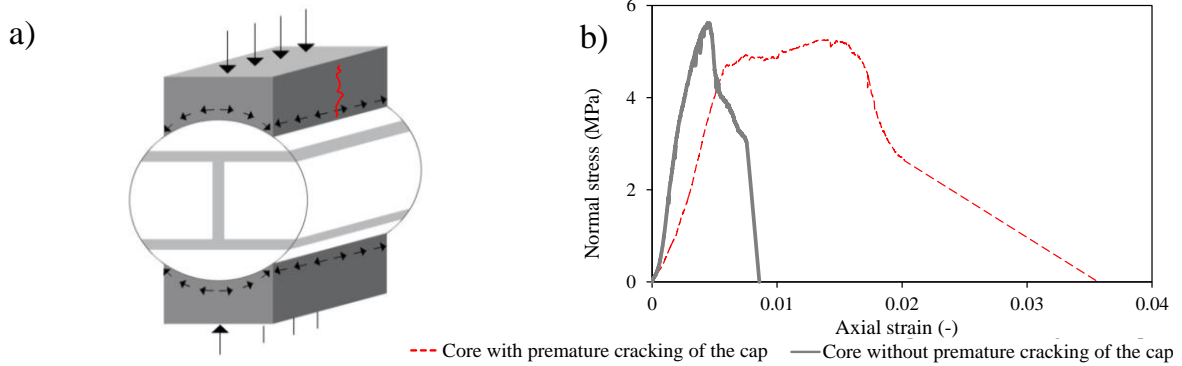
Fig. 6. (a) Premature cracking of the capping mortar; (b) difference between compression response of masonry cores with and without premature cracking in the cap.
