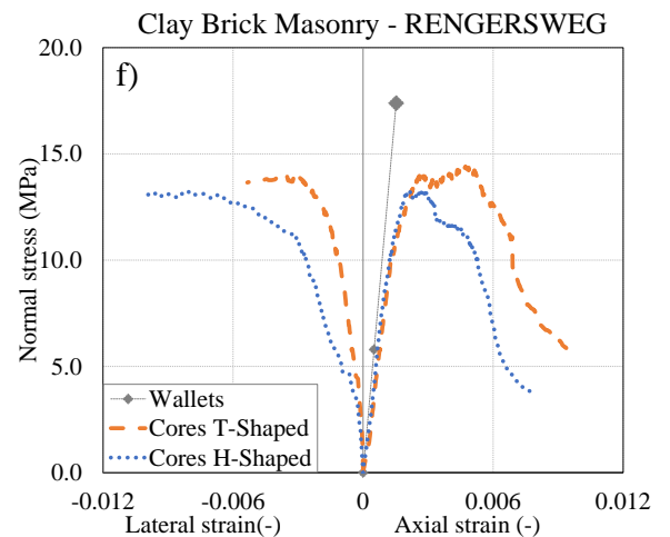
Fig. 13. Existing clay masonry (Rengersweg): (a) no information about crack pattern of wallets was available; (b)-(c) final crack pattern of T-shaped core; (d)-(e) final crack pattern of H-shaped core; (f) mean stress-strain relationships [45].
