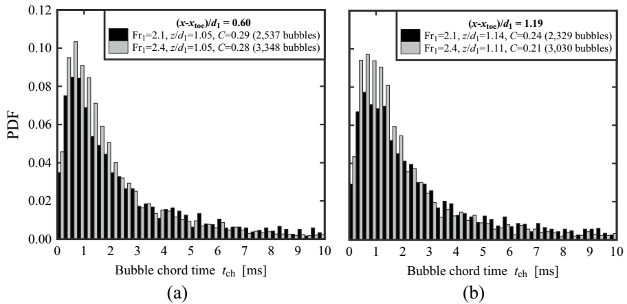
Fig. 13 PDF of the bubble chord time at the elevation where F = F_{\max} for both Fr_1 = 2.1 and 2.4 at two selected locations behind the jump toe (x-x_{\text{toe}})/d_1 = 0.60 and 1.19 . Channel centreline data
