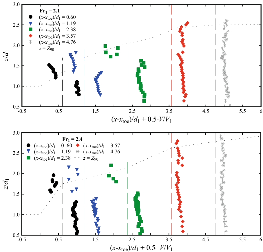
Fig. 15 Air–water interfacial velocities at different locations from the roller toe for: (top) Fr_1 = 2.1 , d_1 = 0.097 , V_1 = 2.10 m/s; (bottom) Fr_1 = 2.4 , d_1 = 0.084 , V_1 = 2.21 m/s. Dashed vertical lines represent reference lines for V/V_1 = 0 at each (x-x_{10e})/d_1 position. Channel centreline data
