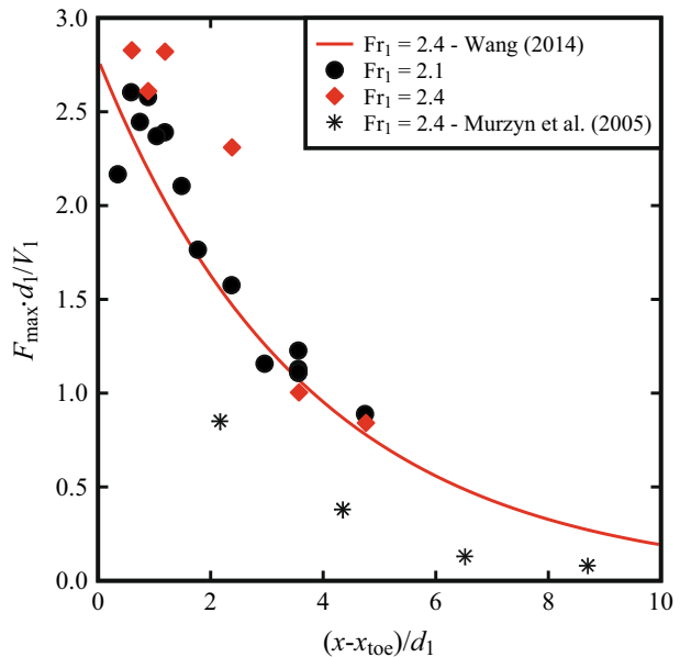
Fig. 12 Maximum bubble count rate F_{\max} as a function of the longitudinal distance from the roller toe for Fr_1 = 2.1 , Fr_1 = 2.4 and comparison with Murzyn et al. [26] for Fr_1 = 2.4 and Re = 7.54 \times 10^4 . Channel centre-line data
