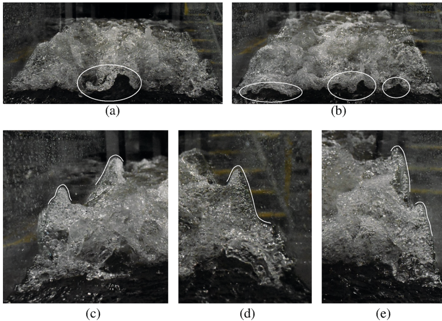
Fig. 6 Photographs of caves ( a , b ) and vertical structures along the sidewall ( c , d and e ) for a hydraulic jump with Fr_1 = 2.1 ( d_1 = 0.097 m, V_1 = 2.1 m/s, Re = 2.03 \times 10^5 ). Initial flow from foreground to background. Shutter speed 1/800 s
