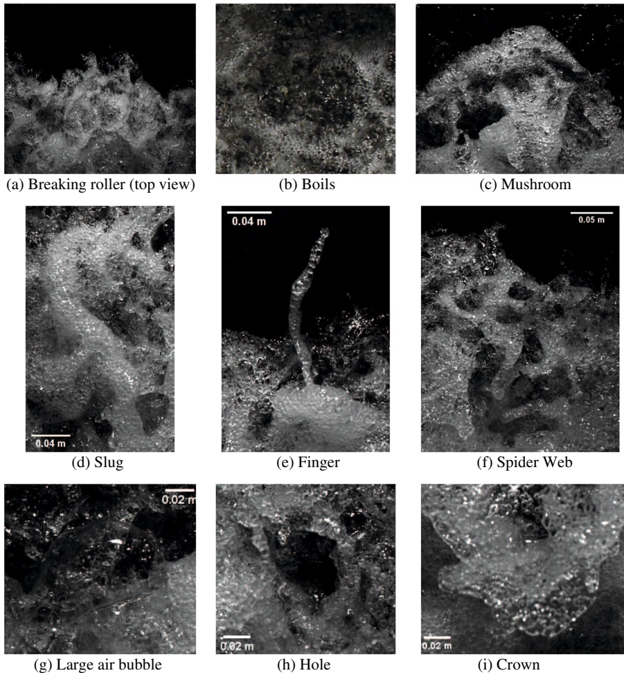
Fig. 5 Top view of the strong free surface turbulence observed in a breaking roller with Reynolds number Re = 1.86 \times 10^5 and Froude number Fr_1 = 2.4 : a Top view of the roller; b Boil; c Mushroom; d Slug; e Finger; f Spider web; g Large air bubble; h Hole; i Crown. Initial flow direction from top to bottom
