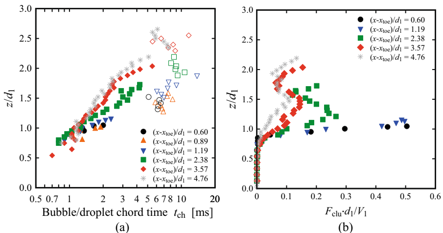
Fig. 14 Fr_1 = 2.1 ( d_1 = 0.097 m, V_1 = 2.10 m/s): a Vertical distributions of the median particle chord time t_{\text{ch}} : full symbols represent bubble chord times ( C < 0.3 ), while empty symbols represent water droplets chord times ( C > 0.7 ); b Cluster count rate F_{\text{clu}} for C < 0.3 at different locations behind the roller toe. Channel centreline data
