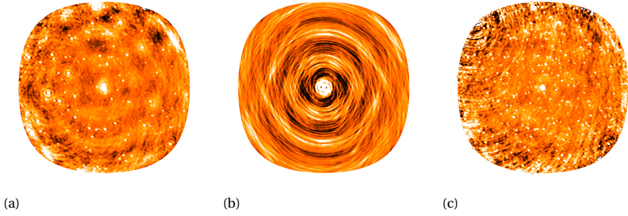
Figure 5.12: Three CLEAN related images. Left an input dirty image, in the middle a point-spread function representing the telescope response function, and on the right the dirty image deconvolved with the point-spread function.
