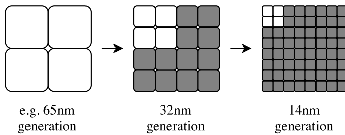
Figure 1.5: Effect of the ‘power wall’: for every process generation, we have to switch-off a larger fraction of the transistors to stay within the power budget, even at constant frequencies. This is popularized as ‘dark silicon’ [16]. (image based on: [18])
