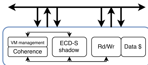
Figure 4.5: The main components in the near-data processor access point (NDP-AP). The fat arrows indicate data ramps.
