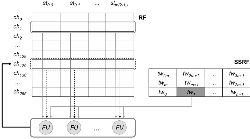
Figure 3.4: Proposed input data organization for the FIR and the FFT algorithm. The picture also sketches how data are processed by the proposed micro-architecture when implementing the FFT.
