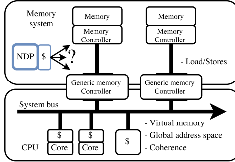
Figure 4.2: The problem of integrating NDPs with a CPU: all relevant integration features stop at the memory controllers.
