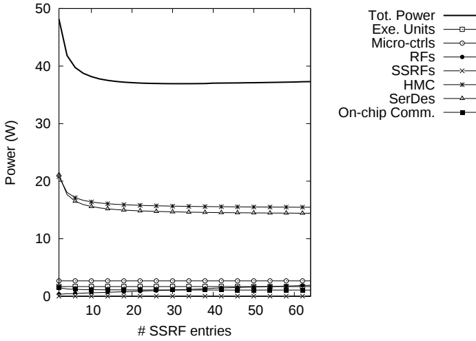
Figure 3.9: Power consumption while varying the size of the SSRF (8 FUs per core).
