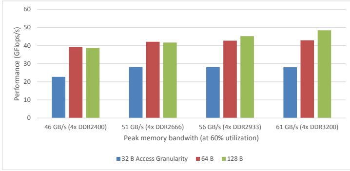
Figure 6.5: Impact of the access granularity and peak bandwidth for the HPCG benchmark.
