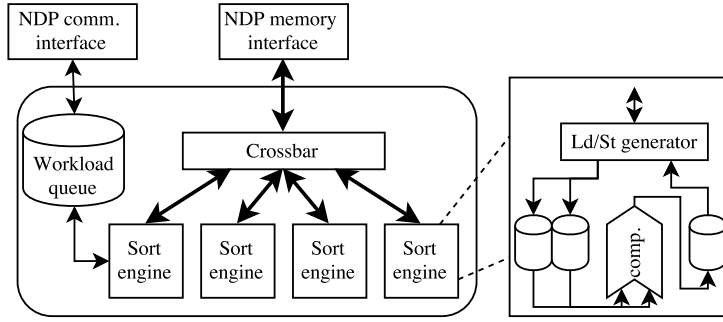
Figure 7.5: Block diagram of the workload-optimized merge core implemented in the NDP.
