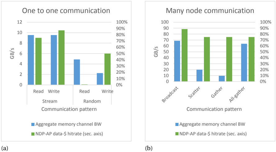
Figure 4.9: Synthetic benchmark results, showing bandwidths and NDP-AP data cache hit rates for various inter-NDP communication patterns.
