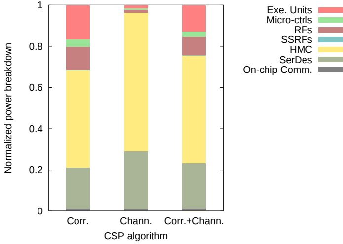
Figure 3.10: Power breakdown for correlation and channelization.
