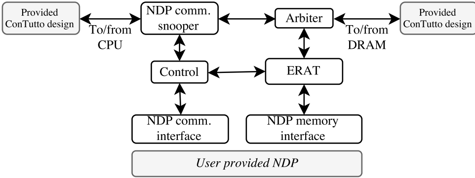
Figure 5.2: The main components of the NDP-M, implemented in VHDL. IO is defined by the provided ConTutto interfaces based on Altera Avalon.
