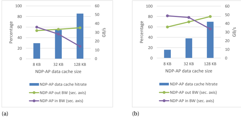
Figure 6.10: Impact of the NDP-AP data cache size on the NDP-AP data cache hit rate and NDP-AP incoming and outgoing bandwidths.
