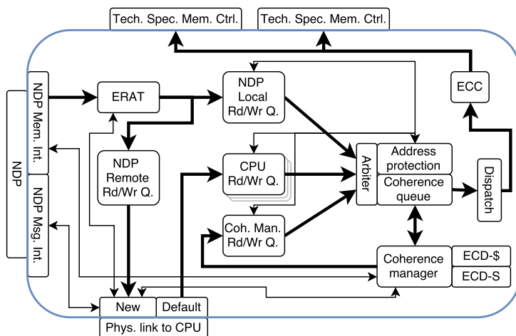
Figure 4.4: Main functional blocks within the near-data processor manager (NDP-M). In reality, the CPU Rd/Wr queue can consist of several queues, for example a separate one for prefetch loads. For simplicity, only the forward path towards the DRAM is shown.
