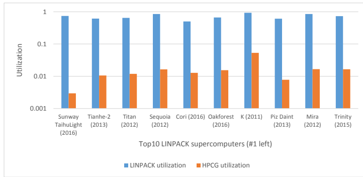
Figure 1.8: The utilization for the top 10 supercomputers, running the LINPACK and the HPCG benchmark.
