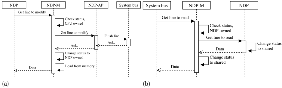
Figure 4.6: Two activity diagrams showing possible coherence interactions between the NDP and the CPU. In (a) the NDP wants to write to a line currently owned by the CPU, and in (b), the CPU wants to read a line currently owned by the NDP.
