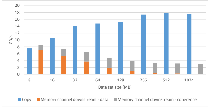
Figure 4.10: Using an NDP to copy a data set, of which 8 MB is stored in the caches of the CPU. The initial coherence state is CPU owned .
