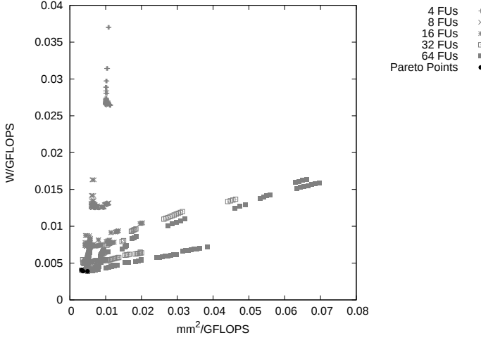
Figure 3.7: Results of the parameters design-space exploration for the proposed architecture.
