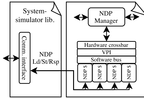
Figure 5.9: Complementary to Figure 5.8, showing the ability to run arbitrary software on general-purpose NDP cores, while still using the hardware NDP-M.
