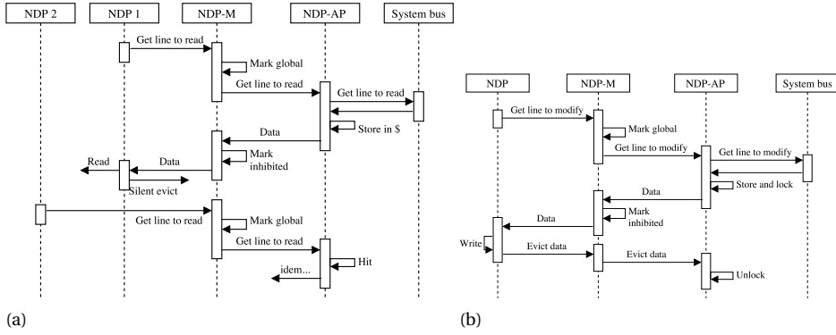
Figure 4.7: Two activity diagrams showing the process of a remote read (a) and a remote write (b).
