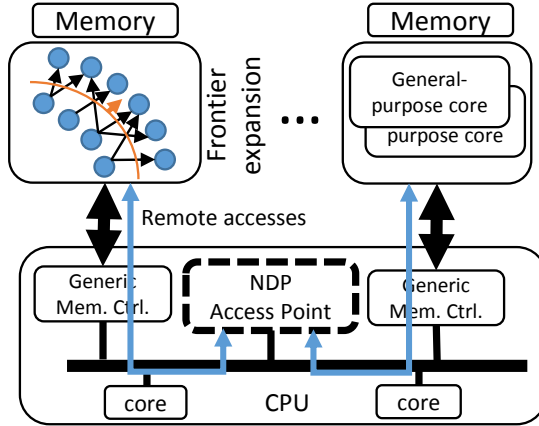
Figure 4.12: Graph500 mapped on our architecture. The frontier expansion is done at the NDPs, with non-local accesses being forwarded to the NDP-AP.
