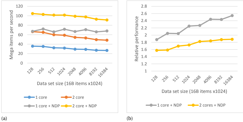
Figure 7.6: (a) Absolute mergesort performance for four different systems configurations. (b) Relative performance with respect to configuration with no NDPs.
