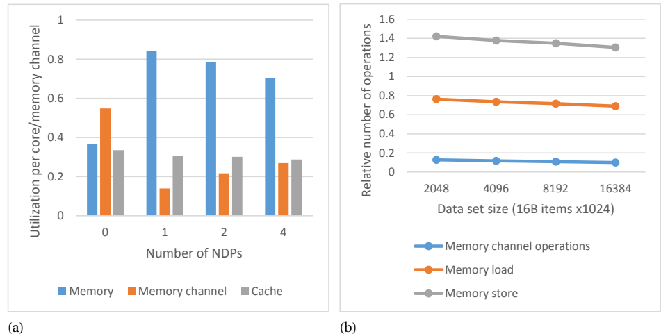
Figure 7.8: (a) The component utilization for various number of memory channels / NDPs, when sorting 16 mega items. (b) Relative number of operations generated by the single CPU core and single NDP configuration, with respect to a single CPU configuration.
