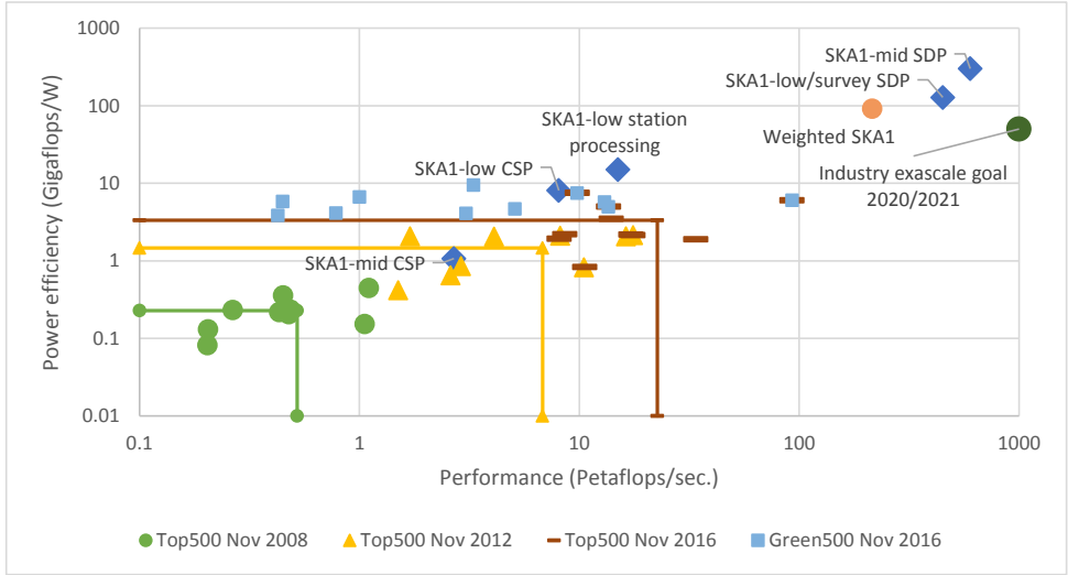
Figure 2.6: The compute and power efficiency points for the SKA subsystems, put next to TOP500 trends.
