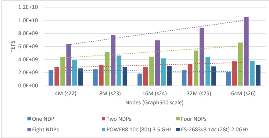
Figure 4.13: Performance for Graph500 running at our NDP architecture, with an IBM POWER8 and Intel Xeon CPU serving as reference.
