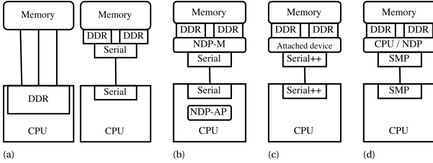
Figure 8.1: Evolution of memory attachment technologies. (a) Shows both traditional direct-attached DDR memory, as well as serial attached DDR as found in the POWER7 and POWER8 CPUs. (b) Shows the NDP-integration strategy proposed in this work, using the existing load/store serial interface. (c) Shows future serial-link protocols enabling the attachment of devices without the need of extra components [45]. (d) Shows the far end of the spectrum, attaching devices / NDPs over an SMP link, and making them equal to the CPU.
