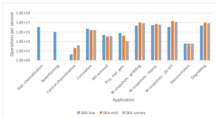
Figure 2.3: Compute requirement estimates for the various applications for the three SKA instruments.
