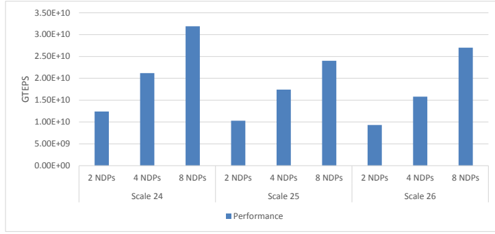
Figure 6.11: Performance for the Graph500 benchmark, varying the problem size as well as the amount of NDPs.
