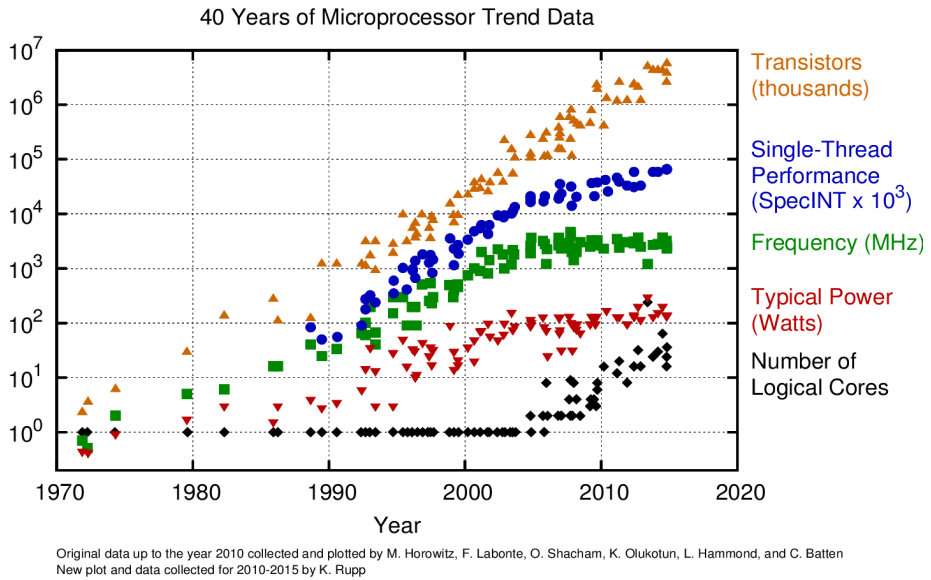
Figure 1.4: The effects of the ‘power wall’: processors have hit the limit of power usage, and the frequency cannot increase further because of that. (Image source: [17])
