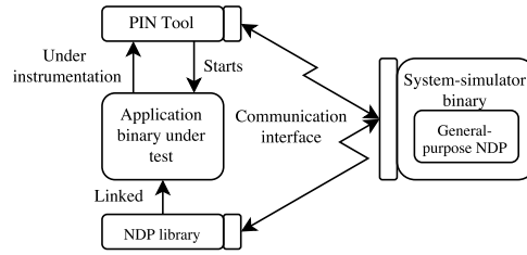
Figure 5.11: High level overview of the performance-simulator, with an Intel PIN front-end.
