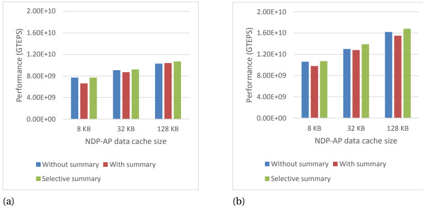
Figure 6.9: Impact of the NDP-AP data cache size on Graph500 performance, including the (selective) use of bitmap summaries.
