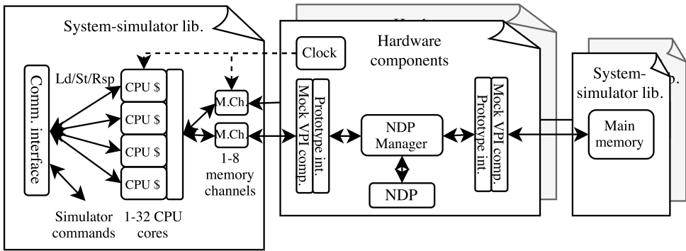
Figure 5.8: Overview of the system-simulator. Clearly identifiable are the parts implemented in hardware, and how they are connected to the parts implemented in software.
