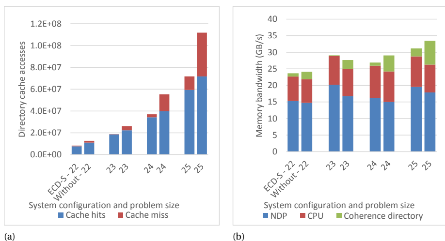
Figure 4.15: Performance of the coherence architecture as described in Section 4.5.3, with and without the use of the proposed ECD-S described in Section 4.5.3.
