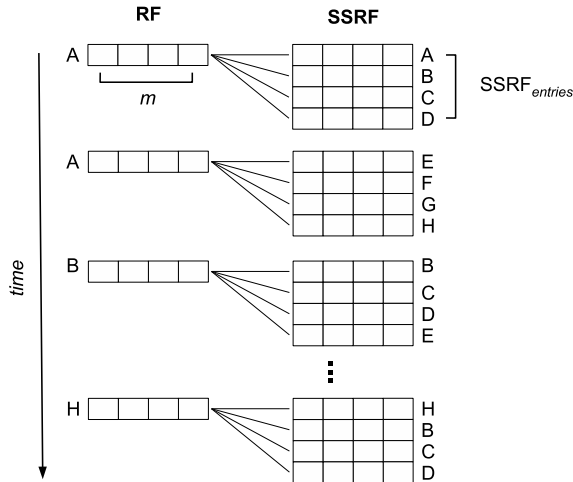
Figure 3.6: Overview of an optimized input data scheduling on the proposed architecture for the correlation algorithm.
