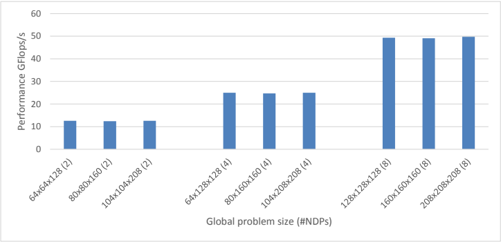
Figure 6.7: Performance scaling for the HPCG benchmark, using various problems sizes and number of NDPs.
