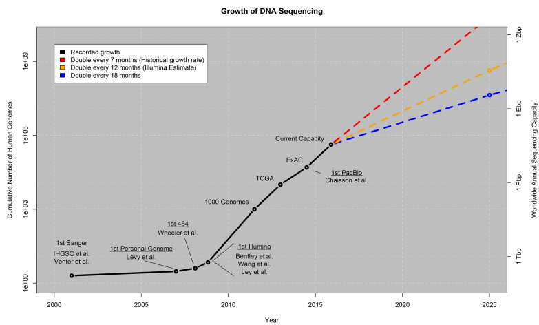
Figure 1.3: Illustrating the amount of available genomic data, growing much faster than Moore's law (source: [8]).
