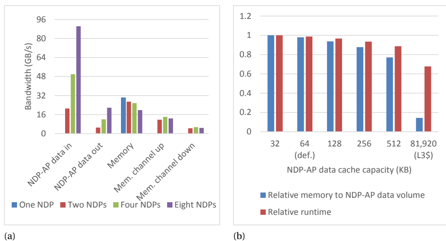
Figure 4.14: (a) Various system bandwidths when running a scale 24 problem. (b) The impact of the NDP-AP data cache size on hitrate and performance running a scale 24 problem, using four NDPs.
