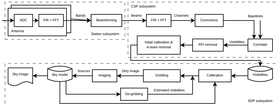
Figure 2.2: Overview of the processing steps for the SKA-low, using imaging pipeline. For SKA-mid and SKA-survey, the antenna/station subsystem will be replaced by a dish.
