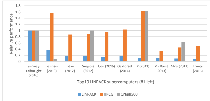
Figure 6.2: The relative performance of the top 10 (out of the TOP500) supercomputers, running the LINPACK, HPCG, and Graph500 benchmark. [3] [57]
