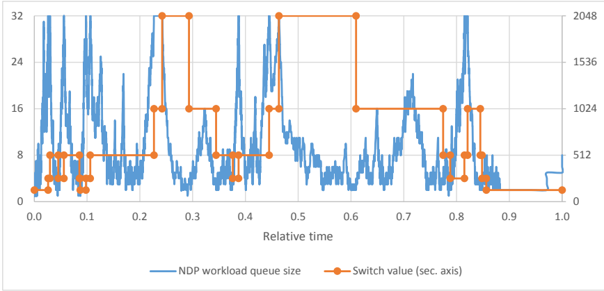
Figure 7.9: NDP work queue size and switch value over time, when sorting four mega items using two CPU cores and a single NDP.
