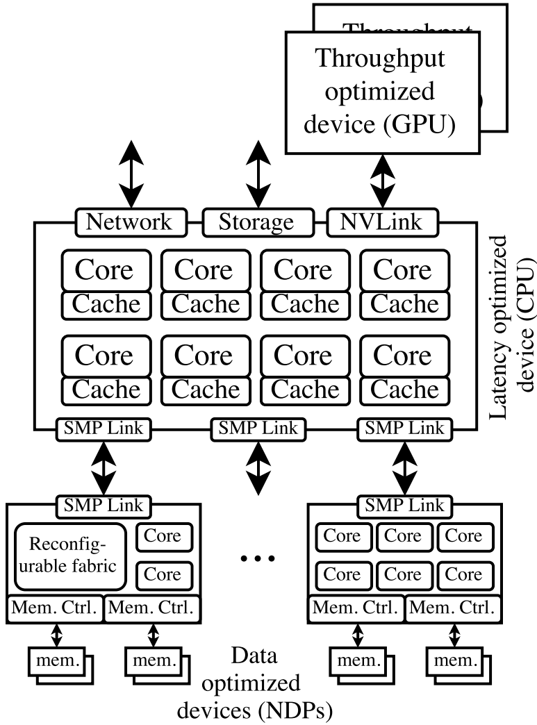
Figure 8.2: Placing NDPs as full CPU-peers in a system.
