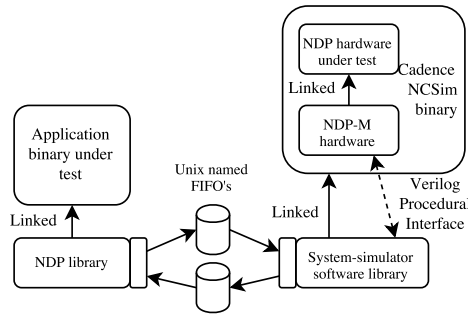
Figure 5.7: Overview figure of how the various applications, libraries and hardware components interact with each other.
