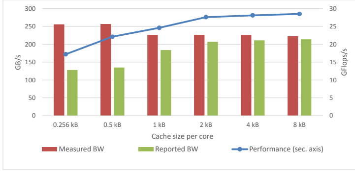
Figure 6.4: Impact of the NDP core cache size. HPCG is able to achieve peak floating-point performance with a 4 KB cache per core.
