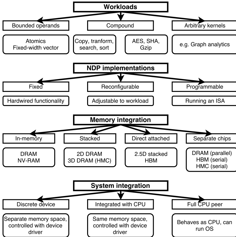
Figure 1.14: Taxonomy of near-data processing in and near main-memory.
