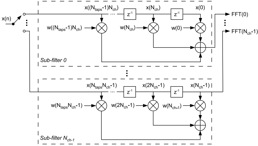
Figure 3.2: Block diagram of the CSP poly-phase filter.
