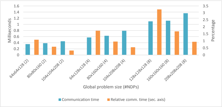
Figure 6.8: Absolute and relative communication time for the HPCG benchmark, using various problems sizes and number of NDPs.
