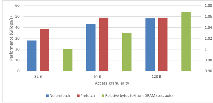
Figure 6.6: Impact of software prefetching for the HPCG benchmark, while also varying the access granularity.
