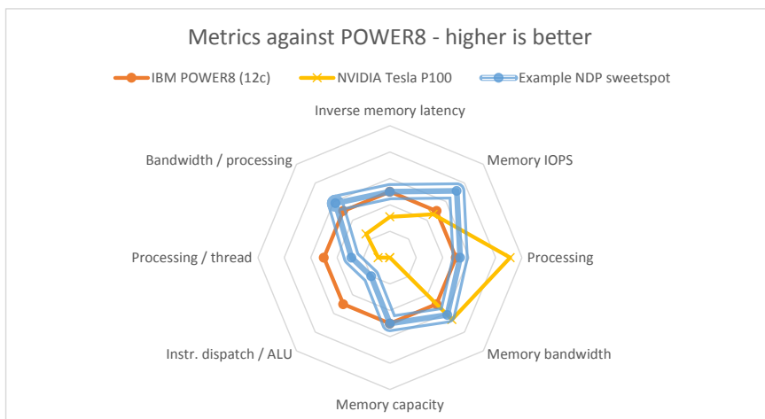
Figure 8.3: Positioning NDPs between a CPU and a GPU, creating a device optimized for data intensive applications. The chart uses a logarithmic scale.
