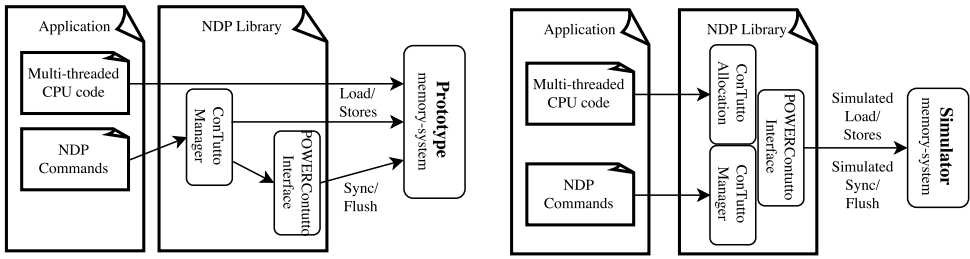
Figure 5.6: Two figures showing how loads, stores, and special commands enter either a real memory system (on the left), or a simulated memory system (on the right).
