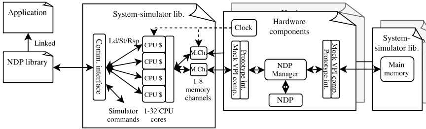
Figure 7.3: The simulator environment used in our experiments.
