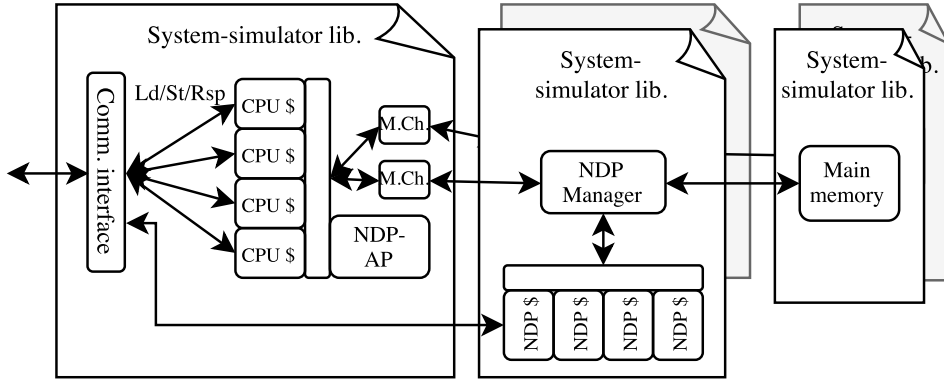
Figure 5.10: Overview of the performance-simulator. The NDP-M and NDP-AP are implemented in software supporting complex system-level interactions. The NDPs are general-purpose cores.
