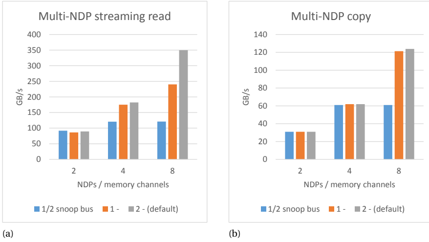
Figure 4.11: (a) Accumulated streaming read performance using multiple NDPs, while varying the amount of snoop buses at the CPUs' system bus. (b) Accumulated copy performance using multiple NDPs, while varying the amount of snoop buses at the CPUs' system bus.
