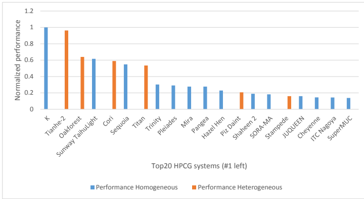
Figure 1.11: The relative performance of the top 20 system running the HPCG benchmark, indicating which ones are homogeneous, and which ones are heterogeneous.
