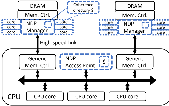
Figure 6.3: The studied system, with processing capabilities included close to the main-memory of a CPU.
