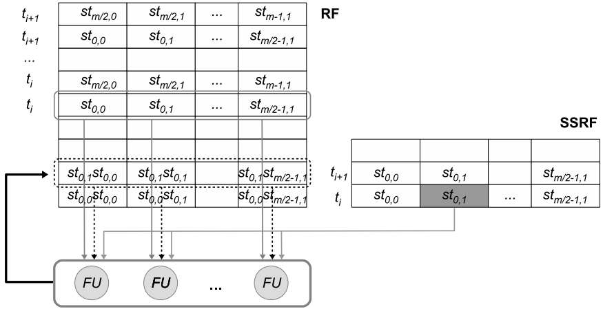
Figure 3.5: Proposed input data organization for the correlation. The picture also sketches how data are processed by the proposed micro-architecture when implementing the correlation (one channel).
