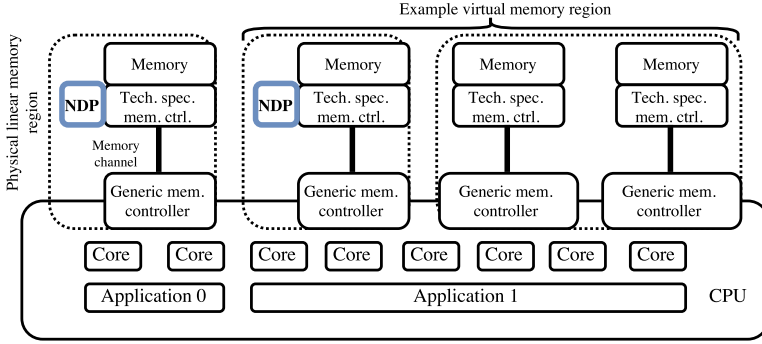
Figure 4.1: The high level view of the proposed architecture, where compute capabilities are added close to the main memory of a CPU.
