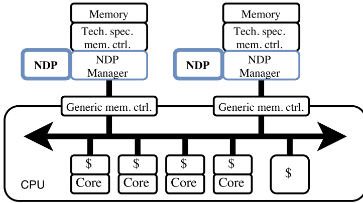
Figure 7.2: High-level view of the system organization. Near-data processors are tightly integrated with the memory controllers.
