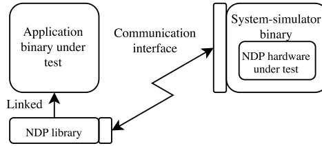
Figure 5.5: High level view of the system-simulator, showing both the application under test, the simulator, and the communication channel.
