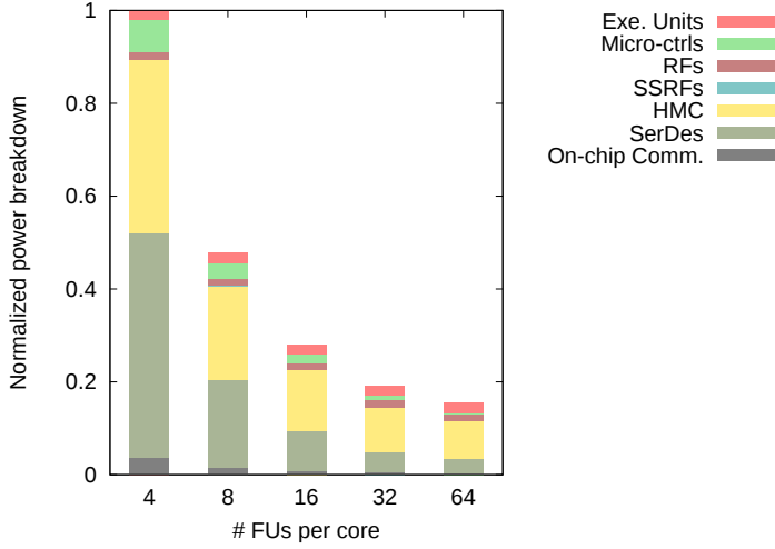
Figure 3.8: Power breakdown for different core configurations.
