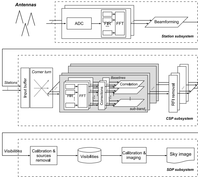
Figure 3.1: Overview of the processing steps for the SKA1-Low, using the continuum imaging science case [142].
