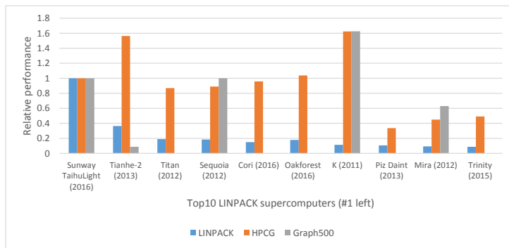
Figure 1.9: The relative performance of the top 10 supercomputers running the LINPACK, HPCG, and the Graph500 benchmark.
