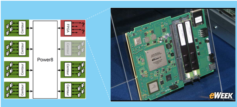
Figure 5.1: An illustration of the ‘ConTutto’ prototype platform. One of the Centaur ASICs in a POWER8 is replaced by an FPGA.
