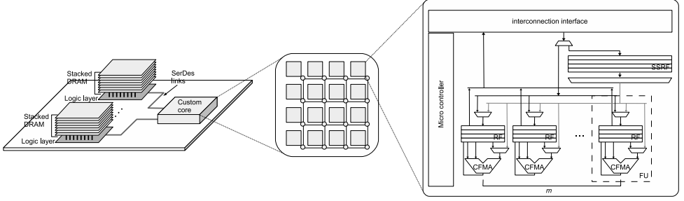
Figure 3.3: Overview of the proposed accelerator architecture. From left to right: socket, chip, core.
