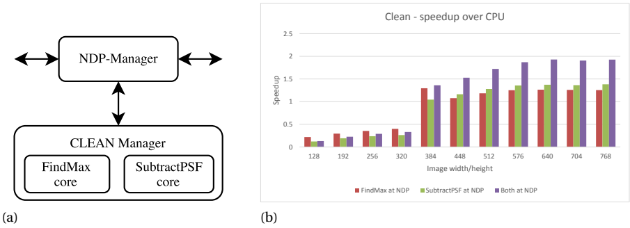
Figure 5.13: NDP hardware design for CLEAN implemented in VHDL, showing the two type of coprocessors for the two offloaded methods. (b) Results for clean, showing speedups when running one of the two, or both, methods on the NDP. Horizontal axis shows the image-size along a single side.
