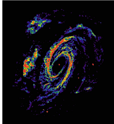
Figure 2.1: Cold atomic hydrogen gas in the M81 galaxy, measured at 1420.4 MHz. As a reference, human-visible red light has a frequency of 430 THz. Image courtesy of NRAO, D. S. Adler, D. J. Westpfahl.
