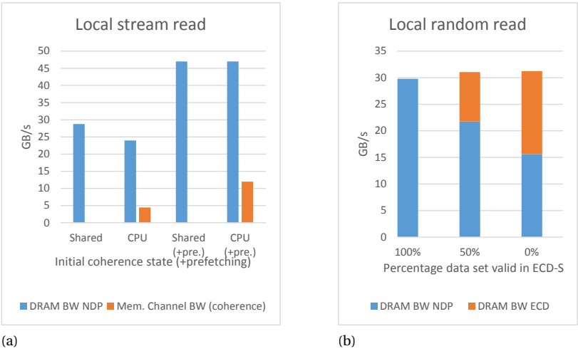
Figure 4.8: (a) Shows achieved DRAM bandwidth and memory channel bandwidth (coherence messages) for local streaming reads, while varying the initial coherence state, with and without software prefetching. (b) Shows achieved DRAM bandwidth for local random reads, while varying the percentage of data valid in the ECD-S.
