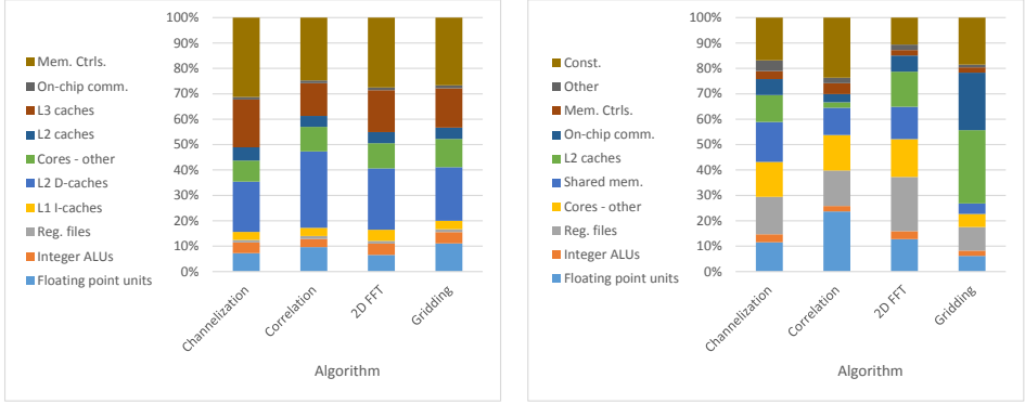
Figure 2.5: Power breakdown on CPUs (left) and GPUs (right) for the four SKA algorithms considered in this work: channelization (Chann.), correlator (Corr.), 2D FFT and Gridding (Grid.).
