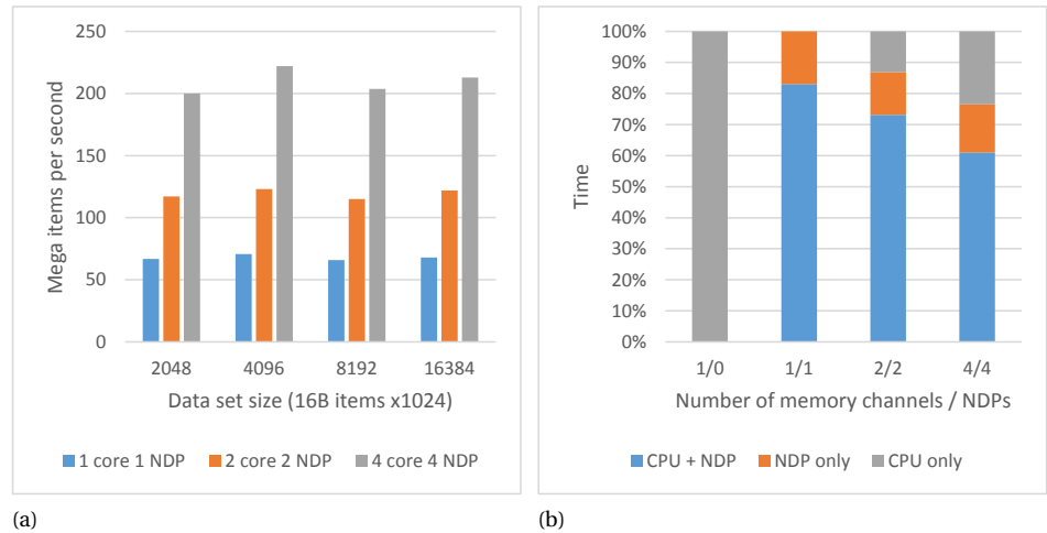
Figure 7.7: (a) Performance for systems containing more memory channels and NDPs. (b) Time distribution of the heterogeneous usage of both the CPU and the NDP.
