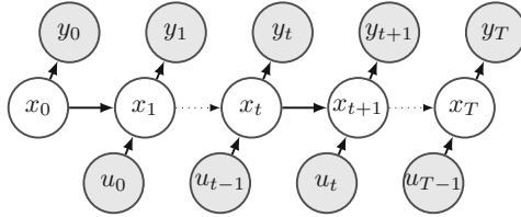
Fig. 1. Probabilistic graph model of a Hidden Markov Chain.
