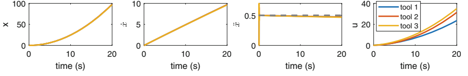
Fig. 4. Meta-TAIC takes the SMD to a constant goal acceleration (task 3) using all tools. The graphs are coinciding for all tools. All tools reach the goal acceleration (marked by dotted black in Fig. 4c).
