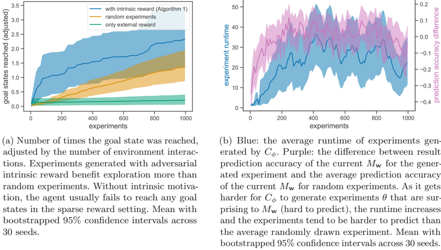
Fig. 3. Experiments in the differentiable force field environment
