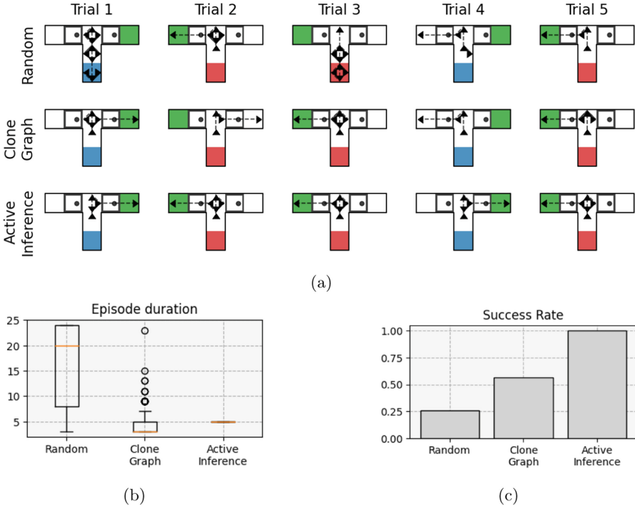
Fig. 4. (a) Qualitative results of navigating the T-maze with the three different agents. The green square marks the goal observation, and the black arrows the trajectory followed by the agent. At the bottom of the T, there is a colored cue, blue marks that the goal is on the right, while red marks that the goal is on the left. (b) Shows the number of steps needed for reaching the target, only measured for the success cases. (c) Shows the success rate, computed over 400 trials for the three agents. (Color figure online)
