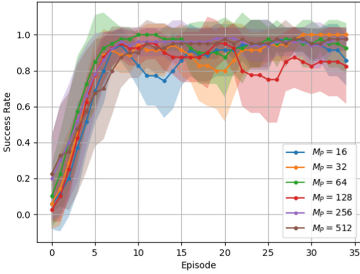
Fig. 4. Impact on the success rate when changing the number of neurons M_P in the state transition network .
