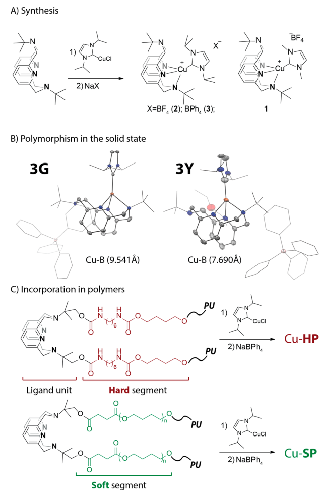
Figure 1. Structures and synthesis of new compounds used in this work (A). Selected solid-state structures of polymorphs of complex 3 and Cu–B distances (B) and selective polymer phase labeling pathway (C). For structural data for compounds 2 and 3, see Supporting Information.
