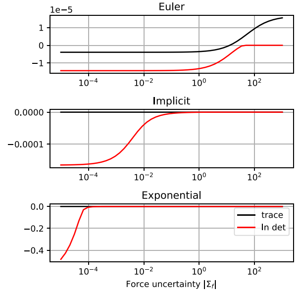
Fig. 4. Minimum eigenvalue of the Hessian \nabla^2 \text{Tr} \Sigma^+ and \nabla^2 \ln \det \Sigma^+ with respect to impedance parameters as \Sigma_f varies, where the minimum eigenvalue must be positive for this objective to be convex. The integrator schemes (Euler/implicit/exponential) and objective (Tr vs ln det) affect the convexity, where the implicit and exponential integrator with trace performs best over a range of force uncertainty.
