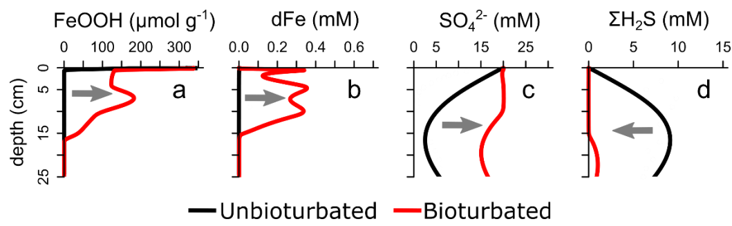
Figure 7: Model results of two identical sediments, one without bioturbation (black line) and one with bioturbation (red line). Model set-up is described in Appendix 1, model scenario shown here is ‘B + SP’ and an irrigation rate of 1.2 yr -1 . (a) iron oxide (FeOOH), (b) dissolved iron (dFe), (c) sulphate (SO 4 2- ), (d) free sulphide (HS - ). Grey arrow indicates the effect of bioturbation; the sediment becomes higher in iron content due to the stimulation of iron cycling, which limits the build-up of free sulphide.
