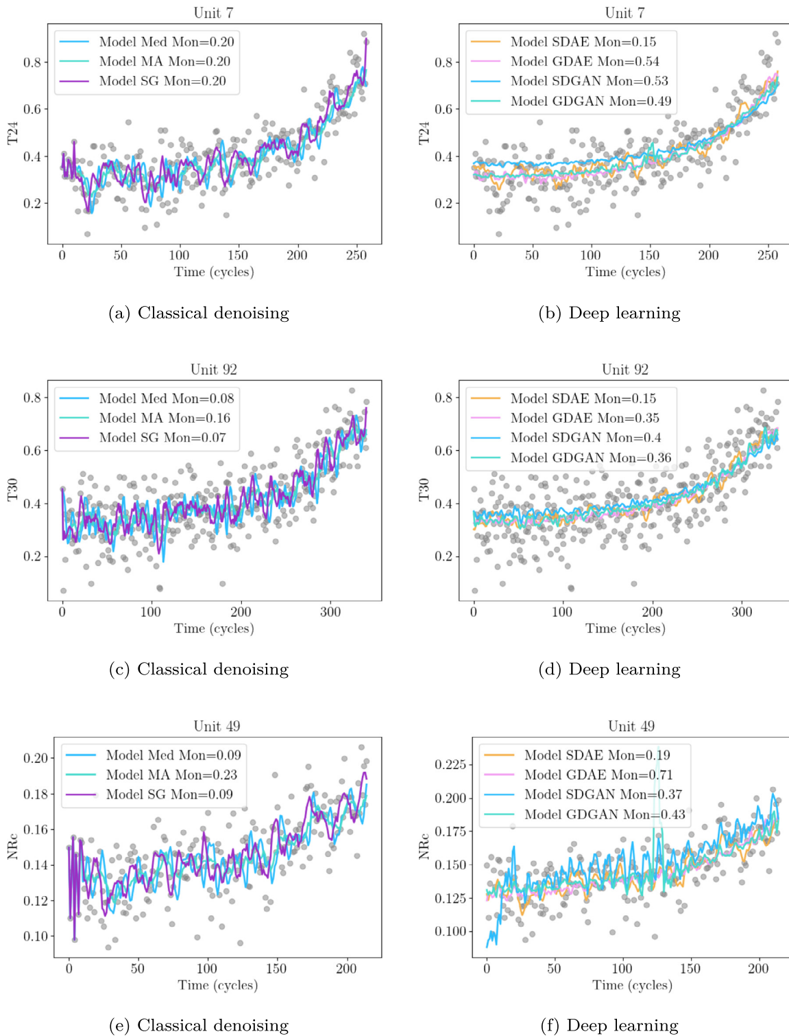
Fig. 9. Visualization of denoising methods for randomly selected engines. On the left side, we show the classical techniques from statistics, and on the right side, the deep learning approaches. The deep learning approaches perform better than the classical denoising methods.
