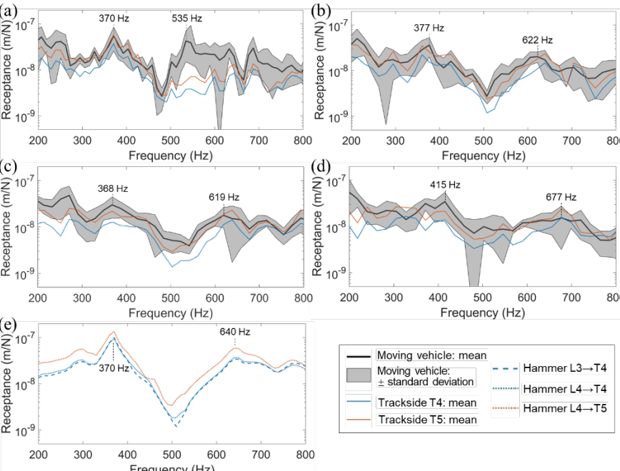
Figure 5.15: TF estimation and comparison on Track section ⑤ (Vehicle B). (a) 8 km/h; (b) 10 km/h; (c) 14 km/h; (d) 16 km/h; (e) Hammer tests.
