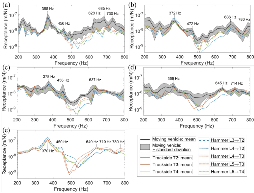
Figure 5.14: TF estimation and comparison on Track section ④ (Vehicle A). (a) 8 km/h; (b) 10 km/h; (c) 14 km/h; (d) 16 km/h; (e) Hammer tests.
