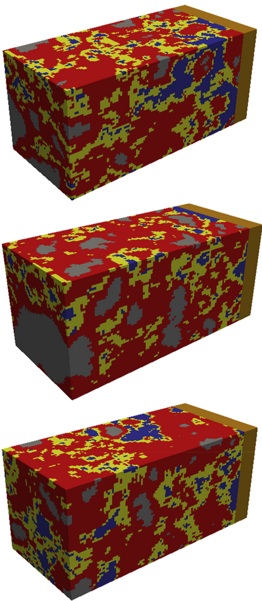
Fig. 9. Type I specimens with size of 220 μm × 100 μm × 100 μm (110 voxel × 50 voxel × 50 voxel, three specimens are shown for clarity).
