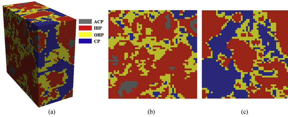
Fig. 11. Type II specimen with size of 50 \mu\text{m} \times 100 \mu\text{m} \times 100 \mu\text{m} (25 voxel \times 50 voxel \times 50 voxel): (a) side view; (b) view from the bulk cement paste side; (c) view from the aggregate side.
