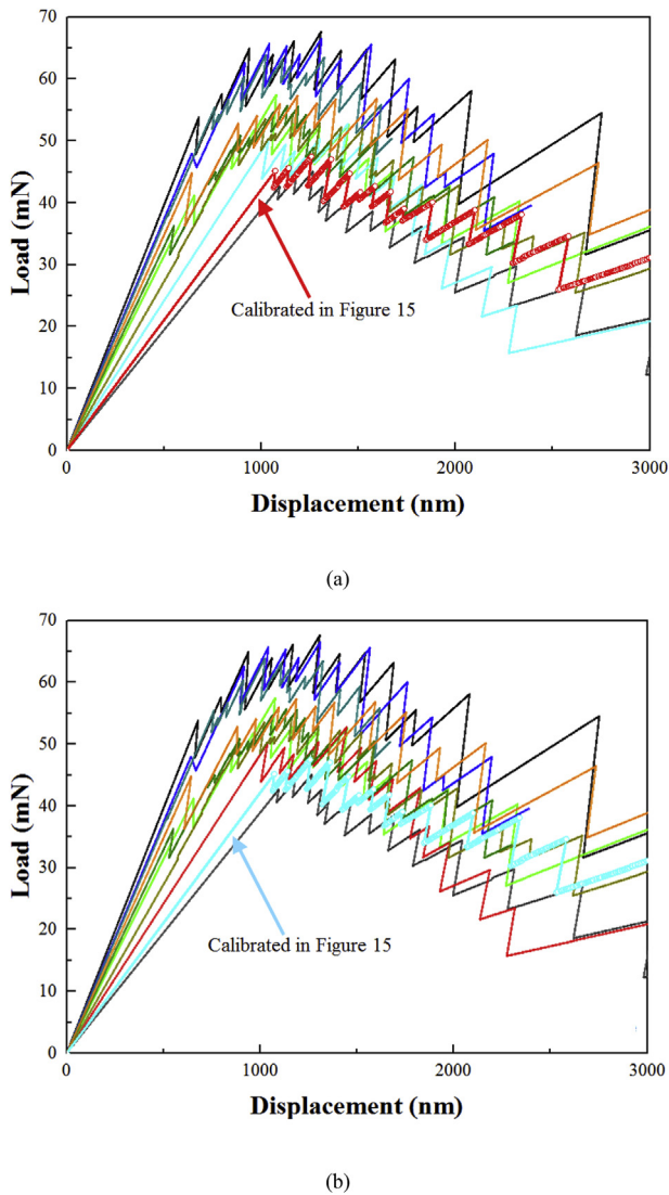
Fig. 15. Modelling results of 10 ITZ cantilever specimens under: (a) fully contacted boundary conditions (b) edge contacted boundary conditions.
