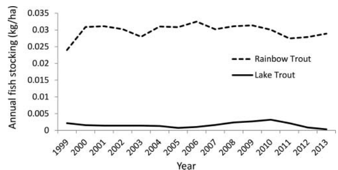
FIGURE A.3.2. Annual fish stocking biomass for Rainbow Trout and Lake Trout. The values are based on those in the 2014 annual report by the Lake Erie Cold Water Task Group ( http://www.glfc.org/lakecom/lec/CWTG_docs/annual_reports/CWTG_report_2014.pdf [March 2015]).
