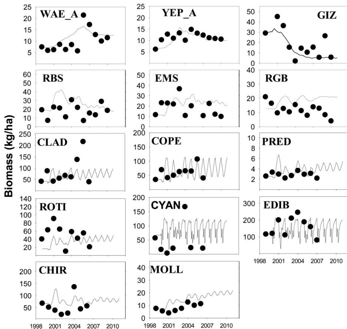
FIGURE 2. Model calibration of selected species/groups in the Lake Erie EwE model. The lines represent model-simulated biomass values, and the circles represent empirical observations from resource agency monitoring surveys. There were 12 years of observed biomass data for fish species (1999–2010), 9 years for plankton groups (1999–2007), and 8 years for benthic groups (1999–2006). See Table 1 for full species/group names.
