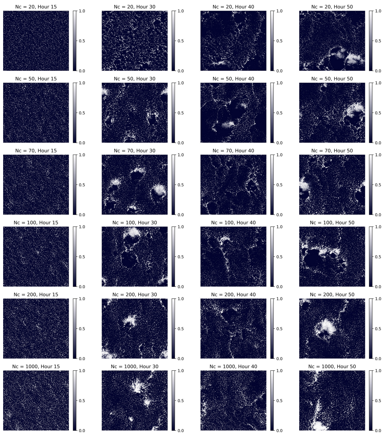
Figure 3. Cloud-field albedo examples. The panels show how cloud fields develop in our LESs featuring the diurnal cycle of insolation with N_c of 20 (first row), 50 (second row), 70 (third row), 100 (fourth row), 200 (fifth row), and 1000 \text{cm}^{-3} (sixth row), at hours 15 (first column), 30 (second column), 40 (third column), and 50 (fourth column) after the start of simulations.
