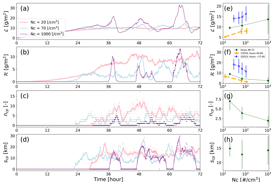
Figure 4. Time series of clouds, rain, and spatial properties of cold pools in simulations without a diurnal cycle. Panels (a)–(d) show time series of \mathcal{L} , \mathcal{R} , n_{cp} , and s_{cp} for simulations without the diurnal cycle of solar incoming radiation, where solid lines shown for cold-pool number and size provide a guide to the eye obtained through Gaussian filtering of the original data points. Note that there is significant precipitation in the N_c = 20 \text{ cm}^{-3} case before cold pools with diameters larger than the 5 km threshold appear. Panels (e)–(h) show the response of \mathcal{L} , \mathcal{R} , n_{cp} , and s_{cp} to N_c . The results from Yamaguchi et al. (2019b) averaged over the last 20 h of their simulations are shown in orange. The results from Seifert et al. (2015) for their near-equilibrium state are shown in blue. Dashed lines are added as a visual guide where the mean values show a trend.
