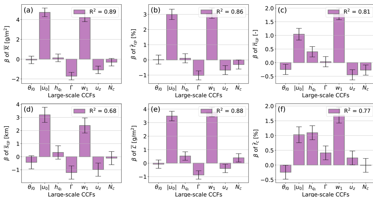
Figure A3. Cloud-field response to large-scale cloud-controlling factors and cloud droplet number perturbations. The standardized \beta coefficients of the multiple regression analysis for the (a) rainwater path ( \bar{\mathcal{R}} ), (b) cold-pool fraction ( \bar{f}_{cp} ), (c) cold-pool number ( \bar{n}_{cp} ), (d) cold-pool size ( \bar{s}_{cp} ) (e) liquid water path ( \bar{\mathcal{L}} ), and (f) cloud fraction ( \bar{f}_c ), all averaged over the last 2 d of the LESs of the Cloud Botany ensemble. The error bars show the 95 % confidence interval for each regressor. The larger the distance of the confidence interval from zero, the more significant the corresponding regressor. The p values of the F test of all models are smaller than 10^{-15} .
