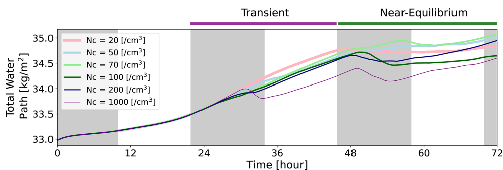
Figure A2. Total water path time series for several values of N_c . The figure shows the development of the domain-mean total water path, which is the sum of both the cloud water and water vapor paths. The transient and near-equilibrium phases are marked by purple and green, respectively.
