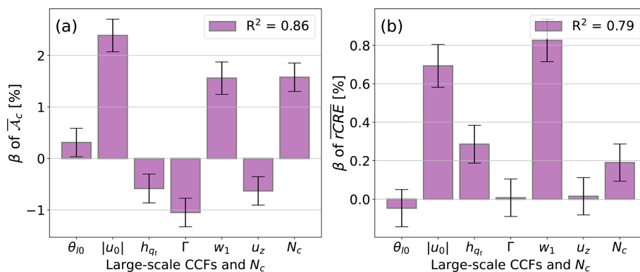
Figure 9. Cloud-field response to large-scale cloud-controlling factors and cloud droplet number concentration. The standardized \beta coefficients of the multiple regression analysis for (a) cloud albedo ( \mathcal{A}_c ) and (b) relative cloud radiative effect (rCRE), all averaged over the last 2 d of the LESs of the Cloud Botany ensemble. The error bars show the 95 % confidence interval for each regressor. The p values of the F test of all models are smaller than 10^{-22} .
