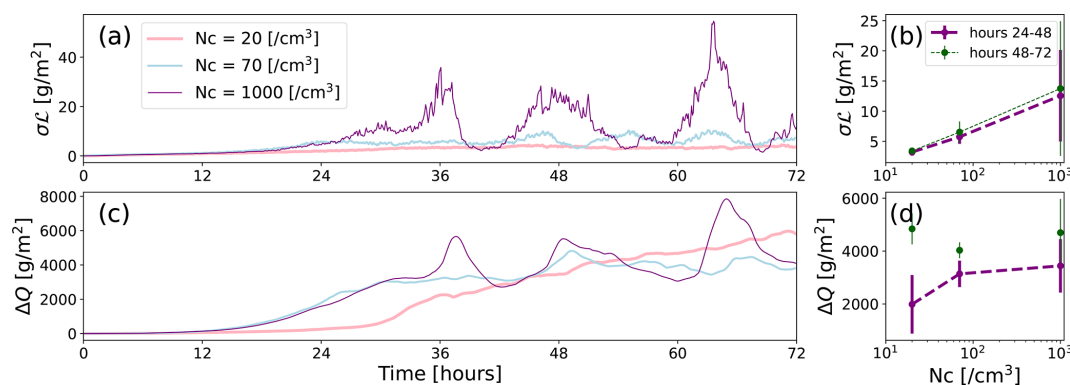
Figure 6. Dependence of mesoscale organization of cloud fields on N_c . Panels (a) and (c) show the time series of the spatial standard deviation of the liquid water path \sigma_L and the difference between the 5th and 95th percentiles of the mesoscale total moisture anomaly fields \Delta Q for the simulations without the diurnal cycle of insolation. Panels (b) and (d) show their responses to N_c for hours 24–48 in purple and hours 48–72 in green. Dashed lines are added as a visual guide where the mean values have a trend.
