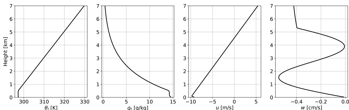
Figure 2. Large-scale and initial conditions of the simulation for potential temperature ( \theta_t ), total moisture ( q_t ), horizontal wind ( u ), and updraft ( w ) following the assumptions of the Cloud Botany ensemble (Jansson et al., 2023a) with parameter values of sea-surface (potential) temperature \theta_{l0} = 299 K, near-surface wind speed u_0 = -10.6 m s -1 , moisture scale height h_{q_t} = 1810 m, temperature lapse rate \Gamma = 5 K km -1 , large-scale vertical velocity variability w_1 = 0.0393 cm s -1 , and horizontal wind shear u_z = 0.0022 (m s -1 ) m -1 .
