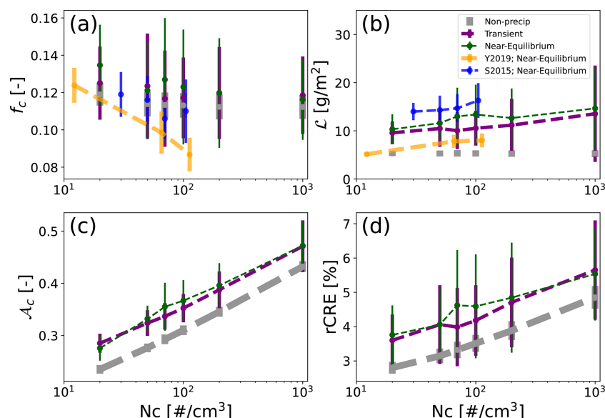
Figure 8. Sensitivity of the relative cloud radiative effect to cloud droplet number. Panels (a)–(d) show the response of the cloud fraction ( f_c ), domain-mean liquid water path ( L ), cloud albedo ( A_c ), and relative cloud radiative effect (rCRE) to N_c during the non-precipitating (dark gray), transient (purple), and near-equilibrium (green) phases. The results from Yamaguchi et al. (2019b) averaged over the last 20 h of their simulations are shown in orange. The results from Seifert et al. (2015) for their near-equilibrium state are shown in blue. Note that Yamaguchi et al. (2019b) and Seifert et al. (2015) do not report on the cloud albedo and rCRE in their studies. Dashed lines are added as a visual guide where there is a trend.
