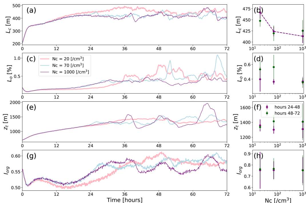
Figure A1. Dependence of several mesoscale cloud organization metrics on N_c . Panels (a), (c), (e), and (g) show the time series of the domain-mean size of cloud objects ( L_c ), the mean fraction of the open-sky areas ( L_o ), the domain-mean of cloud-top height ( z_t ), and the degree of organization ( I_{org} ) for the simulations without the diurnal cycle of insolation. Panels (b), (d), (f), and (h) show their mean responses to N_c for hours 24–48 in purple and 48–72 in green. The dashed line is shown as a visual guide where there is a trend.
