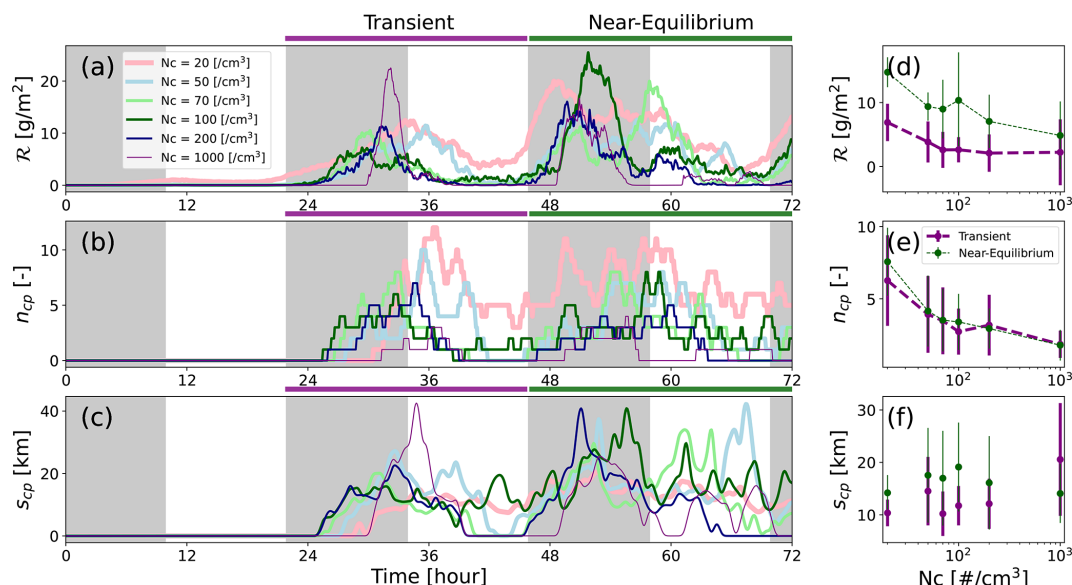
Figure 7. Effects of the diurnal cycle of insolation on the evolution and N_c response of rain and cold pools. Panels (a)–(c) show time series of the rainwater path ( R ), cold-pool number ( n_{cp} ), and cold-pool size ( s_{cp} ) for simulations with the diurnal cycle of solar incoming radiation. Nighttime is shown by the gray color. Solid lines shown for cold-pool number and size provide a guide to the eye obtained through Gaussian filtering of the original data points. Note that there is significant precipitation in the N_c = 20 \text{ cm}^{-3} case before cold pools with diameters larger than the 5 km threshold appear. Panels (d), (e), and (f) show the response of R , n_{cp} , and s_{cp} to N_c during the transient (purple) and near-equilibrium (green) phases, which are marked in the time series plots (a), (b), and (c), respectively. Dashed lines are added as a visual guide where there is a trend.
