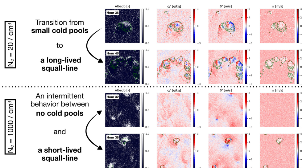
Figure 5. Effects of cold pools on the organization of the (sub-)cloud layer properties for the simulations without a diurnal cycle and with N_c = 20 and N_c = 1000 \text{ cm}^{-3} . For each condition, columns 1–4 indicate the 2D top views of cloud albedo, total moisture anomalies ( q'_t ) at the 200 m level, the horizontal wind speed anomalies ( U' ) at the first level of the model, and the vertical velocity ( w ) at 200 m height. The dashed green contour line marks the cold-pool boundaries quantified from the mixed-layer height fields. In the U' fields, red indicates that cold pools accelerate the wind, whereas blue indicates that they decelerate it.
