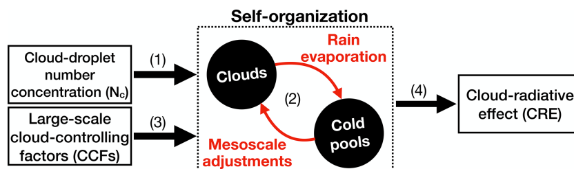
Figure 1. Conceptual picture of the study. The diagram summarizes how (link 1) cloud fields respond to changes in N_c and how (link 2) cold pools feed back to clouds (self-organization). The diagram also shows that the trade-cumulus system is forced by (link 3) the large-scale cloud-controlling factors (CCFs) whose relative importance for (link 4) the cloud radiative effect will be quantified compared to N_c .
