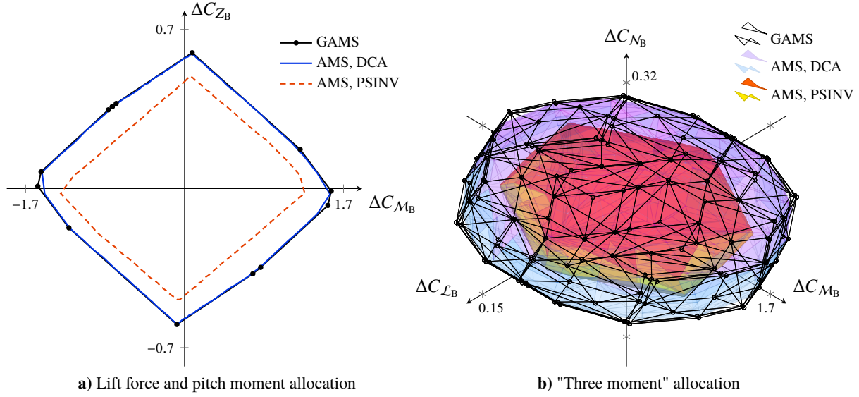
Fig. 5 Comparison of GAMS with AMS of different CA methods in \mathbb{R}^2 (left) and \mathbb{R}^3 (right), for \alpha = 0^\circ , \beta = 0^\circ and M_\infty = 0.5 at standard sea level conditions. The DCA method is able to attain the complete GAMS, while the PSINV only a subset of it.
