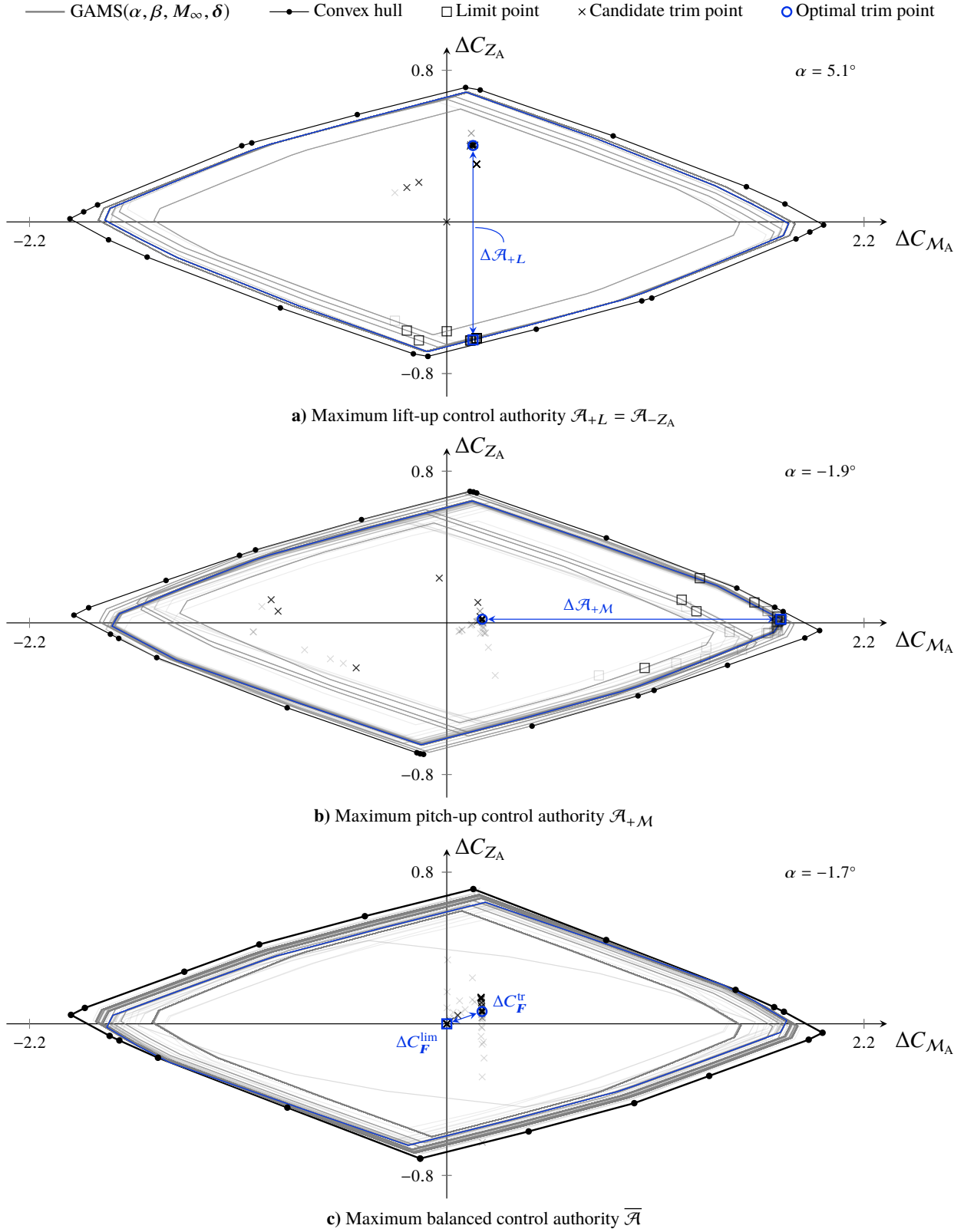
Fig. 7 Visualization in Moment Space of the trim optimization method presented in Sec. IV. Imposed trim conditions at sea level altitude: V^{\text{tr}} = 170 \text{ m} \cdot \text{s}^{-1} , \gamma^{\text{tr}} = 0 . Non-linear, 3-DoF longitudinal-symmetric flight simulations.
