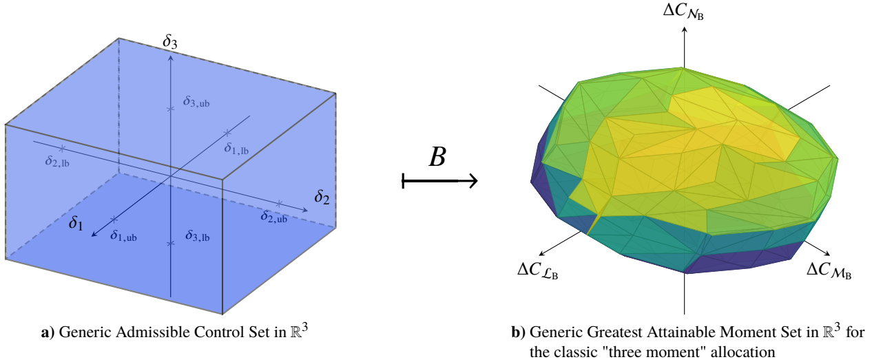
Fig. 3 Mapping of the Admissible Control Set (ACS) to the Greatest Attainable Moment Set (GAMS) through the control effectiveness matrix B . In this specific example, both the AMS and the GAMS are subspaces of \mathbb{R}^3 .
