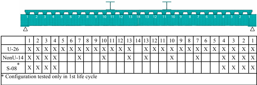
Fig. 4. Testing program
