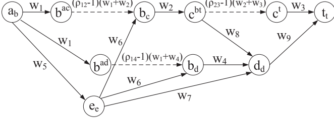
Fig. 4: Auxiliary graph of Fig. 3 for the SPDCM problem under the nodal deterministic correlated model.
