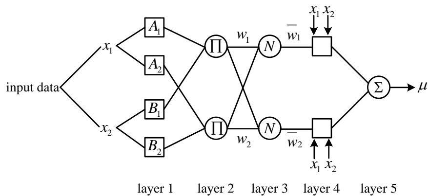
Figure 1. ANFIS structure.
