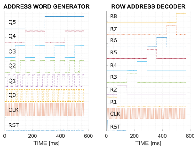
Figure 6: Measurement results of the address word generator and row address decoder circuits. The address word ( Q0-Q5 ) and row selection signals ( R1-8 ) are probed to verify correct operation. The global clock ( CLK ) and reset ( RST ) input signals are also probed and included.
