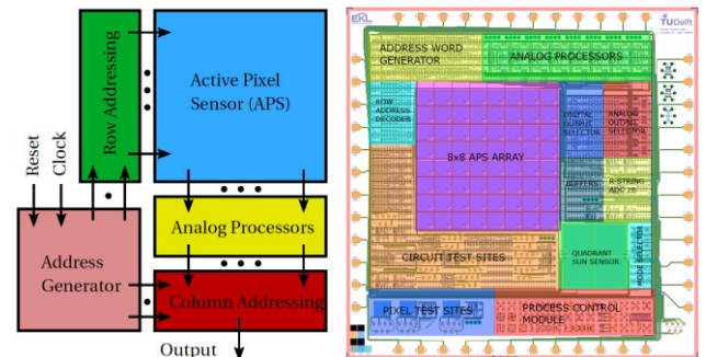
Figure 4: Functional design overview of the 8x8 pixel array with readout circuitry block diagram (left) and highlighted functional blocks in the layout hardware design of the 10x10mm chip (right).
