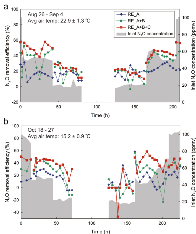
Figure 2. Performance of the bench-scale biotrickling filtration system during the short-term experiments performed with a 40 h \text{N}_2\text{O} starvation in (a) August and (b) October 2019. The cumulative \text{N}_2\text{O} removal efficiencies after treatment in the filter columns A (◆), B (●), and C (■) are presented. The shaded areas represent the measured inlet \text{N}_2\text{O} concentrations. The result from the replicate short-term experiment performed in September 2019 is shown in Figure S6.
