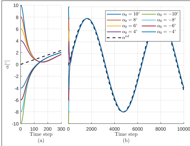
Fig. 5. The tracking performance using the GDHP algorithm with different initial angle of attack.
