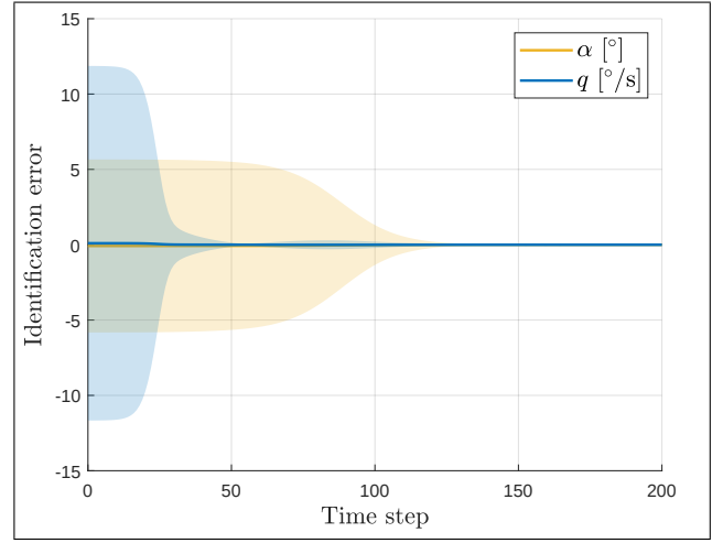
Fig. 3. The system identification errors.
