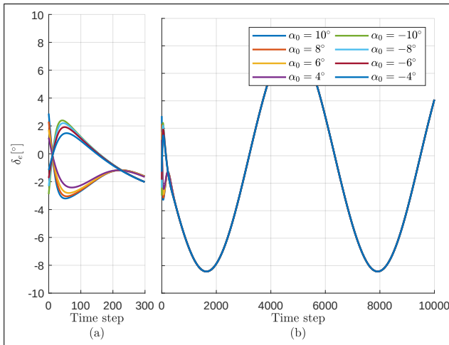
Fig. 6. The control input performance using the GDHP algorithm with different initial angle of attack.
