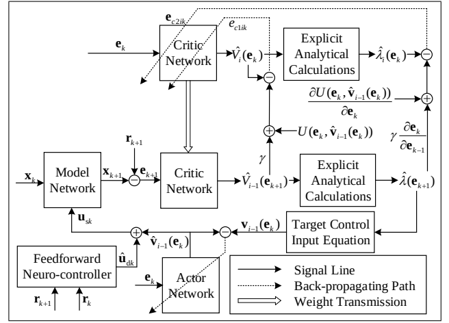
Fig. 1. The architecture diagram of the iterative GDHP algorithm (adapted from [9]).
