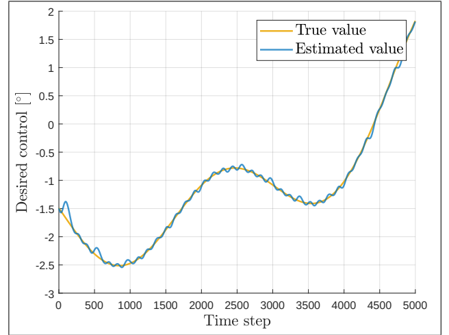
Fig. 4. Comparison between the estimated desired control produced by the feedforward neuro-controller and the true value.
