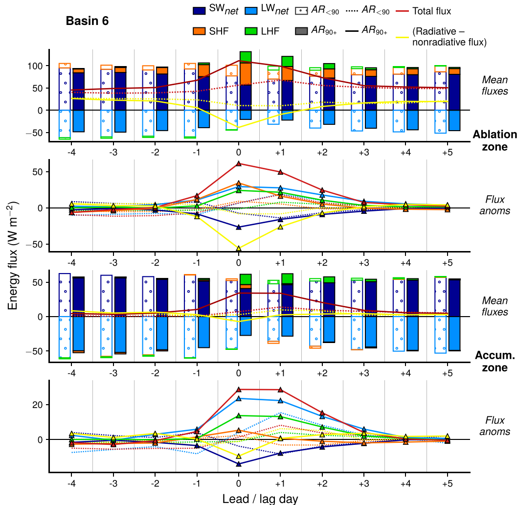
FIG. 3. Composite mean and anomalies of MAR surface energy balance terms averaged over the ablation zone and accumulation zone of basin 6 for the days surrounding AR_{<90} and AR_{90+} events. Also plotted is the difference between summed radiative and nonradiative flux terms (yellow lines) and the sum of all terms (red lines).
