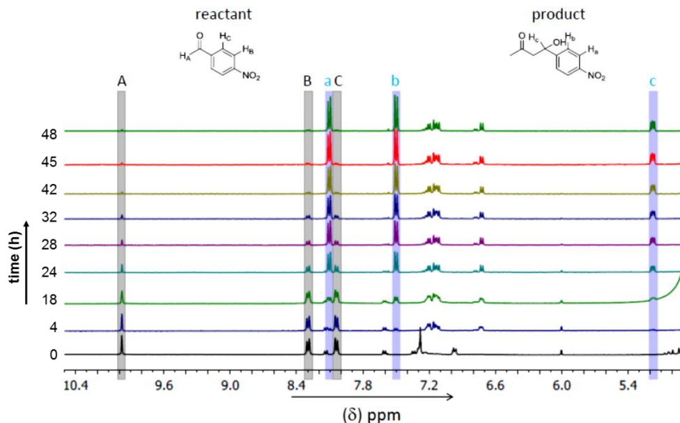
Figure S3.11: ^1\text{H} NMR (partial) spectral analysis of enzyme triggered direct aldol reaction using PP-3 in phosphate buffer (100 mM, pH 7.4) at room temperature in different time interval.
