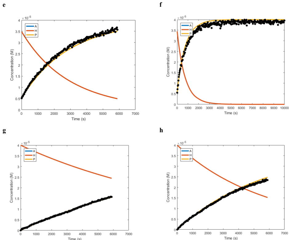
Figure S4.8: Best fits found with a least square error fit with Matlab for the concentration profiles of the formation of hydrazone 6 (black dots) compared with the kinetic model (product 6 : yellow line, aldehyde 4 : blue line (not visible because of the scale), hydrazide 5 : red line). Reaction conditions: 0.4 mM aldehyde 4 , 0.040 M hydrazide 5 in 10 mM phosphate buffer pH 6.0, 25 °C. (a) Uncatalysed reaction, (b) reaction with catalyst 1 , (c) reaction with CB[7], (d) reaction used to fit k_4 with CB[7] (0.84 mM) and catalyst 1 (0.4 mM), (e) with CB[7] (0.07 mM) and catalyst 1 (0.4 mM), (f) with CB[7] (0.42 mM) and catalyst 1 (1.8 mM), (g) with CB[7] (0.42 mM) and catalyst 1 (0.4 mM), (h) with CB[7] (0.28 mM) and catalyst 1 (0.4 mM).
