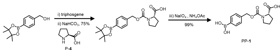
Scheme S3.1: Synthetic pathway for the preparation of PP-1.
