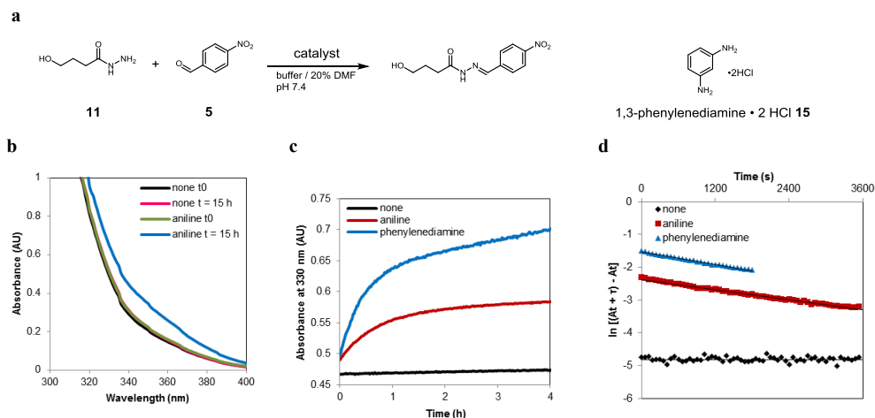
Figure 5.1. The hydrazone formation reaction 9 and response to aniline 1 and 1,3-phenylenediamine ·2HCl 15 catalysis. Reaction conditions: 0.020 mM hydrazide 11 , 0.5 mM aldehyde 5 , 0.5 mM 1 or 0.5 mM 15 catalyst in 20% DMF in 100 mM sodium phosphate buffer pH 7.4 ( a ) Reaction 9 between hydrazide 11 and aldehyde 5 . ( b ) Absorbance spectra of the reaction mixtures for the uncatalysed reaction at t0 (black line) and at t = 15 h (magenta line), for the reaction catalysed by 1 at t0 (green line), at t = 15 h (blue line). ( c ) Hydrazone formation followed over time for the uncatalysed reaction (black), for the reaction catalysed by 1 (red) and for the reaction catalysed by 15 (blue). ( d ) The first-order rate constants were determined by Guggenheim fits, uncatalysed reaction (black), reaction catalysed by 1 (red), reaction catalysed by 15 (blue).
