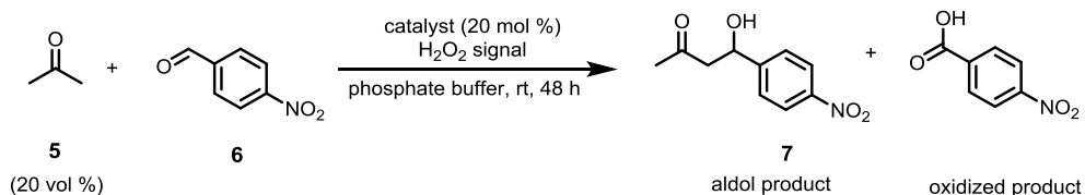
Scheme S3.5: Aldol formation and the oxidation of 4-nitrobenzaldehyde 6 .
