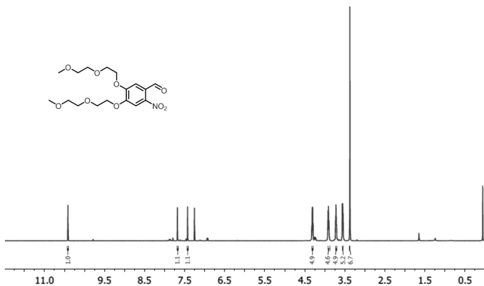
Figure S3.19: ^1\text{H} NMR spectrum of 4,5-bis(2-(2-methoxyethoxy)ethoxy)-2-nitrobenzaldehyde in \text{CDCl}_3 at 25 °C.
