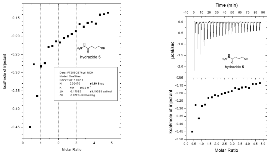
Figure S4.5: ITC measurements for hydrazide 5. The binding constant was too low to determine.
