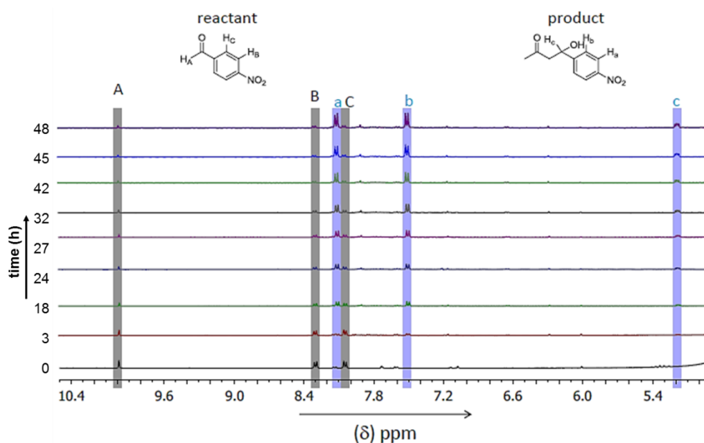
Figure S3.10: 1 H NMR (partial) spectral analysis of light triggered direct aldol reaction using PP-2 in phosphate buffer (100 mM, pH 7.4) at room temperature at different time intervals.
