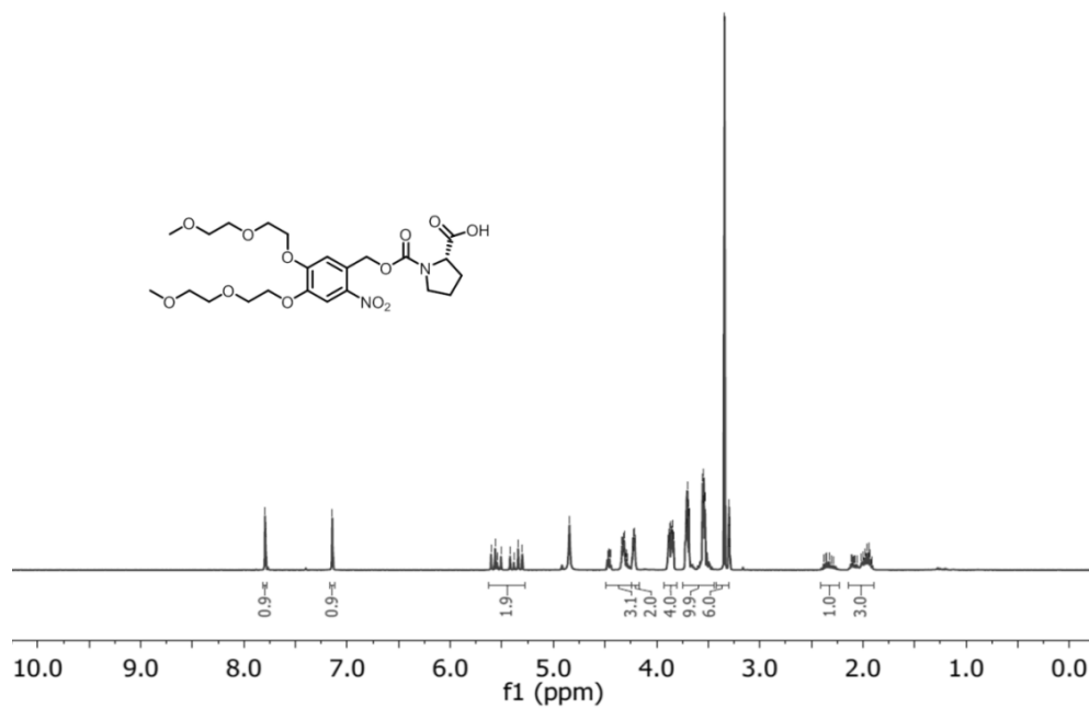
Figure S3.23: ^1\text{H} NMR spectrum of PP-2 in \text{CD}_3\text{OD} at 25^\circ\text{C} .
