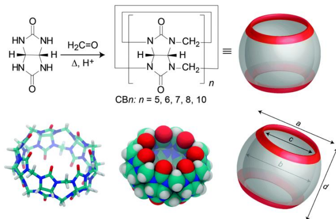
Figure 1.10: The macromolecular host molecule cucurbit[n]uril consists of glycouril units. 62 Reprinted from reference 62.
