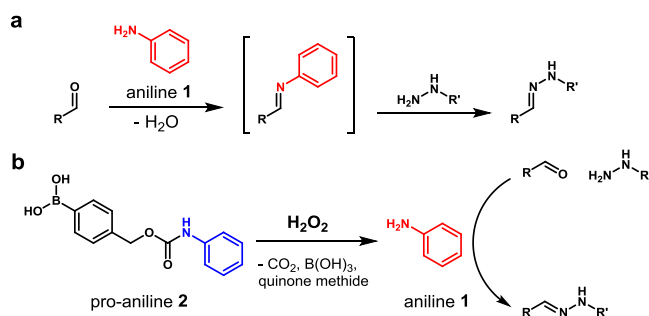
Scheme 5.1. Catalysis of hydrazone formation. (a) Hydrazone formation: the reaction between an aldehyde and a hydrazide catalysed by aniline 1 . (b) The pro-catalyst pro-aniline 2 and the chemical signal H 2 O 2 react to release the organocatalyst aniline 1 which catalyses hydrazone formation between an aldehyde and a hydrazide. [8]
