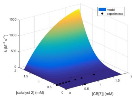
Figure S4.13: Kinetic model defined by eq. 4.3 fits total reaction rate constants for different concentrations of CB[7] and catalyst 2 . (a) 0.42 mM CB[7], 0 – 1.8 mM catalyst 2 , the model fits the experimental values with an R^2 of 0.855. (b) 0.4 mM catalyst 2 , 0 – 0.84 mM CB[7], the model fits the experimental values with an R^2 of 0.997. (c) 0 – 1.8 mM catalyst 2 , 0 – 0.84 mM CB[7].
