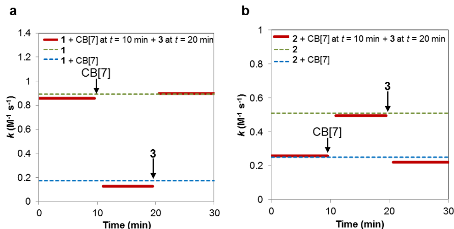
Figure 4.3: Using cucurbit[7]uril (CB[7]) to control hydrazone formation by reversibly binding to the catalyst. Conditions: 0.4 mM aldehyde 4 , 0.040 M hydrazide 5 , 0.4 mM catalyst 1 , 0.4 mM catalyst 2 , 0.42 mM CB[7], 0.8 mM super guest 3 in 10 mM phosphate buffer pH 6.0, 25 °C. The second-order reaction rate constants ( \text{M}^{-1} \text{s}^{-1} ) were determined using the Guggenheim time lag method. 28, 29 (a) The second-order reaction rate constant ( \text{M}^{-1} \text{s}^{-1} ) with catalyst 1 , CB[7] (0.42 mM) is added after 10 min and super guest 3 (0.8 mM) is added after 20 min (red line). For comparison, the second-order rate constant with catalyst 1 (green line) and the second-order rate constant with catalyst 1 and CB[7] (blue line). (b) The second-order reaction rate constant ( \text{M}^{-1} \text{s}^{-1} ) with catalyst 2 , CB[7] (0.42 mM) is added after 10 min and super guest 3 (0.8 mM) is added after 20 min (red line). For comparison, the second-order rate constant with catalyst 1 (green line) and the second-order rate constant with catalyst 1 and CB[7] (blue line).
