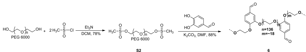
Scheme S2.3: Synthetic route to form PEG-aldehyde copolymer 6 .
