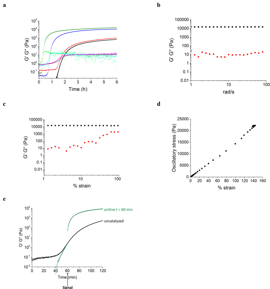
Supplementary Figure S2.5: Rheological data of the polymer gel. Total volume of the gels is 0.6 mL. Composition of the gels: 140 mg/mL polymer aldehyde 6 , 10 mM aniline 2 or 10 mM pro-aniline 1 , 10 mM hydrazide 7 , 20% DMF in 100 mM phosphate buffer pH 6.0. (a) Time sweep, G' and G'' measured during the formation of the gel, uncatalyzed G' (black), uncatalyzed G'' (grey), aniline 2 G' (green), aniline 2 G'' (light green), pro-aniline 1 G' (red), pro-aniline 1 G'' (pink), pro-aniline 1 + H_2O_2 (blue), pro-aniline 1 + H_2O_2 (light blue). (b) Frequency sweep of polymer gel formed with aniline 2 (10 mM) G' (black), G'' (red). (c) Strain sweep of polymer gel formed with aniline 2 (10 mM), G' (black), G'' (red). (d) Stress/strain curve of polymer gel formed with aniline 2 (10 mM) G' (black), G'' (red). (e) Time sweep, G' and G'' measured during the formation of the gel (total volume 1 mL), aniline 2 is added after 60 minutes, uncatalyzed (black), catalyzed and aniline 2 (50 \mu L, 200 mM) added at t = 60 min (green).
