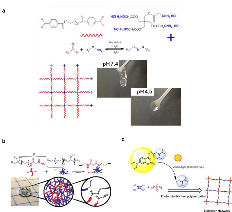
Figure 1.4: Materials that can be controlled by catalysis. (a) The properties of a gel featuring oxime bonds is controlled by acid catalysis. 21 Reprinted from reference 21. (b) A gel featuring hydrazone bonds is controlled by acid catalysis. 22 Reprinted from reference 22. (c) The formation of a polymer network featuring thiol-Michael bonds is controlled by a visible-light-sensitive photobase generator. 24 Reprinted from reference 24.
