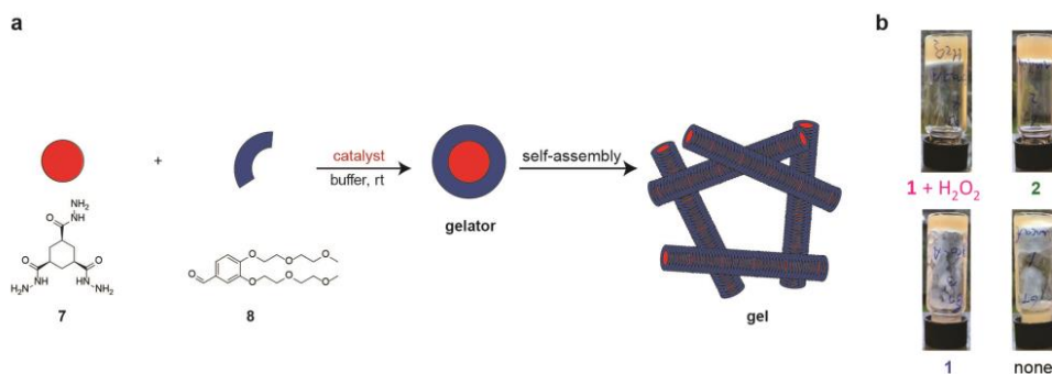
Figure 2.4: Supramolecular gel formation controlled by the activation of pro-aniline 1 . To demonstrate the versatility of the pro-aniline system, we used the pro-aniline 1 to control the formation of a supramolecular gel. 18 (a) Schematic representation of the two water-soluble building blocks aldehyde 8 and hydrazide 7 that react by hydrazone formation in the presence of a catalyst to form a gelator which stacks into fibers and forms a gel. (b) We performed a gelation test for the supramolecular gel in vials. Photographs of gelation samples taken after 15 h of reaction time for the mixture (16 mM hydrazide 7 and 96 mM aldehyde 8 in 20% methanol in phosphate buffer, 100 mM, pH 6.0) with, top left: pro-aniline 1 (10 mM) and H 2 O 2 (100 mM), top right: aniline 2 (10 mM), bottom left: unactivated pro-aniline 1 (10 mM), bottom right: without catalyst. The mixtures with aniline 2 or pro-aniline 1 with H 2 O 2 formed gels after 15 h, whereas the mixture without catalyst or with unactivated pro-aniline 1 did not form gels, although the viscosity of the mixtures was increased after 15 h.
