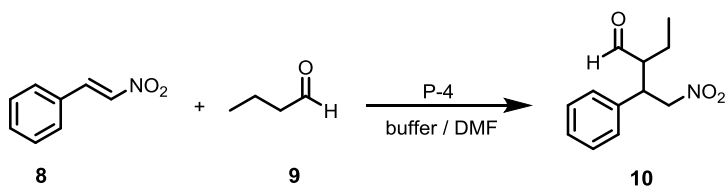
Scheme S3.6: Michael reaction between trans - \beta -nitrostyrene 8 and butanal 9 .
