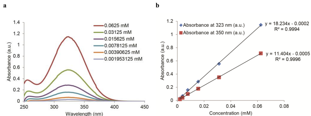
Supplementary Figure S2.6: (a-b) Calibration line of hydrazone 5 measured in 20% DMF in phosphate buffer (100 mM, pH 7.4). The extinction coefficient of hydrazone 5 under these conditions at the absorbance maximum of 323 nm is 2.1 \pm 0.13 \cdot 10^4 \text{ M}^{-1} \text{ s}^{-1} . The extinction coefficient at 350 nm is 1.3 \pm 0.087 \cdot 10^4 \text{ M}^{-1} \text{ s}^{-1} . The errors are the standard error of mean (the standard deviation divided by the square root of the number of measurements).
