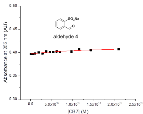
Figure S4.7: UV/vis titration measurement to determine the binding constant of aldehyde 4 with CB[7]. The binding constant was too low to determine.
