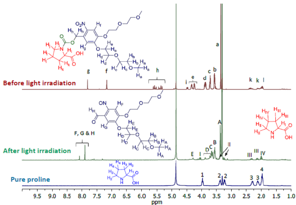
Figure S3.4: ^1\text{H} NMR analysis of light triggered proline release from PP-2 in \text{CD}_3\text{OD} at 25^\circ\text{C} – before (top in red) and after light irradiation (middle in green). The released proline has a comparable spectrum to pure proline (bottom in blue).
