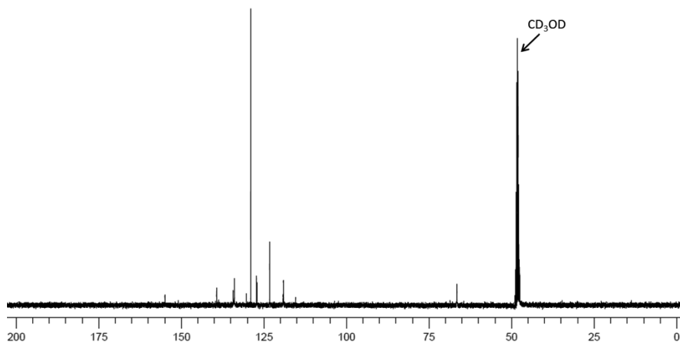
Supplementary Figure S2.12: ^{13}\text{C} NMR spectrum of pro-aniline 1 in \text{CD}_3\text{OD} .
