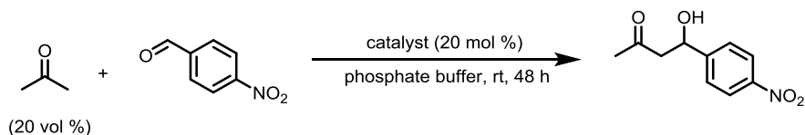
Scheme S3.4: General reaction scheme for direct aldol reaction.
