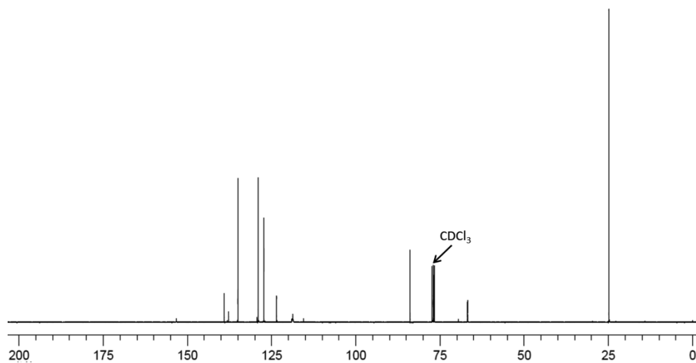
Supplementary Figure S2.10: 13 C NMR spectrum of pro-aniline boronate ester S1 in CDCl 3 .
