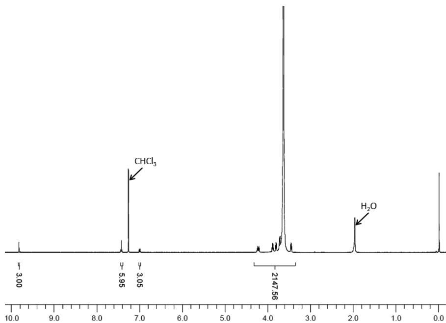
Supplementary Figure S2.16: ^1\text{H} NMR spectrum of PEG-aldehyde 6 in \text{CDCl}_3 .
