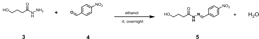
Scheme S2.2: Synthetic route to form hydrazone 5 .
