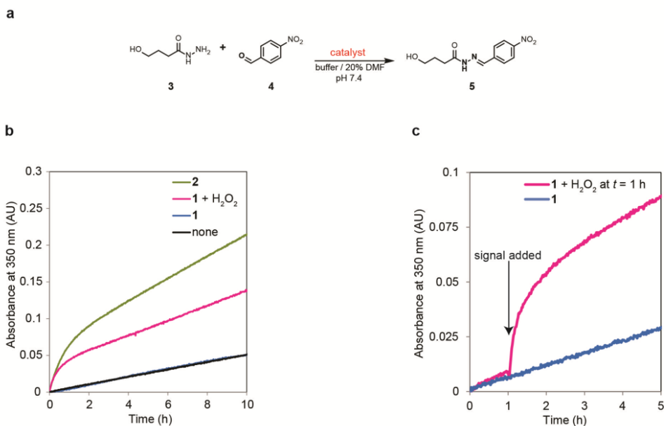
Figure 2.2: Control over the rate of hydrazone formation by activation of the catalyst. (a) Model hydrazone formation reaction, yielding the UV active probe 5 . Reaction conditions: 0.1 mM hydrazide 3 , 0.5 mM aldehyde 4 , 0.5 mM pro-aniline 1 , 0.5 mM aniline 2 , 2.5 mM (5 equivalents) \text{H}_2\text{O}_2 in 20% dimethylformamide (DMF) in phosphate buffer (100 mM, pH 7.4). All experiments were carried out at 25 °C. The 20% DMF was used to ensure that 1 was completely dissolved. The rate of formation of 5 is 10 times higher when using \text{H}_2\text{O}_2 -activated pro-aniline 1 than for unactivated pro-aniline 1 . (b) Formation of 5 over time, without catalyst (black line), in the presence of aniline 2 (green line), in the presence of unactivated pro-aniline 1 (blue line) and in the presence of activated pro-aniline 1 with 5 equivalents of \text{H}_2\text{O}_2 (magenta line). (c) The rate of formation of 5 can be controlled during the process by adding a chemical signal (5 equivalents of \text{H}_2\text{O}_2 here after 1 hour), liberating the catalyst. Reaction with pro-aniline 1 and subsequent addition of \text{H}_2\text{O}_2 (magenta line), reaction with unactivated pro-aniline 1 (blue dashed line). After addition of the chemical signal an immediate response was observed: the reaction rate increased 9-fold.
