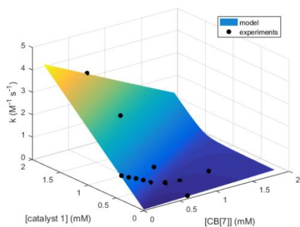
Figure S4.9: Kinetic model defined by eq. 4.1 fits total reaction rate constants for different concentrations of CB[7] and catalyst 1 . (a) 0.42 mM CB[7], 0 – 1.8 mM catalyst 1 , the model fits the experimental values with an R^2 of 0.987. (b) 0.4 mM catalyst 1 , 0 – 0.84 mM CB[7], the model fits the experimental values with an R^2 of 0.971. (c) 0 – 1.8 mM catalyst 1 , 0 – 0.84 mM CB[7].
