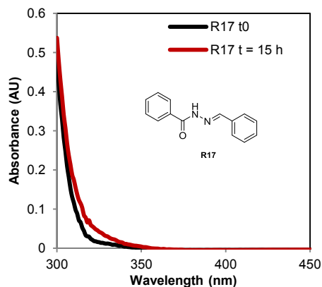
Supplementary Fig. 5.1: Absorbance spectrum of aldehyde and hydrazone mixtures with aniline 1 at t0 (black line) and at t = 15 h (red line). Reaction conditions: 0.020 mM hydrazone, 0.5 mM aldehyde, 0.5 mM aniline 1 , 20% DMF in 100 mM sodium phosphate buffer pH 7.4. R1 means reaction 1 (etc.) from Table 5.1 in the main text. (a) Reaction 1 between hydrazone 3 and aldehyde 4 , (b) reaction 2 between hydrazone 3 and aldehyde 5 , (c) reaction 3 between hydrazone 3 and aldehyde 6 , (d) reaction 4 between hydrazone 7 and aldehyde 8 , (e) reaction 5 between hydrazone 7 and aldehyde 5 , (f) reaction 6 between hydrazone 7 and aldehyde 9 , (g) reaction 7 between hydrazone 7 and aldehyde 10 , (h) reaction 8 between hydrazone 11 and aldehyde 4 , (i) reaction 9 between hydrazone 11 and aldehyde 5 , (j) reaction 10 between hydrazone 12 and aldehyde 4 does not take place, (k) reaction 11 between hydrazone 13 and aldehyde 4 , (l) reaction 12 between hydrazone 14 and aldehyde 4 , (m) reaction 13 between hydrazone 14 and aldehyde 5 , (n) reaction 14 between hydrazone 11 and aldehyde 16 does not take place, (o) reaction 15 between hydrazone 11 and aldehyde 8 , (p) reaction 16 between hydrazone 14 and aldehyde 16 does not take place, (q) reaction 17 between hydrazone 14 and aldehyde 8 , (r) reaction 18 between hydrazone 14 and benzaldehyde 17 does not take place.
