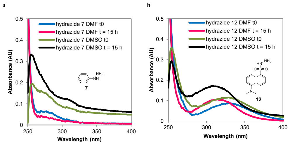
Supplementary Fig. 5.5: Change in absorbance of hydrazides in DMF and in DMSO. (a) Hydrazide 7 in DMF at t0 (blue line), hydrazide 7 in DMF at t = 15 h (magenta line), hydrazide 7 in DMSO at t0 (green line) and hydrazide 7 in DMSO at t = 15 h (black line). (b) Hydrazide 12 in DMF at t0 (blue line), hydrazide 12 in DMF at t = 15 h (magenta line), hydrazide 12 in DMSO at t0 (green line) and hydrazide 12 in DMSO at t = 15 h (black line). Conditions: 0.020 mM hydrazide in 20% DMF or 20% DMSO in 100 mM sodium phosphate buffer pH 7.4.
