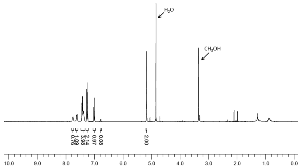
Supplementary Figure S2.11: ^1\text{H} NMR spectrum of pro-aniline 1 in \text{CD}_3\text{OD} .
