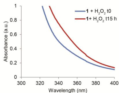
Supplementary Figure S2.7: UV/vis spectra of the reaction mixture of hydrazone formation at t = 0 h (blue lines) and at t = 15 h (red lines). (a) Uncatalyzed reaction, (b) reaction in presence of pro-aniline 1 , (c) reaction in presence of pro-aniline 1 and \text{H}_2\text{O}_2 , (d) reaction in the presence of aniline 2 . Reaction conditions: 0.1 mM hydrazide 3 , 0.5 mM aldehyde 4 in 20% DMF in phosphate buffer (100 mM, pH 7.4) without catalyst, in the presence of either unactivated pro-aniline 1 (0.5 mM), or activated pro-aniline 1 (0.5 mM) with 5 equivalents of \text{H}_2\text{O}_2 (2.5 mM) or aniline 2 (0.5 mM).
