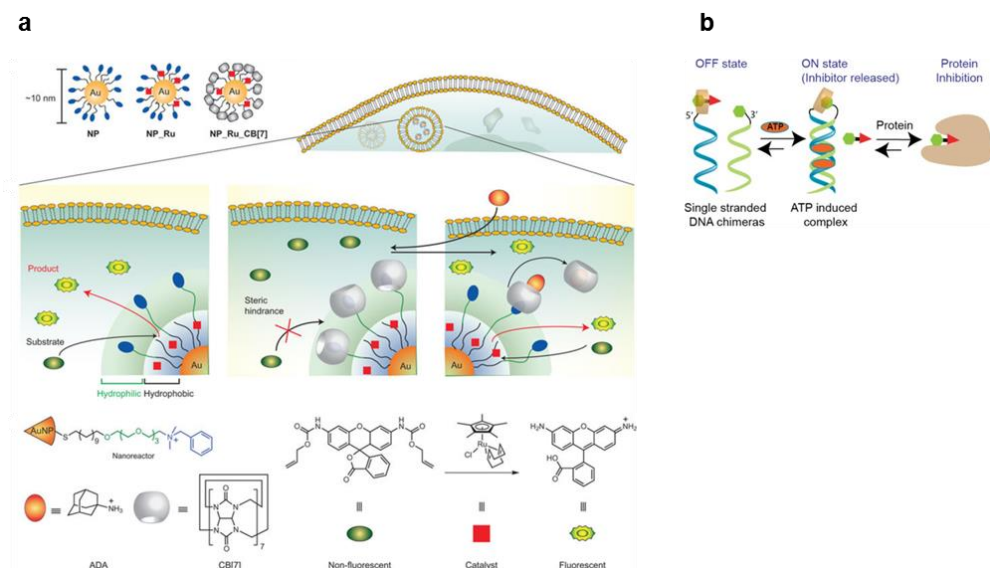
Figure 1.12: Using cucurbiturils to change the activity of catalysts. (a) Cucurbit[7]uril (CB[7]) was used to reversibly block an organometallic catalyst on a gold nanoparticle. 79 Reprinted from reference 79. (b) Cucurbituril was used indirectly to control the activity of an enzyme: addition of ATP (adenosine triphosphate) induces self-assembly of a small DNA strand with a small molecule, which results in release of a protein inhibitor. 81 Reprinted from reference 81.
