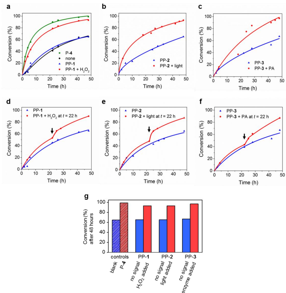
Figure 3.3: Kinetic analysis of the aldol reaction between 4-nitrobenzaldehyde 6 and acetone 5 . Conditions: 10 mM 4-nitrobenzaldehyde 6 , 20 volume % acetone 5 , 2 mM (20 mol%) PP-1, 2 mM (1 eq.) H 2 O 2 in sodium phosphate buffer (100 mM, pH 7.4) with 10 v% D 2 O and 1 mM sodium dodecyl sulfate (SDS). (a) Conversion of the aldol product followed with NMR spectroscopy in the presence of P-4 (green), without catalyst (black), PP-1 without activation (blue), PP-1 and H 2 O 2 (red). (b) Conversion of the aldol reaction in the presence of PP-2 without activation (blue) and in the presence of PP-2 after irradiation with light (red). (c) Conversion of the aldol reaction in the presence of PP-3 without activation (blue) and in the presence of PP-3 after addition of penicillin acylase (PA) (red). (d) Conversion of the aldol reaction in the presence of PP-1 (blue), the signal H 2 O 2 was added after 22 h (red). (e) Conversion of the aldol reaction in the presence of PP-2 (blue), after 22 h, the reaction mixture was irradiated with light (red). (f) Aldol reaction in the presence of PP-3 (blue), after 22 h, penicillin acylase (PA) was added (red). (g) Conversion to the aldol product after 48 hours, in the absence or presence of the appropriate signal. In (d–f) the arrow indicates the moment of signal addition.
