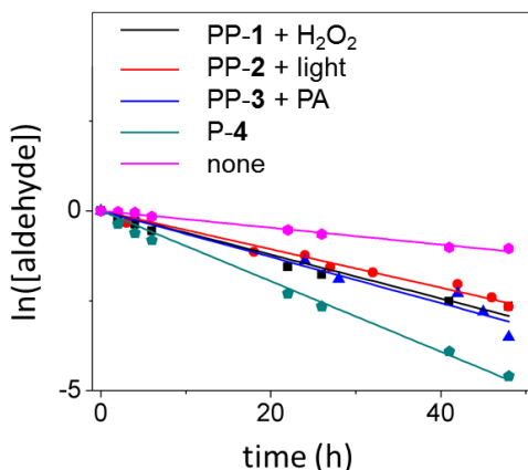
Figure S3.13: Signal triggered proline release and subsequent catalysis of an aldol reaction between 4-nitrobenzaldehyde 6 and acetone 5 in aqueous buffer media (100 mM, pH 7.4), where [\text{aldehyde}] = \ln \left\{ 1 - \frac{[P]_t}{([B]_t + [P]_t)} \right\} . Signal triggered aldol reaction was compared with proline catalysed aldol reaction and background reaction.
