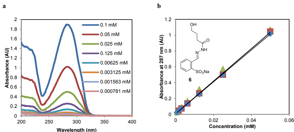
Figure S4.1: Extinction coefficient for hydrazone 6 at 287 nm: (2.03 \pm 0.003) \times 10^4 \text{ M}^{-1} \text{ cm}^{-1} , error is the standard error of the mean ( n = 3 ). (a) UV/vis spectra of hydrazone 6 at different concentrations. (b) Absorbance at 287 nm of hydrazone 6 at different concentrations, the experimental data of 3 experiments are shown.
