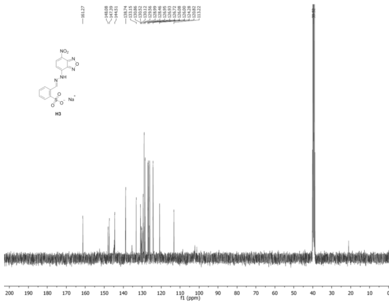
^{13}\text{C} NMR H3 in DMSO- d_6
