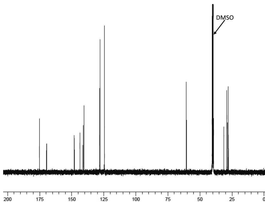
Supplementary Figure S2.14: 13 C NMR spectrum of hydrazone 5 in DMSO-d 6 .
