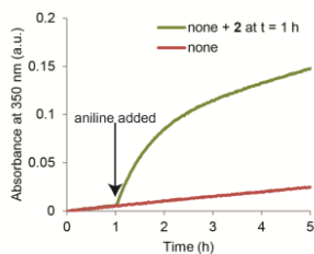
Supplementary Figure S2.3: (a) UV/vis absorbance spectrum measured for aldehyde 4 (0.5 mM) with \text{H}_2\text{O}_2 at t = 0 h and at t = 15 h, the compound remains stable. (b) Absorbance at 350 nm of hydrazone 5 formation followed in UV/vis spectroscopy (conditions: hydrazide 3 (0.1 mM), aldehyde 4 (0.5 mM), 20% DMF in 100 mM phosphate buffer pH 7.4) without catalyst (blue line), with \text{H}_2\text{O}_2 (2.5 mM, red line). \text{H}_2\text{O}_2 has no influence on the reaction rate. (c) UV/vis absorbance spectrum measured for aniline 2 (0.5 mM) at t = 0 h and at t = 15 h, the compound remains stable. (d) Absorbance at 350 nm of hydrazone 5 formation followed in UV/vis spectroscopy (conditions: hydrazide 3 (0.1 mM), aldehyde 4 (0.5 mM), 20% DMF in 100 mM phosphate buffer pH 7.4) with aniline 2 (0.5 mM, blue line), with aniline 2 + boric acid (0.5 mM, red line), with aniline 2 + boric acid + \text{H}_2\text{O}_2 (2.5 mM, green line), with aniline 2 + boric acid + \text{H}_2\text{O}_2 at t = 1 h (2.5 mM, black line). Boric acid has no influence on the catalytic activity of aniline 2 , with and without \text{H}_2\text{O}_2 . (e) Absorbance at 350 nm of hydrazone 5 formation followed in UV/vis spectroscopy (conditions: hydrazide 3 (0.1 mM), aldehyde 4 (0.5 mM), 20% DMF in 100 mM phosphate buffer pH 7.4) without catalyst (red line), aniline 2 was added after 1 hour (green line, 2.5 mM). For more blank experiments, see Supplementary Table 1.
