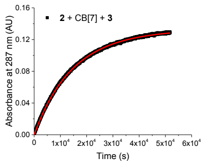
Figure S4.2: Fits of relative absorbance followed at 287 nm of the hydrazone reactions. Experimental data: black squares, fit: red lines. Reaction conditions: 0.4 mM aldehyde 4 , 0.040 M hydrazide 5 , 0.4 mM catalyst 1 , 0.4 mM catalyst 2 , 0.42 mM CB[7], 0.8 mM super guest 3 in 10 mM phosphate buffer pH 6.0, 25 °C. (a) Uncatalysed reaction, (b) reaction with catalyst 1 , (c) reaction with CB[7] + 1 , (d) reaction with 1 + CB[7] + 3 , (e) reaction with catalyst 2 , (f) reaction with 2 + CB[7], (g) reaction with 2 + CB[7] + 3 .
