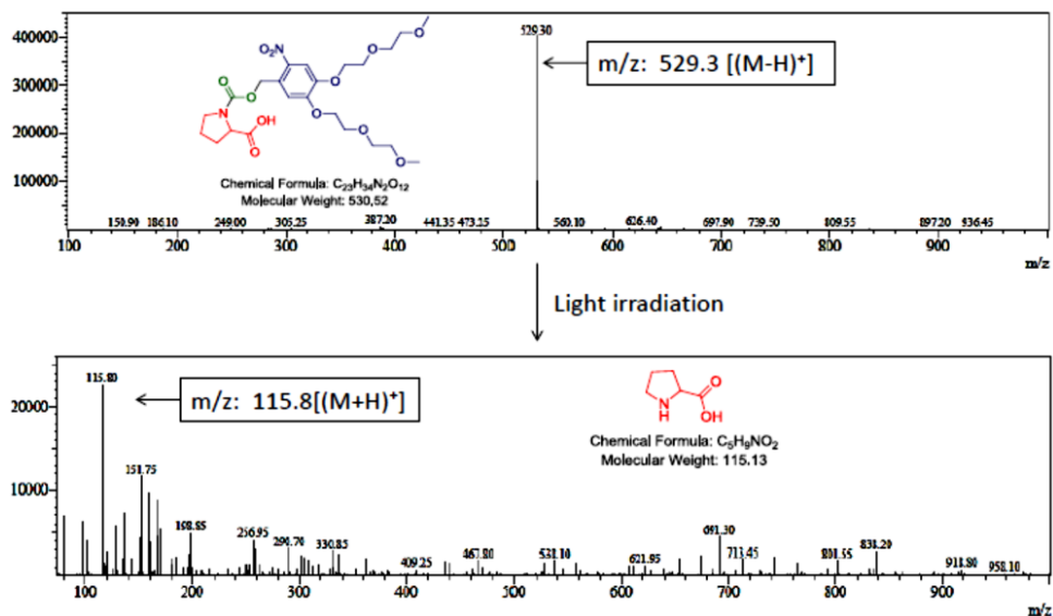
Figure S3.5: Mass spectrometry analysis of proline release from PP-2: before (top) and after (bottom) light irradiation.
