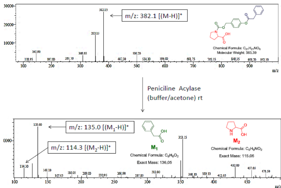
Figure S3.7: Mass spectrometry analysis of enzyme (Penicillin Acylase) triggered proline release from PP-3: before (top) and after (bottom) enzyme treatment.
