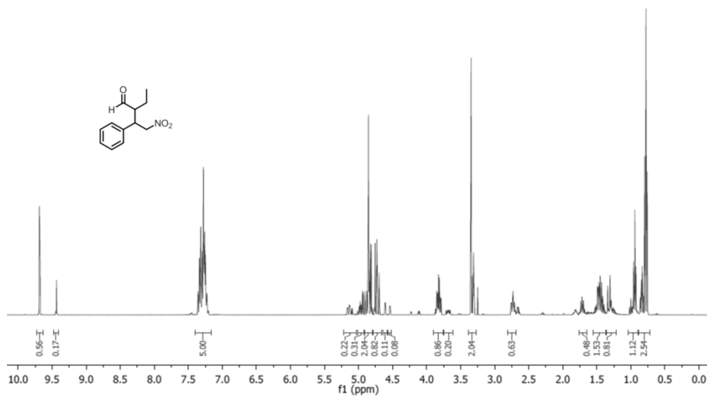
Figure S3.24: 1 H NMR spectrum of the Michael product 10 in CD 3 OD.
