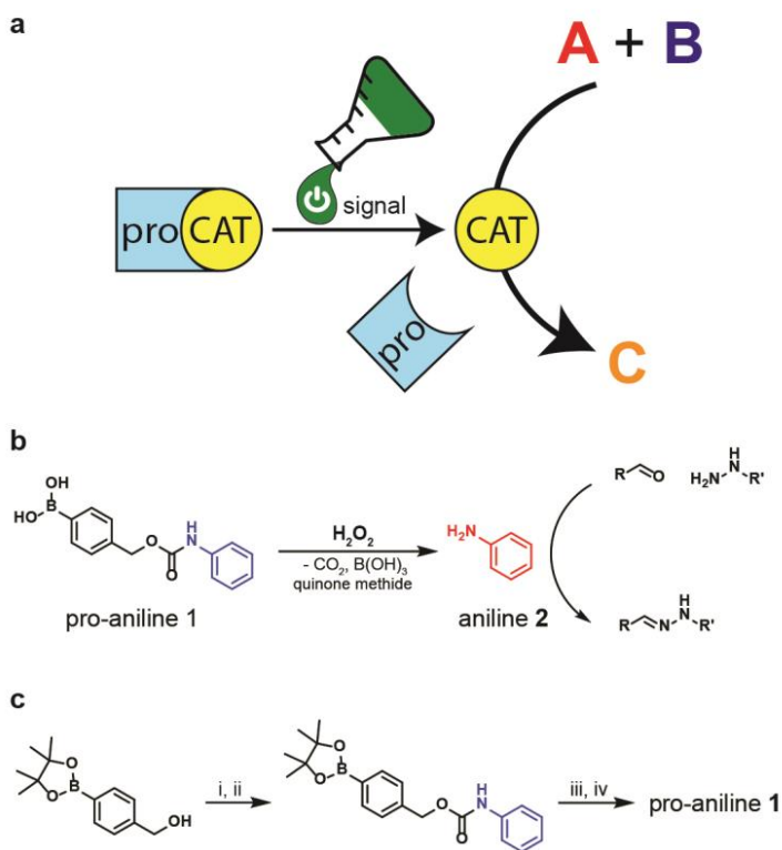
Figure 2.1: Design and synthesis of the protected catalyst. (a) Schematic representation of the activation of a protected catalyst and subsequent catalysis of a chemical reaction. (b) The pro-catalyst pro-aniline 1 and the chemical signal \text{H}_2\text{O}_2 react to release the organocatalyst aniline 2 which catalyzes hydrazone formation between an aldehyde and a hydrazide. (c) Synthetic route for the synthesis of pro-aniline 1 , i) \text{K}_2\text{CO}_3 , triphosgene, 0^\circ\text{C} – room temperature, ii) aniline 2 , \text{NaHCO}_3 , tetrahydrofuran, 0^\circ\text{C} – room temperature, iii) \text{NaIO}_4 , ammonium acetate, room temperature, iv) 1 M aqueous HCl. Total yield over two steps is 64%.
