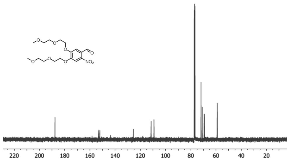
Figure S3.20: ^{13}\text{C} NMR spectrum of 4,5-bis(2-(2-methoxyethoxy)ethoxy)-2-nitrobenzaldehyde in \text{CDCl}_3 at 25 °C.
