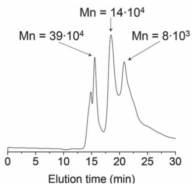
Supplementary Figure S2.17: Gel permeation chromatogram of PEG-aldehyde 6 (10 mg/mL in water).
