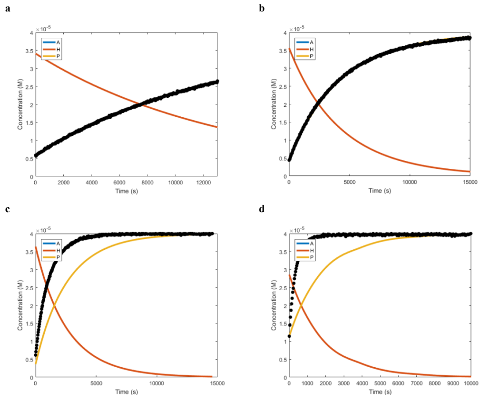
Figure S4.10: Best fits found with a least square error fit with Matlab for the concentration profiles of the formation of hydrazone 6 (black dots) compared with the kinetic model (product 6 : yellow line, aldehyde 4 : blue line (not visible because of the scale), hydrazide 5 : red line). Reaction conditions: 0.4 mM aldehyde 4 , 0.040 M hydrazide 5 in 10 mM phosphate buffer pH 6.0, 25 °C. (a) reaction with catalyst 2 , (b) reaction used to fit k_4 with CB[7] (0.42 mM) and catalyst 2 (0.4 mM), (c) reaction with CB[7] (0.84 mM) and catalyst 2 (0.4 mM), (d) reaction with CB[7] (0.42 mM) and catalyst 2 (1.8 mM).
