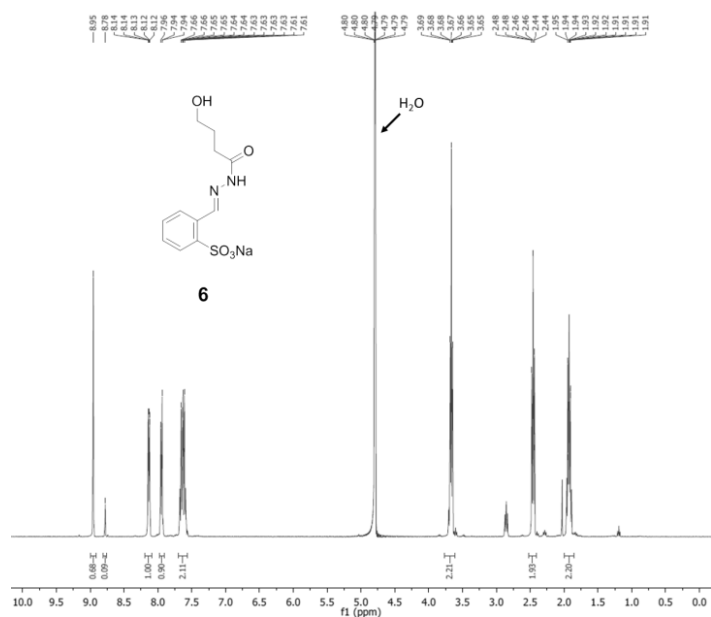
Figure S4.14: 1 H NMR Hydrazone 6 in D 2 O.
