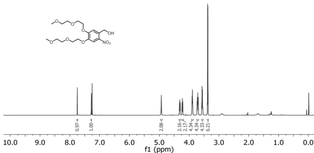
Figure S3.21: 1 H NMR spectrum of 4,5-bis(2-(2-methoxyethoxy)ethoxy)-2-nitrophenyl)methanol in CDCl 3 at 25 °C.
