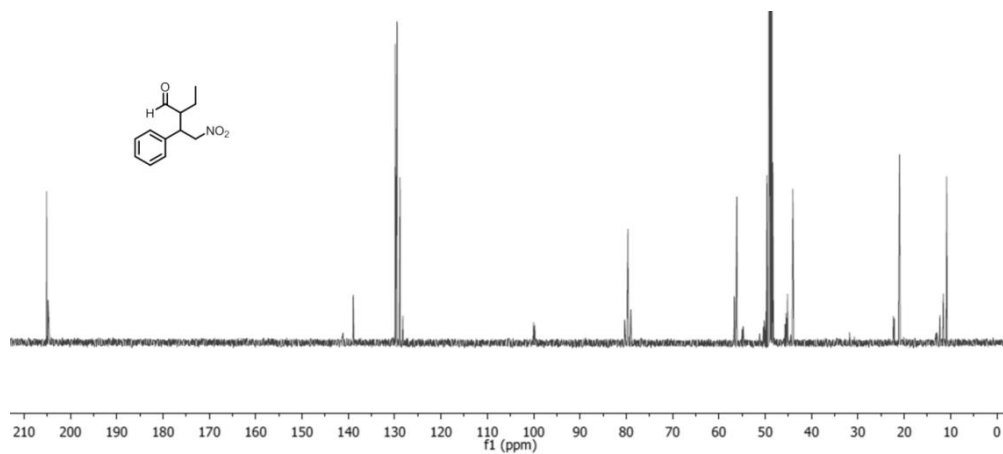
Figure S3.25: 13 C NMR spectrum of the Michael product 10 in CD 3 OD.
