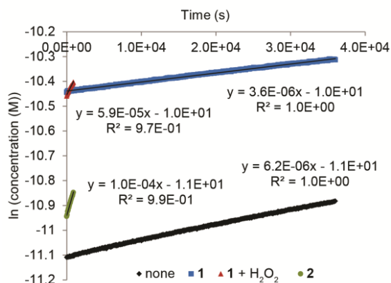
Supplementary Figure S2.8: Plots of \ln (concentration (M)) versus time (s) result in linear graphs, the slope represents the pseudo-first-order rate constant with unit \text{s}^{-1} , without catalyst (black), with pro-aniline 1 (blue), with pro-aniline 1 + H 2 O 2 (red) and with aniline 2 (green). Concentrations were obtained using the extinction coefficient of the product at 350 nm ( 1.3 \pm 0.087 \cdot 10^4 \text{ M}^{-1} \text{ s}^{-1} ). The errors are the standard error of mean (the standard deviation divided by the square root of the number of measurements). Reaction conditions: 0.1 mM hydrazide 3 , 0.5 mM aldehyde 4 in 20% DMF in phosphate buffer (100 mM, pH 7.4) without catalyst, in the presence of either unactivated pro-aniline 1 (0.5 mM), or activated pro-aniline 1 (0.5 mM) with 5 equivalents of H 2 O 2 (2.5 mM) or aniline 2 (0.5 mM).
