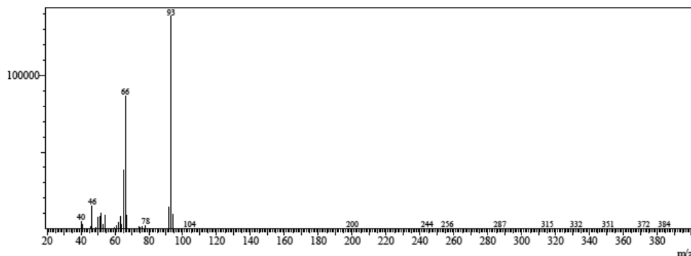
Supplementary Figure S2.1: GC/MS spectrum taken after the reaction of pro-aniline 1 with 18 equivalents of \text{H}_2\text{O}_2 . Conditions: 5 mg, 18 \mu\text{mol} pro-aniline 1 in 0.25 mL ethyl acetate, \text{H}_2\text{O}_2 (18 equivalents, 25.4 \mu\text{L} in 0.25 mL deionized water), stirred for 1 h at room temperature. The reaction mixture was quenched with a saturated sodium thiosulfate solution and the organic layer was used for analysis in GC/MS. Only aniline 2 was detected in the reaction mixture, MS (GC/MS) m/z: 93 [\text{M}]^+\bullet , 66 [\text{C}_5\text{H}_6]^+\bullet (expected m/z = 93.06, 66.05), retention time: 11 min.
