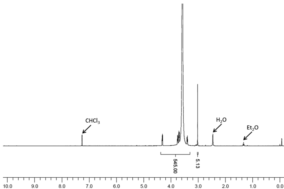
Supplementary Figure S2.15: ^1\text{H} NMR spectrum of PEG-mesylate S2 in \text{CDCl}_3 .
