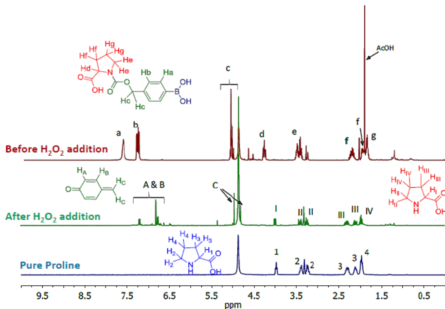
Figure S3.1: 1 H NMR analysis of chemical (H 2 O 2 ) trigger proline release from PP-1 in CD 3 OD at 25 °C: PP-1 before (top in red) and after H 2 O 2 treatment (middle in green). The released proline has comparable spectrum as pure proline (bottom in blue).
