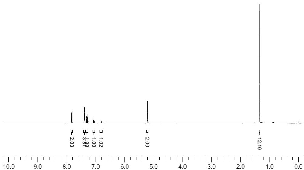
Supplementary Figure S2.9: 1 H NMR spectrum of pro-aniline boronate ester S1 in CDCl 3 .
