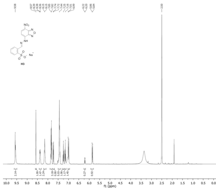
^1\text{H} NMR H3 in DMSO- d_6
