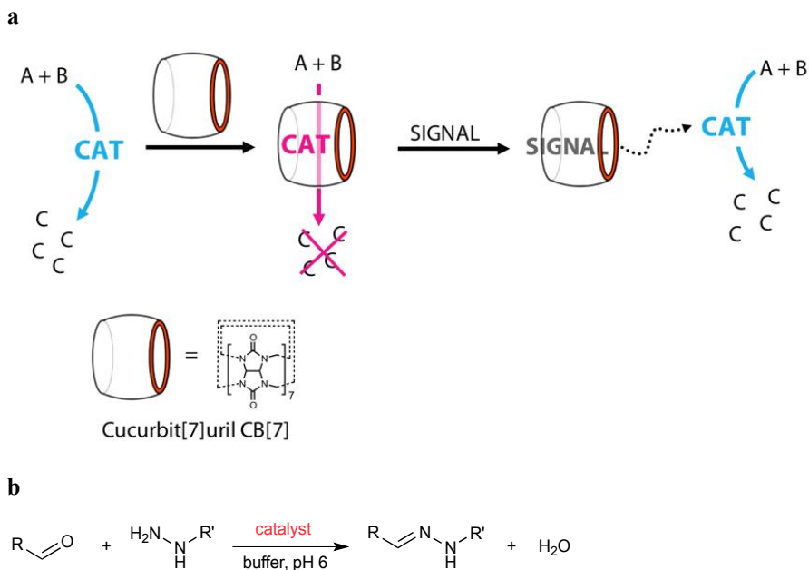
Figure 4.1: Using host-guest chemistry to control the activity of catalysts. (a) Schematic representation of cucurbit[7]uril (CB[7]) binding to the organocatalyst (cat), hindering its catalytic activity. Addition of the stronger binding signal leads to the release of the catalyst and restores its catalytic activity. (b) The hydrazone formation reaction between an aldehyde and hydrazide is catalysed by organocatalysts, such as catalysts 1 and 2 (Table 4.1).
