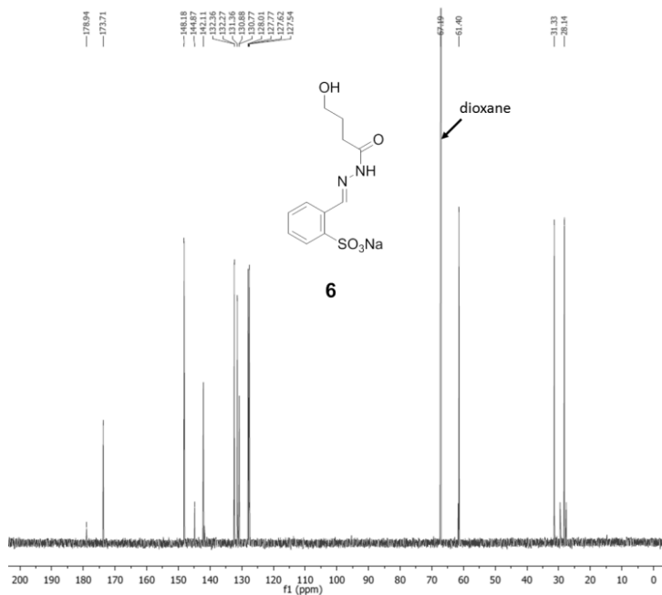
Figure S4.14: 1 H NMR Hydrazone 6 in D 2 O.
