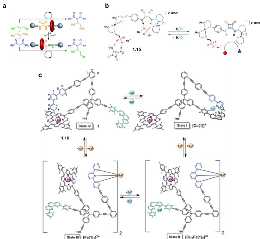
Figure 1.8: Examples of pro-catalysts that can be controlled by chemical signals. (a) A rotaxane-based pH switchable organocatalyst that can be switched between imine catalysis and hydrogen bonded catalysis to result in two different Michael products. 43 Reprinted from reference 43. (b) A chemically activated catalyst for a Michael addition and for the ring opening of lactide. 44 Reprinted from reference 44. (c) A four state catalyst that can be switched using \text{Fe}^{2+} and \text{Cu}^+ cations. The two active states catalyse a two-step reaction: an azide-alkyne click reaction followed by a Michael addition. 45 Reprinted from reference 45.
