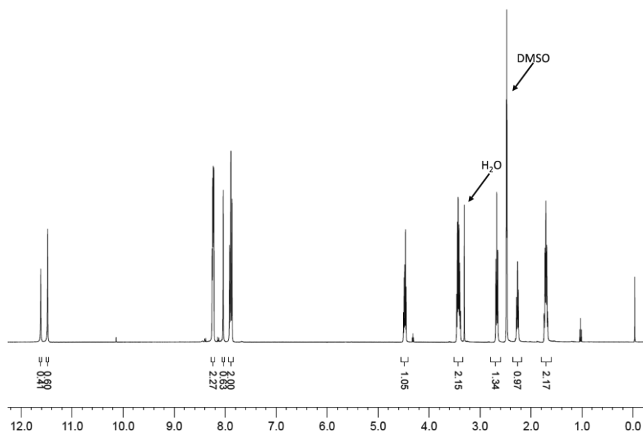
Supplementary Figure S2.13: 1 H NMR spectrum of hydrazone 5 in DMSO-d 6 .
