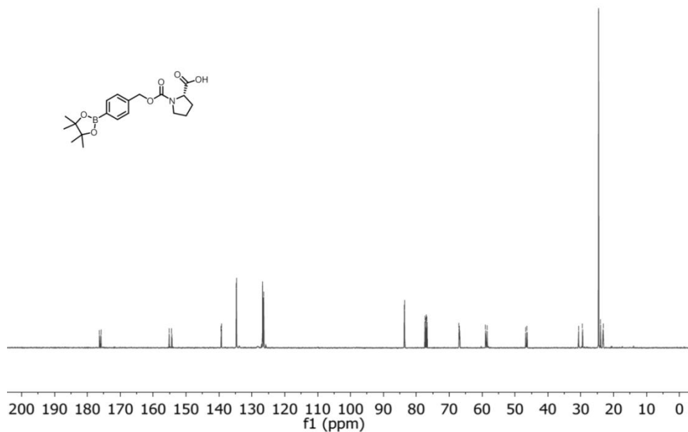
Figure S3.16: 13 C NMR spectrum of boronate-ester derivative in CDCl 3 at 25 °C.
