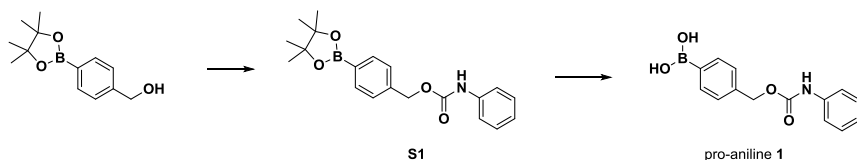
Scheme S2.1: Synthetic route to form pro-aniline 1 .
