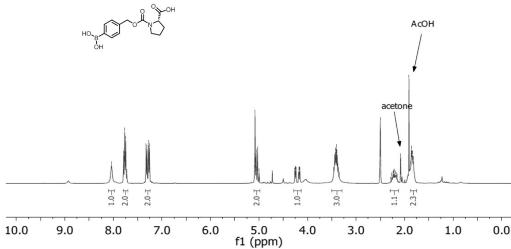
Figure S3.17: 1 H NMR spectrum of PP-1 in DMSO-d 6 at 25 °C.
