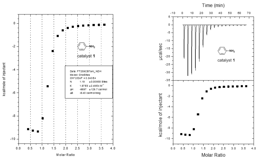
Figure S4.3: ITC measurements for catalyst 1 . Found K_a (1.85 \pm 0.16) \cdot 10^5 \text{ M}^{-1} , error is the standard error of the mean, n = 3 .
