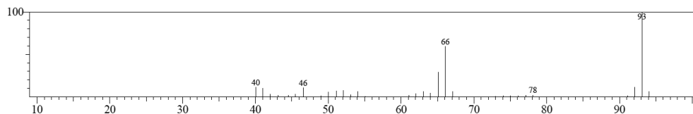
Supplementary Figure S2.4: GC/MS spectrum taken after 65 h of reaction time of hydrazide 3 with aldehyde 4 in the presence of pro-aniline 1 and H 2 O 2 . Conditions: hydrazide 3 (20 mM), aldehyde 4 (20 mM), pro-aniline 1 (10 mM), H 2 O 2 (11 mM) in 20% DMF in 100 mM phosphate buffer pH 7.4. The reaction mixture was extracted after 65 h of reaction time with dichloromethane. The organic layer was evaporated and re-dissolved in ethyl acetate for GC/MS analysis. Aniline 2 was detected in the extract of the reaction mixture, MS (GC/MS) m/z: 93 [M] + •, 66 [C 5 H 6 ] + • (expected m/z = 93.06, 66.05), retention time: 11 min.
