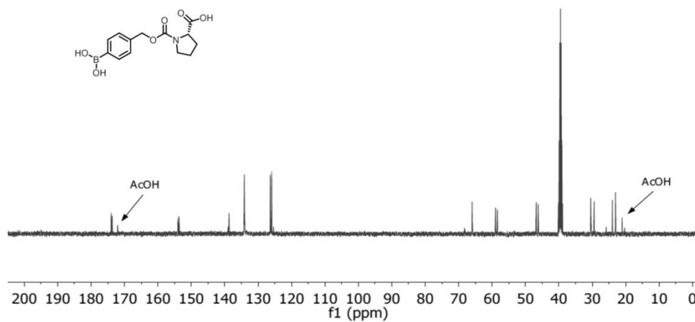
Figure S3.18: 13 C NMR spectrum of PP-1 in DMSO-D 6 at 25 °C.
