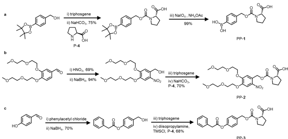
Figure 3.2: Synthetic route to form pro-prolines PP-1, PP-2 and PP-3. (a) Synthesis of PP-1, reaction conditions: i) \text{Na}_2\text{CO}_3 , triphosgene, toluene, 0 °C – room temperature, 6 h. ii) \text{NaHCO}_3 , proline P-4, water, 0 °C – room temperature, overnight, iii) \text{NaIO}_4 , \text{NH}_4\text{OAc} , water / acetone (2:1 v/v). (b) Synthesis of PP-2, reaction conditions: i) \text{HNO}_3 (70% in water), 0 – 20 °C, 2 h, ii) \text{NaBH}_4 , methanol, 1 h, room temperature, iii) \text{K}_2\text{CO}_3 , triphosgene, toluene, 0 °C – room temperature, 6 h, iv) \text{NaHCO}_3 , P-4, water, 0 °C – room temperature, overnight. (c) Synthesis of PP-3, reaction conditions: i) phenylacetyl chloride, triethylamine, tetrahydrofuran, 0 °C – room temperature, overnight, ii) \text{NaBH}_4 , 2-propanol, 1 h, room temperature, iii) \text{K}_2\text{CO}_3 , triphosgene, toluene, 0 °C – room temperature, 6 h, iv) trimethylsilylchloride (TMSCl), diisopropylamine, dichloromethane, 0 °C – room temperature, 4 h.
