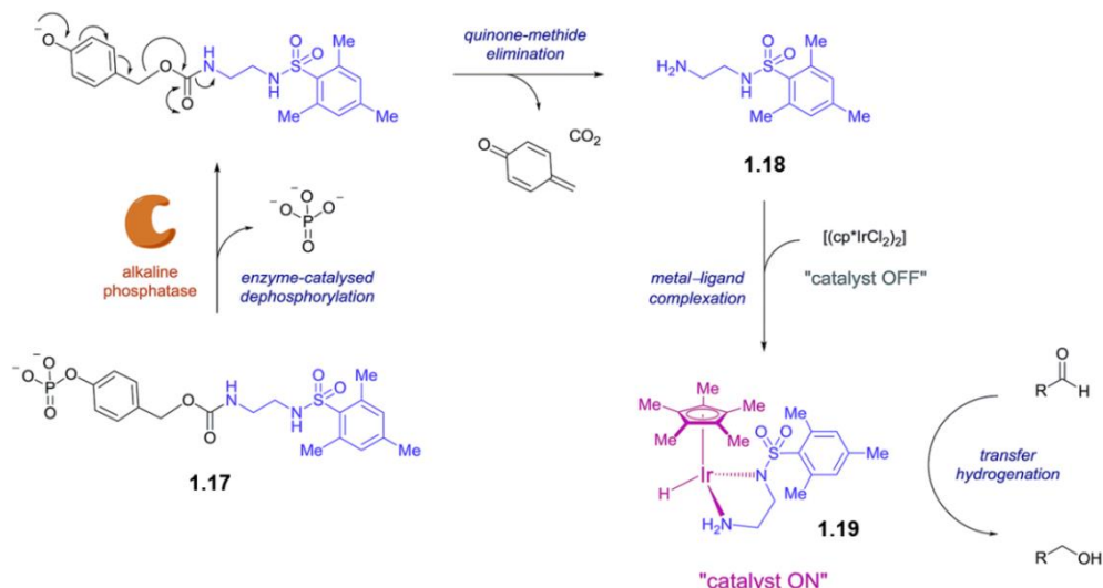
Figure 1.9: Self-immolative chemistry is used to block the binding of a ligand to form an organometallic catalyst for transfer hydrogenation. Enzyme catalysed dephosphorylation induces the self-immolative reaction and release of the ligand which can coordinate to form the active organometallic catalyst. 50 Reprinted from reference 50.
