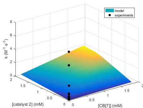
Figure S4.11: Kinetic model defined by eq. 4.1 fits total reaction rate constants for different concentrations of CB[7] and catalyst 2 . (a) 0.42 mM CB[7], 0 – 1.8 mM catalyst 2 , the model fits the experimental values with an R^2 of -0.325. (b) 0.4 mM catalyst 2 , 0 – 0.84 mM CB[7], the model fits the experimental values with an R^2 of 0.300. (c) 0 – 1.8 mM catalyst 2 , 0 – 0.84 mM CB[7].
