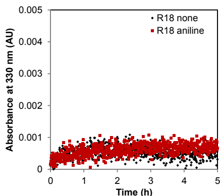
Supplementary Fig. 5.2: Absorbance at rate analysis wavelength of aldehyde and hydrazide mixtures without catalyst (black) and with aniline 1 (red). Reaction conditions: 0.020 mM hydrazide, 0.5 mM aldehyde, 0.5 mM aniline 1 or 0.5 mM 1,3-phenylenediamine · 2 HCl 15 in 20% DMF in 100 mM sodium phosphate buffer pH 7.4. R1 means reaction 1 (etc.) from Table 5.1 in the main text. (a) Reaction 1 between hydrazide 3 and aldehyde 4 , (b) reaction 2 between hydrazide 3 and aldehyde 5 , (c) reaction 3 between hydrazide 3 and aldehyde 6 , (d) reaction 4 between hydrazide 7 and aldehyde 8 , (e) reaction 5 between hydrazide 7 and aldehyde 5 , (f) reaction 6 between hydrazide 7 and aldehyde 9 , (g) reaction 7 between hydrazide 7 and aldehyde 10 , (h) reaction 8 between hydrazide 11 and aldehyde 4 , (i) reaction 9 between hydrazide 11 and aldehyde 5 , (j) reaction 10 between hydrazide 12 and aldehyde 4 does not take place, (k) reaction 11 between hydrazide 13 and aldehyde 4 , (l) reaction 12 between hydrazide 14 and aldehyde 4 , (m) reaction 13 between hydrazide 14 and aldehyde 5 , (m) reaction 13 between hydrazide 14 and aldehyde 5 , (n) reaction 14 between hydrazide 11 and aldehyde 16 does not take place, (o) reaction 15 between hydrazide 11 and aldehyde 8 , (p) reaction 16 between hydrazide 14 and aldehyde 16 does not take place, (q) reaction 17 between hydrazide 14 and aldehyde 8 , (r) reaction 18 between hydrazide 14 and benzaldehyde 8 does not take place.
