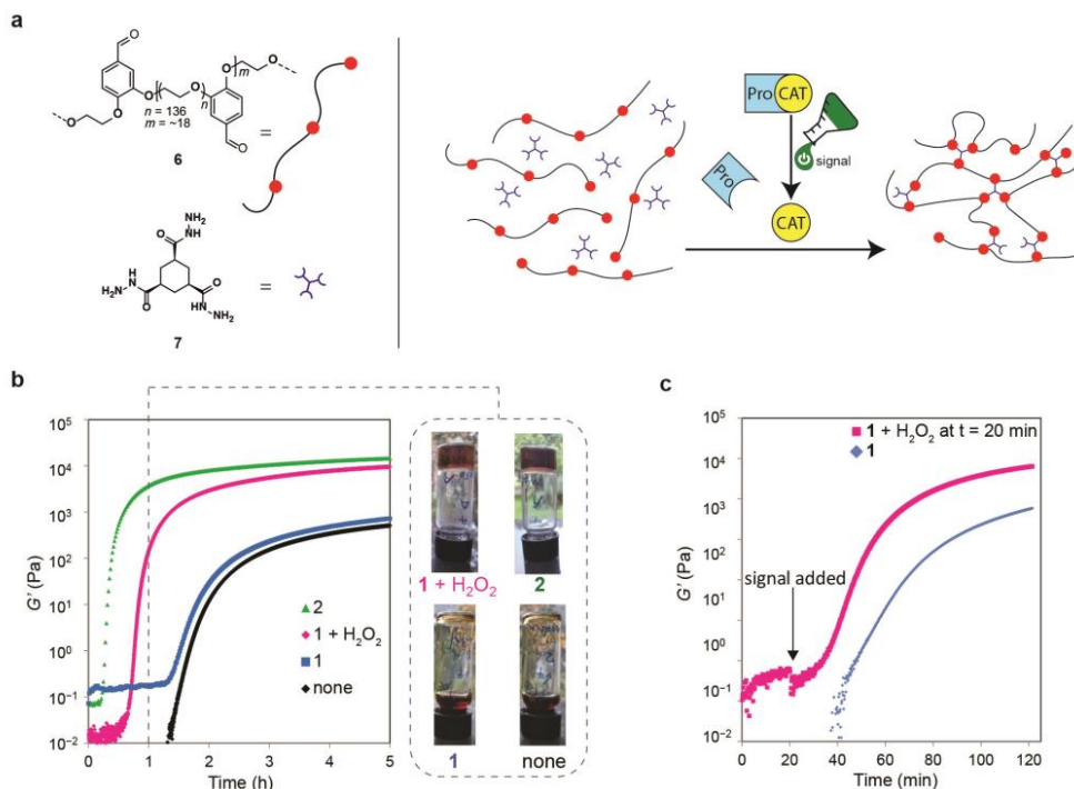
Figure 2.3: Polymer gel formation controlled by the activation of pro-aniline 1 . (a) The formation of a hydrazone polymer gel: aldehyde 6 and hydrazide 7 react to form a cross-linked hydrazone polymer gel. (b) The storage modulus G' measured with oscillatory rheology during gel formation at 25 °C (10 mM hydrazide 7 , 136 mg mL -1 aldehyde 6 in 20% dimethylformamide (DMF) in 100 mM phosphate buffer, pH 6.0) for the uncatalyzed gel (black line), the gel with 10 mM pro-aniline 1 (blue line), the gel with 10 mM pro-aniline 1 and 10 equivalents H_2O_2 (magenta line) and the gel with 10 mM aniline 2 (green line). The gelation rate with activated pro-aniline 1 is comparable to the gelation rate with aniline 2 . Without activation of the pro-aniline 1 , the gelation rate is comparable to the gelation rate of the uncatalyzed reaction. After 1 hour of gelation time, the mixtures with aniline 2 or activated pro-aniline 1 have gelled, whereas the mixtures without catalyst or with unactivated pro-aniline 1 have not gelled yet. We performed the gelation experiment in vials using the same conditions as we used for rheology and took a photograph after 1 hour of reaction time. Top left: pro-aniline 1 (10 mM) and H_2O_2 (100 mM), top right: aniline 2 (10 mM), bottom left: pro-aniline 1 (10 mM) and bottom right: without catalyst. (c) The gelation rate can be controlled during the process by adding a chemical signal (here after 20 minutes), liberating the catalyst. The storage modulus G' measured with oscillatory rheology for the aldehyde 6 /hydrazide 7 (10 mM) mixture with 10 mM pro-aniline 1 (blue line) and the mixture with pro-aniline 1 when 10 equivalents of H_2O_2 was added after 20 min (magenta line). Addition of the chemical signal induces a significant increase in gelation rate.
