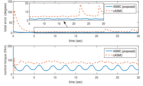
Figure 2. Tracking performance comparison between ASMC (proposed) and c\text{ASMC} .
