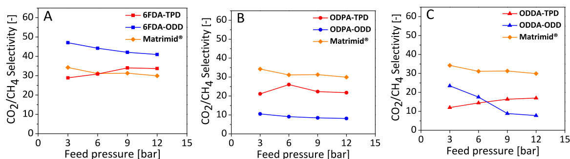
Fig. 6. CO 2 /CH 4 selectivity as function of feed pressure. (A) 6FDA-series, (B) ODPA-series and (C) ODDA-based membrane series. Matrimid® is included for reference purposes. Feed mixed gas: CO 2 /CH 4 (50/50 vol%).
