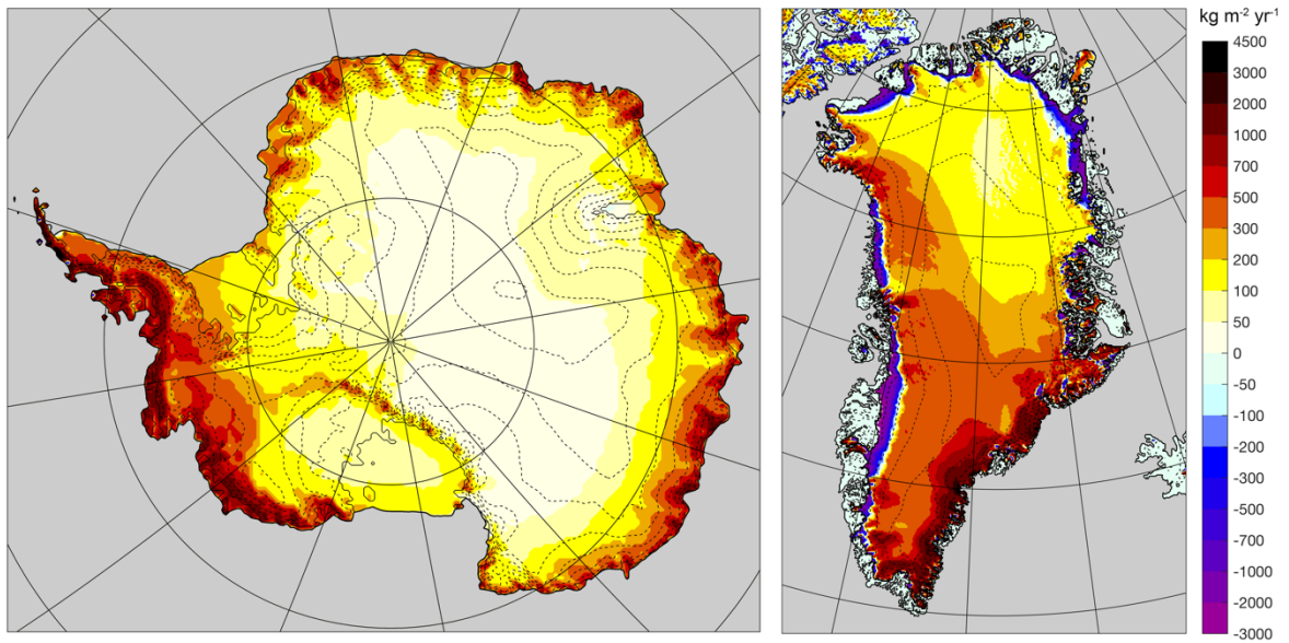
Figure 2. Surface mass balance (averaged over the period 1989-2009) of the Antarctic ice sheets (left) and the Greenland Ice Sheet (right) from the regional climate model RACMO2.3p2 in \text{kg m}^{-2} \text{yr}^{-1} (van Wessem et al., 2018; Noël et al., 2018a). Elevation contour levels (dashed) are shown every 500 m.
