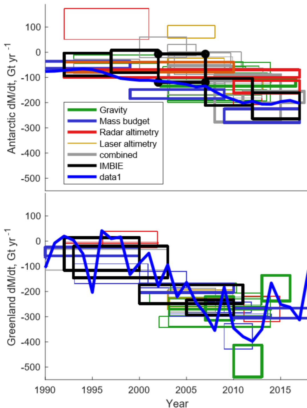
Figure 3. Mass rates for the Antarctic (top) and Greenland (bottom) ice sheets derived from published studies. The horizontal extent of each rectangle indicates the period that each estimate spans, while the height indicates the error estimate. Studies published between 2011 and 2017 are shown with thin lines, studies published in 2018 and early 2019 with heavier lines. The colour of the lines indicates the type of estimate used, and any estimate that is based explicitly on more than one technique is treated as a ‘combined’ estimate. The IMBIE (Shepherd et. al, 2012 for Greenland, Shepherd et al., 2018 for Antarctica) estimates are shown in black. Rectangles are overplotted with annual mass balance estimates from Rignot et al. (2019) for Antarctica and Mouginot et al. (2019) for Greenland, to indicate interannual variability. The studies cited in this plot are described in Supplemental Table I.
