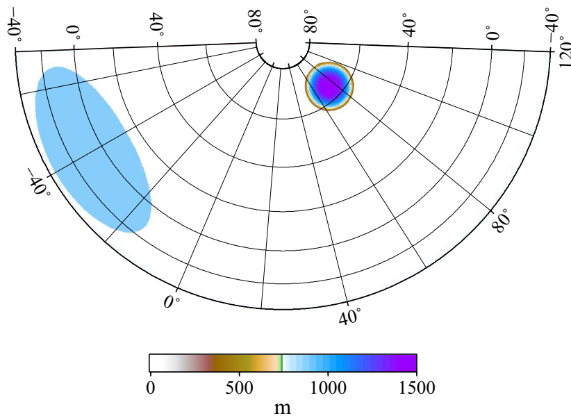
Figure 4. Height of the grounded ice at t = 10 kyr in benchmark B computed by VEGA ref . The grounded ice does not reach the ocean basin during the loading period. The light blue ellipse shows the circular ocean function, which is fixed throughout time.
