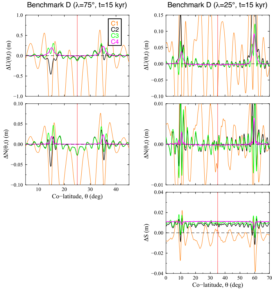
Figure A1. The differences arising from the \text{VEGA}^{\text{Ci}} solutions, i = 1, \dots, 4 , with respect to \text{VEGA}^{\text{ref}} along the co-latitudinal cross-sections shown in the right panels of Figs 14 (left) and 15 (right) for benchmark D. The four combinations C1,...,C4 of the input parameters for the \text{VEGA}^{\text{Ci}} solutions are given in Table A1.
