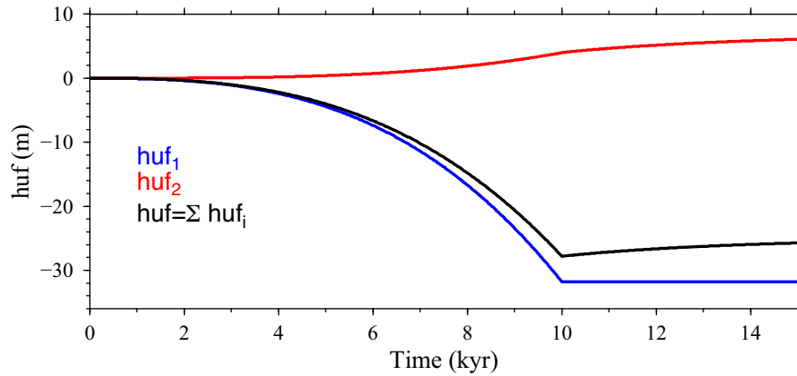
Figure 11. Time evolution of the thickness of the uniform water layer, h_{UF}(t) , for benchmark C computed by VEGA^{ref} . The blue and red curves stand for two terms on the right-hand side of eq. (12), while the sum of them is shown by the black curve.
