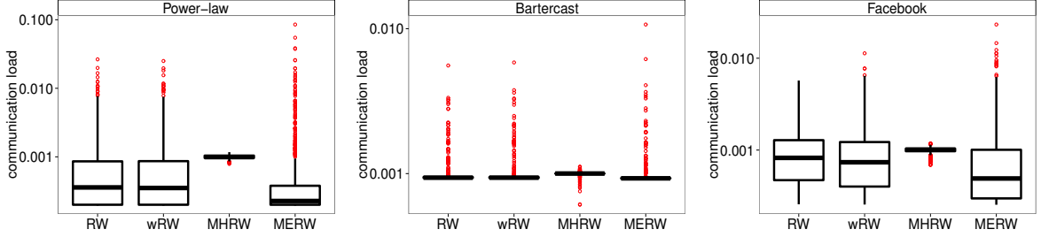
Figure 7: Scalability: the distribution of the communication load of nodes for the different random walks in the power-law, Bartercast, and Facebook graphs.
