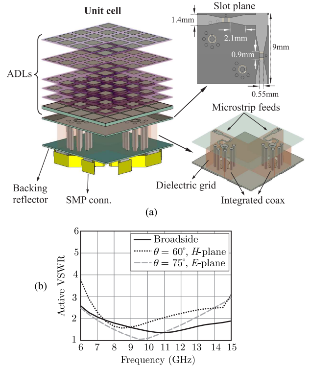
Fig. 3. (a) Three-dimensional view of the final unit cell and (b) active VSWR for broadside and scanning to 60^\circ in the H -plane and to 75^\circ in the E -plane.
