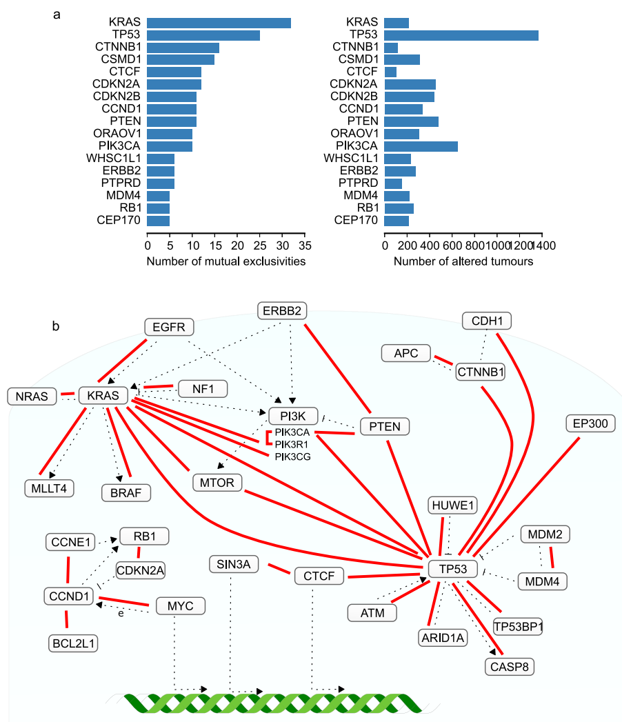
Fig. 4 Overview of detected pairwise mutual exclusivities. a Comparison of the number of significant mutual exclusivities found for a gene and the number of tumors in which it has been altered. b Mutual exclusivities that overlap with high-confidence interactions in the STRING functional interaction network depicted in their biological context. Red lines represent a mutual exclusivity between the connected genes. Dotted lines depict a functional interaction
