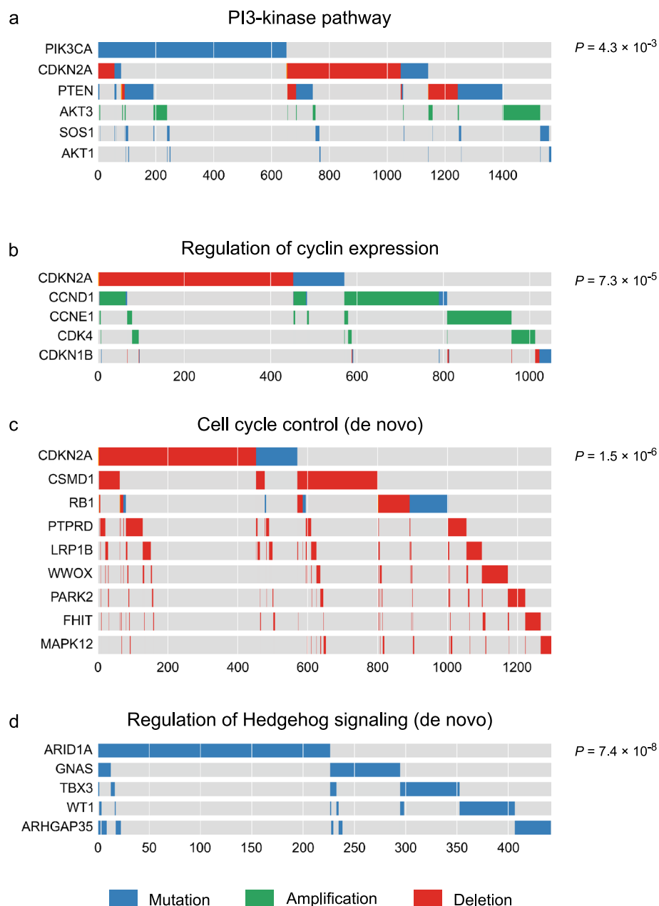
Fig. 5 Examples of gene sets with mutually exclusive alterations. The P values were computed using DISCOVER's group-based test. Panels a and b show predefined gene sets extracted from MSigDB. Panels c and d show gene sets identified using our de novo group detection approach
