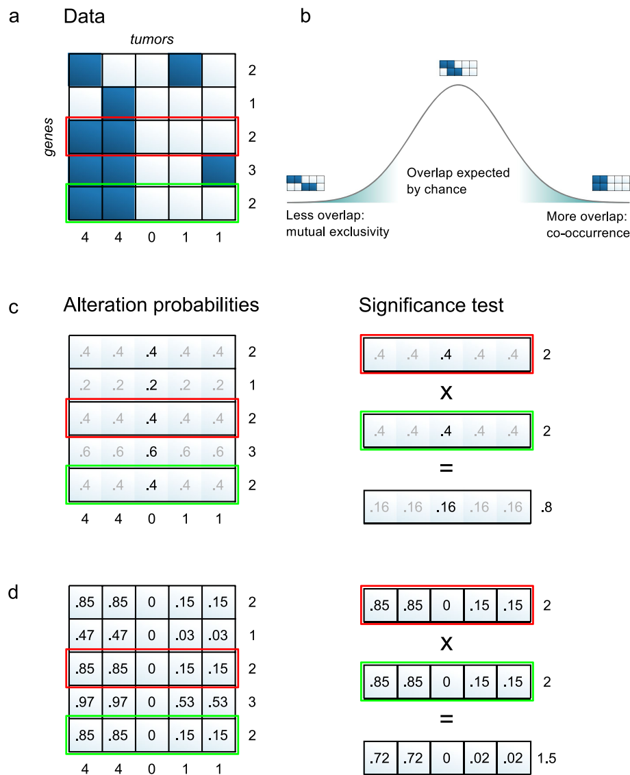
Fig. 1 Overview of the DISCOVER method. a The input to the method is a binary alteration matrix with genes in the rows and tumors in the columns. The following panels illustrate how the two genes highlighted in red and green are tested for co-occurrence. b To identify co-occurrences or mutual exclusivities, a null distribution is estimated that describes the overlap in alterations of two genes expected by chance. Co-occurrence and mutual exclusivity correspond to the tails of this distribution. c In the binomial model, a single alteration probability is estimated per gene that applies to all tumors. The expected number of alterations per gene matches the observed number. The expected number of alterations per tumor does not match the observed number. The product of two genes' alteration probabilities gives the probability of overlap by chance, which multiplied by the number of tumors gives the expected number of tumors with alterations in both genes, in this case 0.8. d In the Poisson-binomial model, gene alteration probabilities are estimated for each tumor individually. The expected number of alterations both per gene and per tumor match the observed numbers. The product of two gene alteration probabilities is also computed per tumor. The expected number of tumors with alterations in both genes according to this model is 1.5
