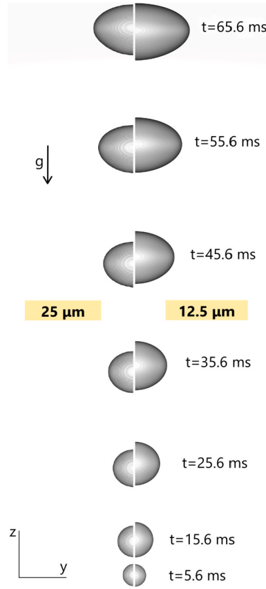
Fig. 15. Temporal evolution of the ethanol bubble shape as it rises due to buoyancy. The results obtained with a grid spacing of 25\ \mu\text{m} (left) and 12.5\ \mu\text{m} (right) are compared. The interface location is visualized by the iso-surface with C = 0.5 .
