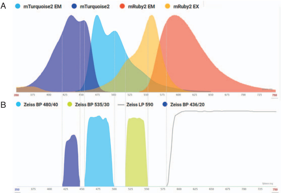
Figure S5.2. Spectral overview of (A) fluorophores and (B) filters used for in vivo co-localization assays. The x-axes display wavelength in nanometers, the spectral plot is generated using FPBase.
