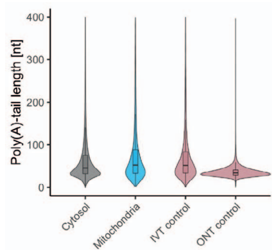
Figure S3.3. Estimated Poly(A)-tail lengths after enzymatic polyadenylation. The length of the poly(A)-tail was estimated by Nanopolish-PolyA on the obtained RNAseq data for RNA of mitochondrial (no native poly(A) tail) and cytosolic origin (natively poly(A)-tailed) and of in vitro -synthesized control RNA (no native poly(A)-tail). The length of the poly(A)-tail of the ONT control RNA (not enzymatically polyadenylated, contains poly(A)-tail) was determined as a control. Distribution of poly(A)-tail lengths is shown as violin plots, the mean is shown as a box plot where the outer ends of the box represent the 25 th and 75 th percentile of the data.
