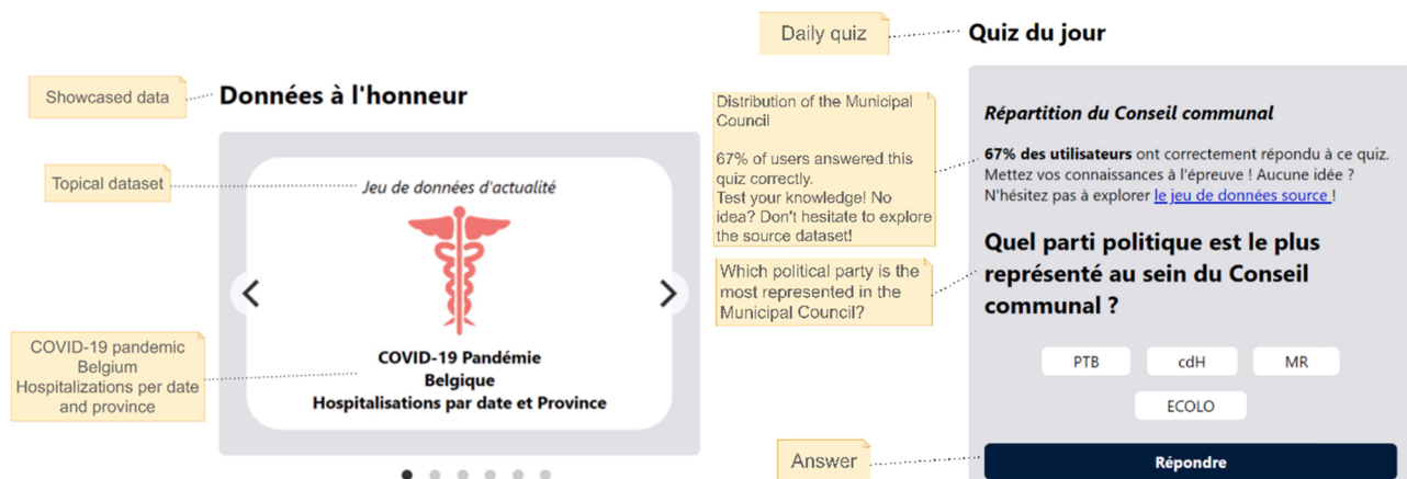
Fig. 4. Highlighted Datasets (DP6) (Left) and Data Quiz (DP1, DP10) (Right).
