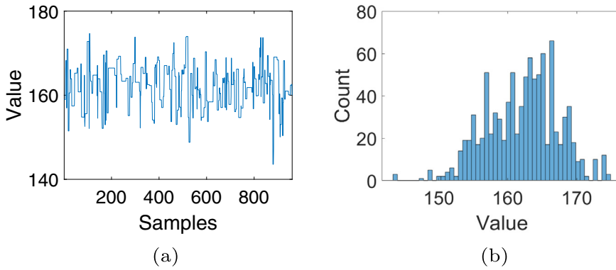
Fig. 5. The resulting trace plot (a) and histogram (b) obtained from MH sampling of 1000 samples after discarding the initial N_{\text{burn-in}} = 40 samples.
