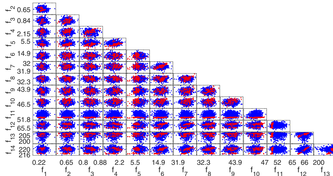
Fig. 33. The scatterplot matrix illustrating the updated model output profile obtained using TCMC. The blue scatter plots represent the frequency output from the updated model while the red scatter plots represent the experimental frequency measurements. (For interpretation of the references to color in this figure legend, the reader is referred to the web version of this article.)
