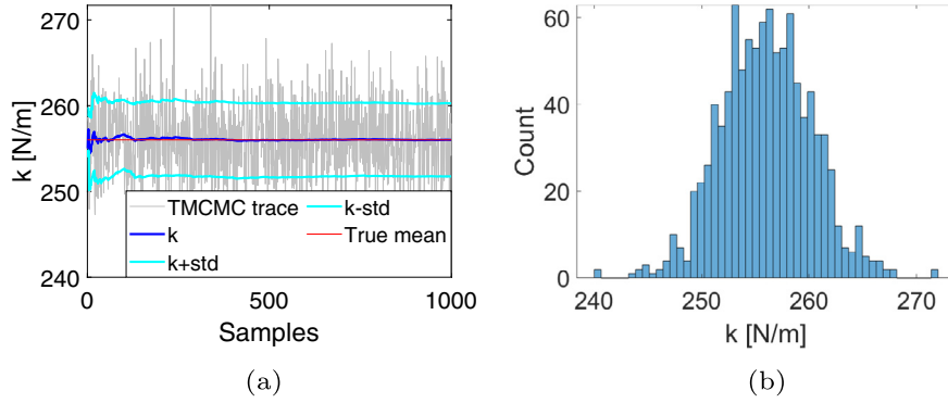
Fig. 15. The resulting time-series sample plot (a) and the histogram (b) obtained using TCMC sampler with sample size 1000. The red line in the time-series sample plot denotes the true sample mean value. (For interpretation of the references to color in this figure legend, the reader is referred to the web version of this article.)
