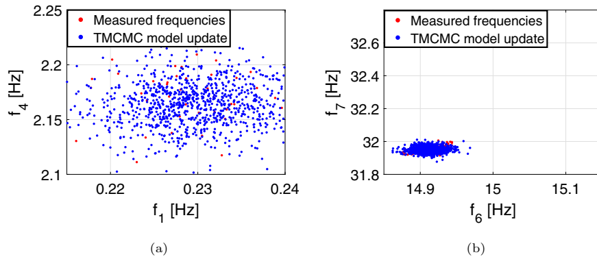
Fig. 29. Comparison between the scatter plot obtained from experimental frequency data and that of from the updated ANN surrogate model via TCMC sampler. Subplot (a) presents the comparison between frequencies f_1 and f_4 , while subplot (b) presents the comparison between frequencies f_6 and f_7 .
