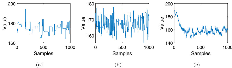
Fig. 3. The corresponding trace plots obtained with 1000 samples using: (a) \sigma_p = 100.5 giving an acceptance level of 0.061; (b) \sigma_p = 22.5 giving an acceptance level of 0.234; (c) \sigma_p = 1.5 giving an acceptance level of 0.865.
