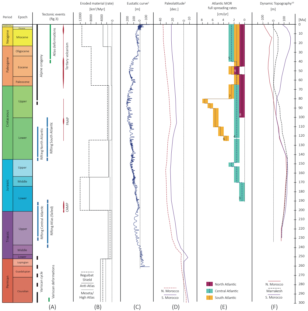
Figure 6.8. Permian to Neogene evolution of A) major tectonic events in the Atlantic realm and Morocco (see references in chapter 1); B) volumes of eroded material per million year for the Meseta/High Atlas, Anti-Atlas, and Reguibat Shield (chapter 4); C) see level 1 Snedden and Liu, 2010); D) paleo-latitude of two points in Morocco (after maps of 2 Scotese, 2012); E) Full Mid Oceanic Ridge (MOR) spreading rates (after 3 Labails et al., 2010; 4 Müller et al., 2008; 5 Schettino et al., 2016; 6 Granot and Dymont, 2015; 7 Nurnberg and Müller, 1991; 8 Mosar et al., 2002; 9 Torsvik et al., 2001); F) and dynamic topography of three points in Morocco (from the GPlates website, after model CIs of 10 Barnett-Moore et al., 2017)
