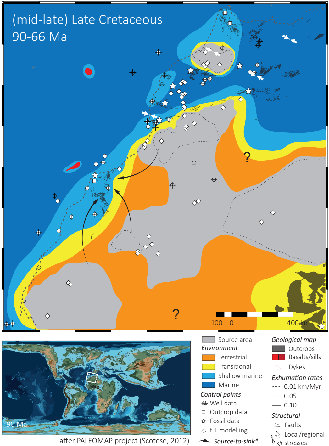
Figure 5.9. (mid-late) Late Cretaceous map. * Simplified source-to-sink systems evidenced with provenance study or paleo-currents.
