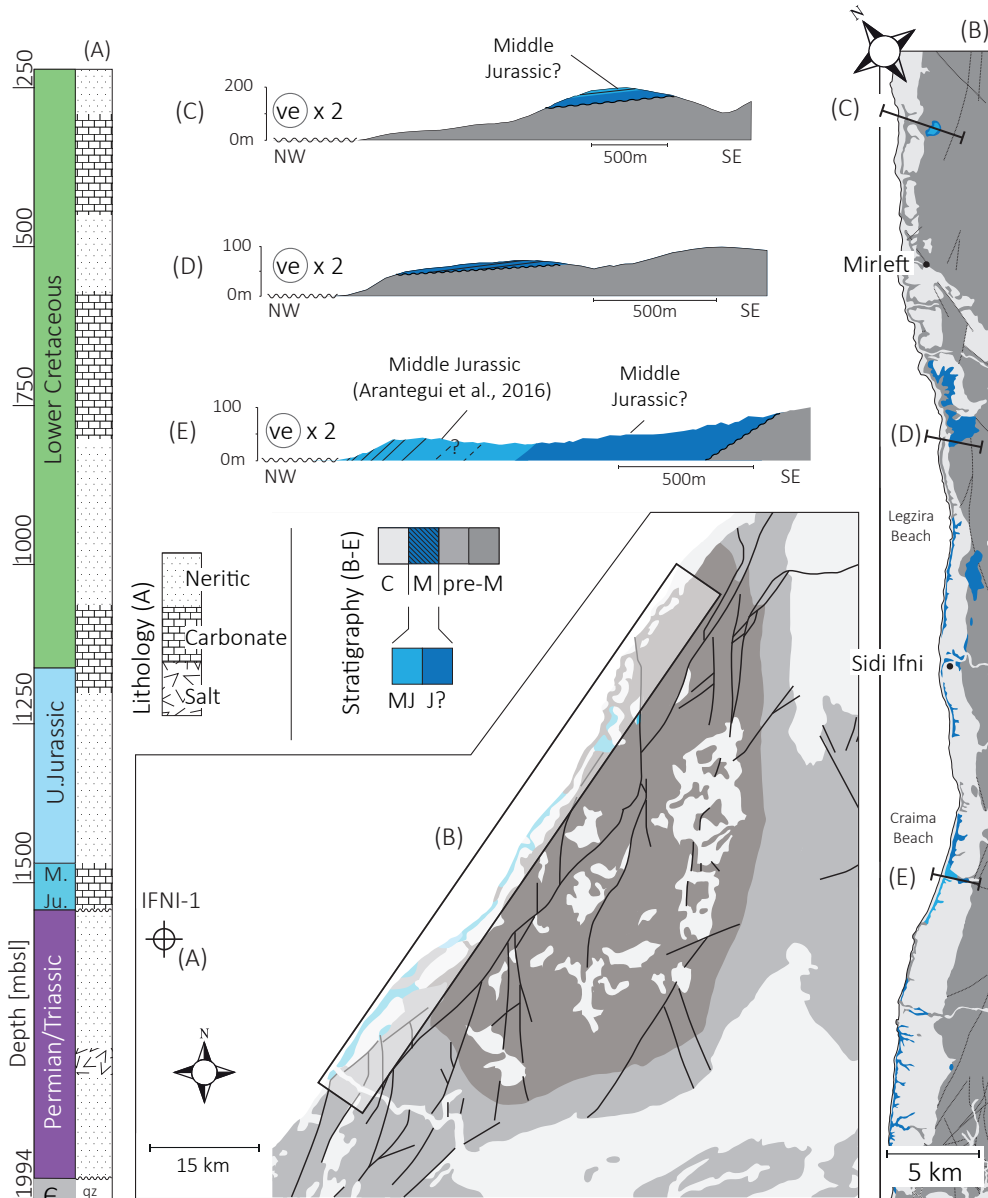
Figure 2.2. A) Stratigraphic log of the Ifni-1 (IF-1) well (after well report). Neritic : Neritic clastics and sandstones (continental for the Triassic), Carbonate : Limestones/dolomites, Salt : Salt and other evaporites. B) Simplified geological map of the Sidi Ifni Margin with highlight on Mesozoic sediments (after 1/100000 geological maps of Tiznit and Sidi Ifni; Yazidi et al., 1986; 1991). J? : Middle? Jurassic fluvial red conglomerates and red/pink/grey coarse to very coarse sandstones; MJ : Intertidal fine clastics and shallow marine carbonates identified as Middle Jurassic (Arantegui et al., 2016; Arantegui, 2018). C-E) Cross-sections illustrating the geometry of the contact between the Sidi Ifni basement rocks and the Mesozoic sediments (based on field work and Google Earth investigations).
