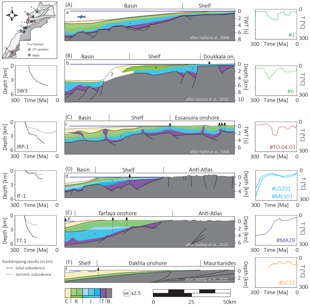
Figure 6.6. Present-day 2D architecture of the Moroccan passive margin (central panels), selected subsidence and backstripping curves (left panels), and t-T modelling (right panels) results. A to F) Rabat, Doukkala, Essaouira, Sidi-Ifni, North Tarfaya, and Dakhla transects, respectively. Note that cross-sections 'a' and 'c' are in time. See location map for orientation. C: Cenozoic; K: Cretaceous; J: Jurassic; T: Triassic; B: Basement (Palaeozoic and Precambrian). The letters "J" and "K" are shown on the sections only if the Jurassic or Cretaceous are locally undifferentiated. The t-T best-fit results of samples 1/6, TO.04.01 and MA29 are from Ghorbal et al., 2008, Ghorbal, 2009 and Sehr et al., 2017a, respectively. The t-T weighted average results of samples LGZ01/MES01 and SC12 are from the present work and Leprêtre et al., 2015, respectively. The subsidence curves from wells SW3 (synthetic), JRP-1 and IF-1/TT-1 are from Gouiza et al., 2010, Bouatmani et al., 2007 and Gouiza, 2011, respectively.
