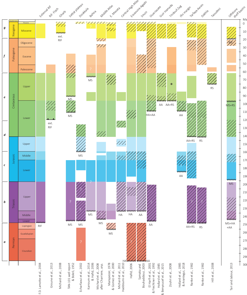
Figure 4.7. Simplified stratigraphic columns. The hatched parts highlight continental facies and/or coarse to very coarse deposits. Below unconformity surfaces are the name of the corresponding Variscan/Precambrian basement (MS: Meseta, HA: High Atlas, AA: Anti-Atlas, and RS: Reguibat shield basements). The seven selected periods (a to g) are shown on the left. *Late Cretaceous in the Tindouf basin is present in the eastern and western parts, but not in its central part (Hollard et al., 1985).
