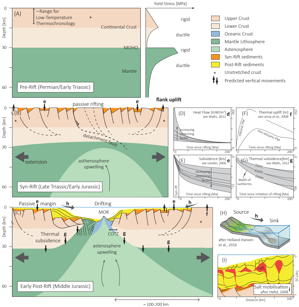
Figure 6.1. Summary of the vertical movements expected in the Central Atlantic margins and their adjacent continental crusts (after Gouiza et al., 2010). A), B), and C) Pre-, Syn- and post-rift situations, respectively. MOR : Mid-Oceanic Ridge (spreading centre); COTZ : Continent-Ocean Transition Zone. D), E), F), and G) Evolution of different aspects of a rifted continental margin. H) and I) Cartoons illustrating source-to-sink systems and salt mobilisation, respectively.
