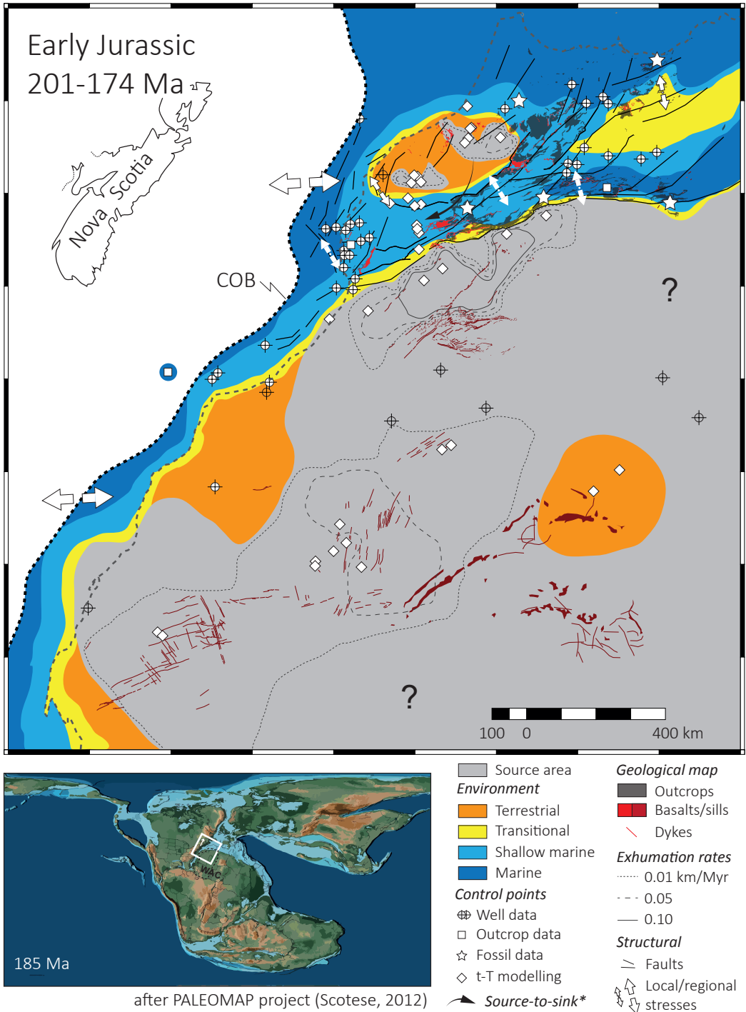
Figure 5.4. Early Jurassic map. * Simplified source-to-sink systems evidenced with provenance study or paleo-currents. CAMP : Central Atlantic Magmatic province.
