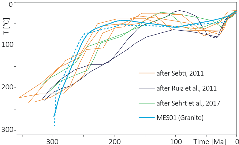
Figure 2.6. Best-fit (dashed) and weighted average t-T paths of MES01 compared to the best-fit t-T paths obtained in previous studies for samples of the Precambrian basement of the Sidi Ifni area.
