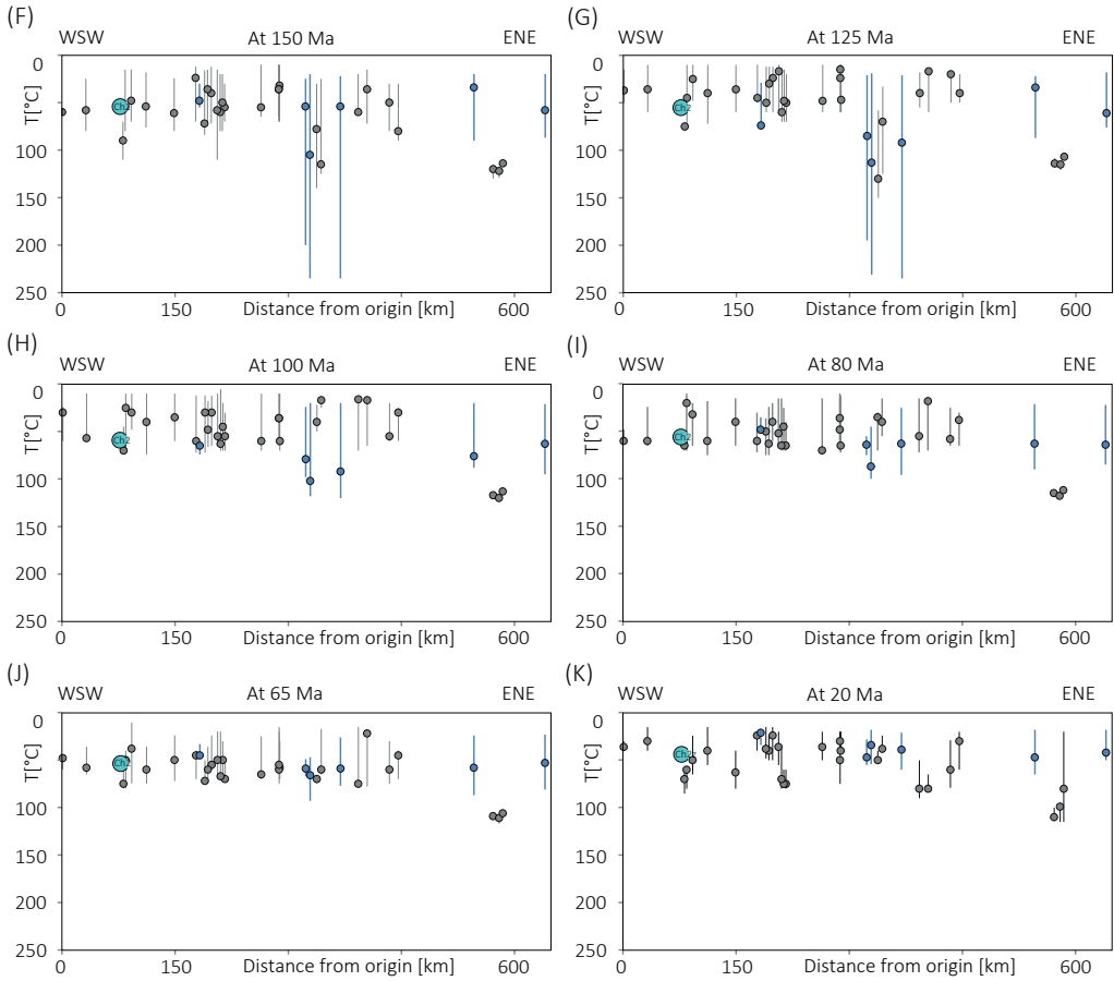
Figure 3.12. (continued) We assume that the post-Variscan exhumation of the Anti-Atlas has only a vertical component (no horizontal), meaning that the relative position of the samples remained similar within the Moroccan margin. Ch2: Temperature of the 'best-fit model of the Sidi Ifni granite (chapter 2).*
