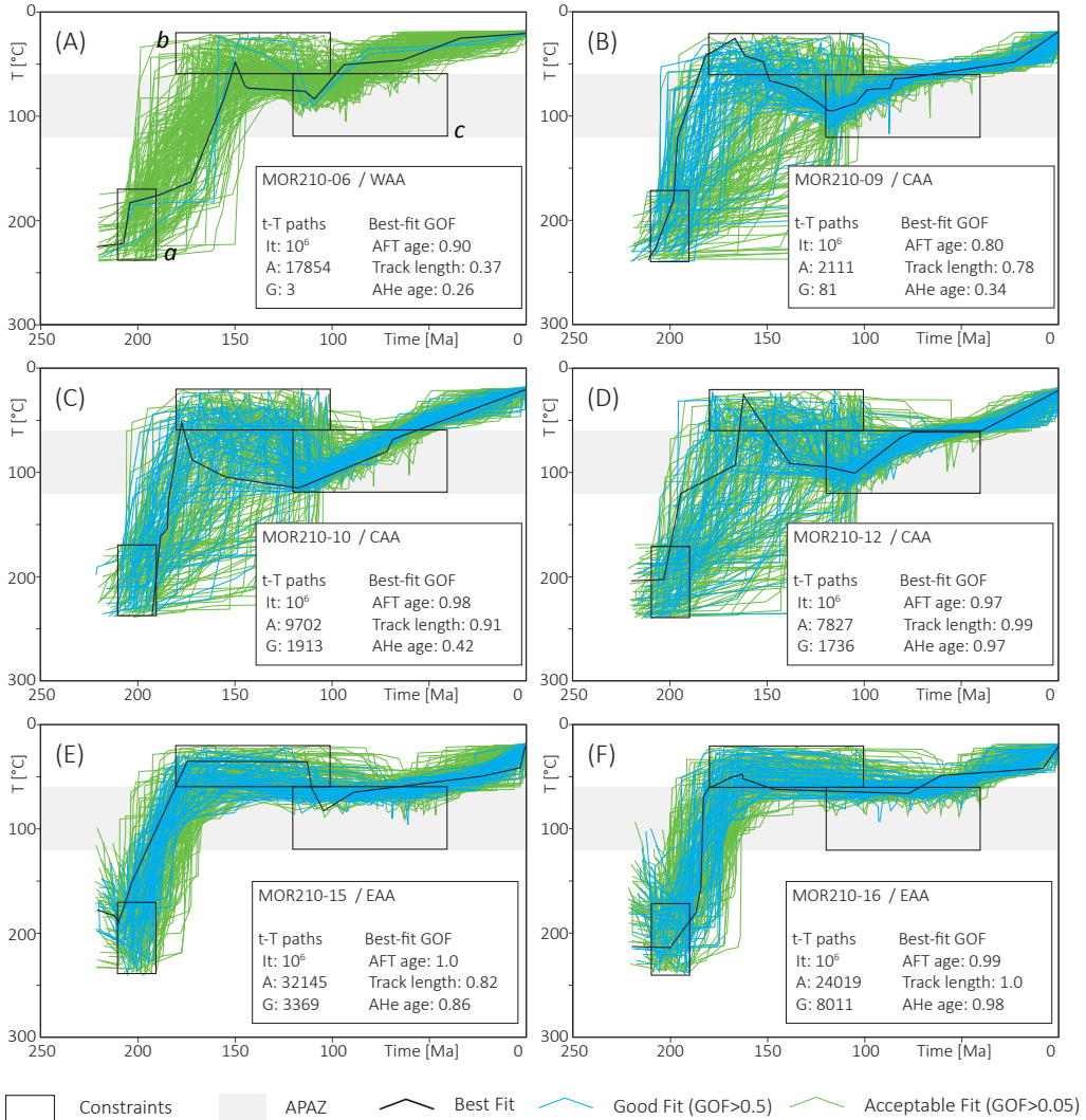
Figure 3.9. Results of thermal history modelling for samples from the Anti-Atlas granitic basement; WAA , CAA , and EAA : Western, Central, and Eastern Anti-Atlas, respectively. 50 good (when possible), 150 acceptable, and the best-fit (highest Goodness of Fit; GOF) t-T curves are displayed. See parameters in table 3.4. It : Number of iteration for the inverse modelling; A : Acceptable paths; G : Good paths.*
