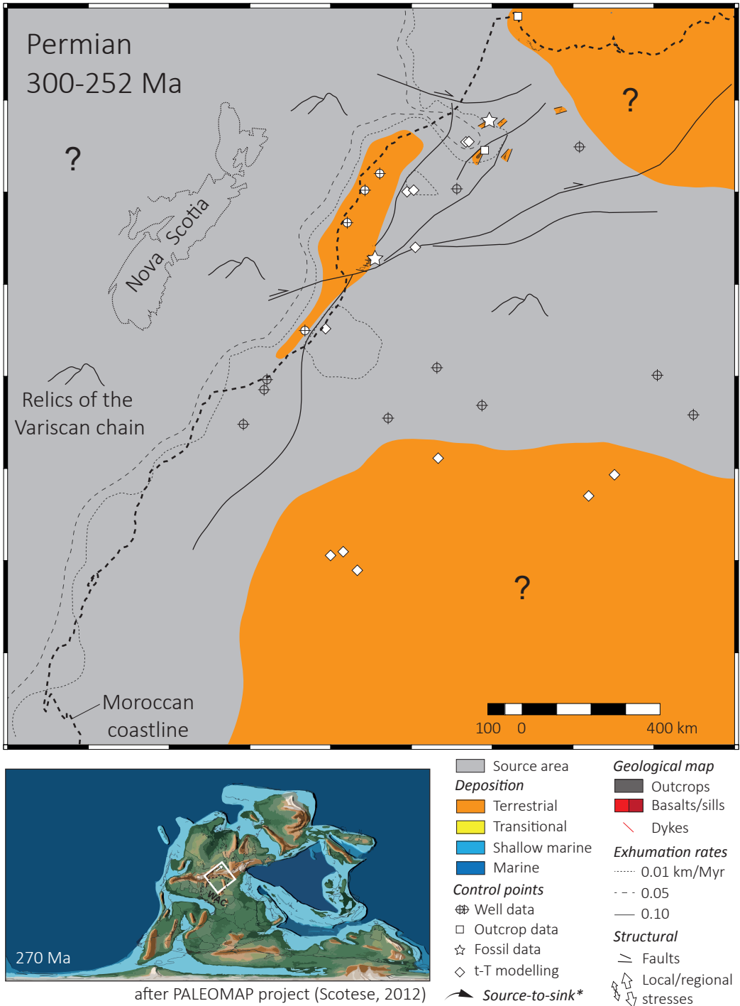
Figure 5.2. Permian map. * Simplified source-to-sink systems evidenced with provenance study or paleo-currents. WAC : Western African Craton
