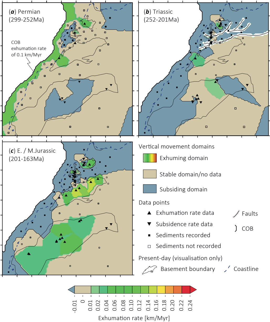
Figure 4.8. Exhumation maps for the seven selected periods (a-c on this page and d-g on the next one) after geological record (fig. 4.7) and vertical movement rates (fig. 4.5). We define three domains in the exhumation maps: a subsiding domain with rates \leq -0.011 km/Myr, a stable domain characterised by rates between -0.01 and 0.01 , and an exhuming domain with rates \geq 0.011 km/Myr. Note that the western boundary is the Continent-Ocean Boundary (COB).
