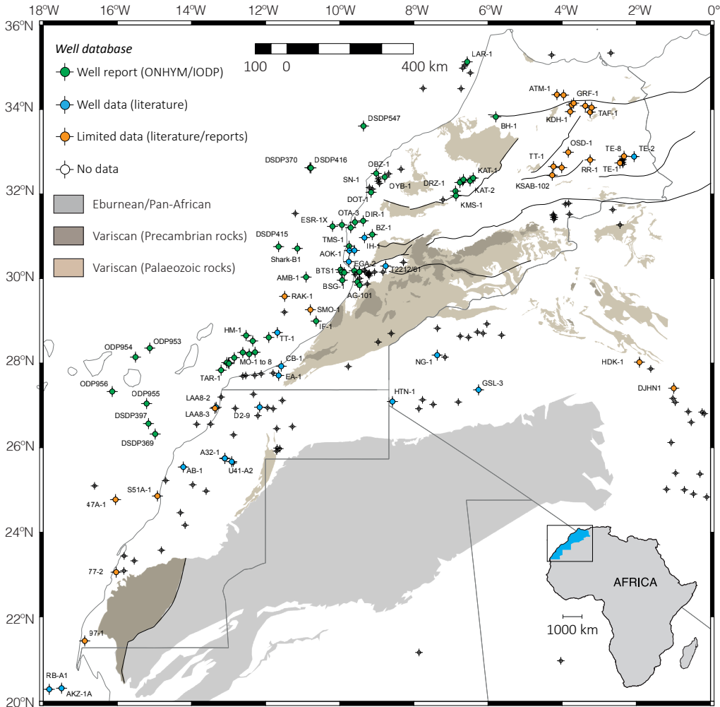
Figure 5.1. Location of boreholes in Morocco and surrounding NW African countries (non-exhaustive). *
