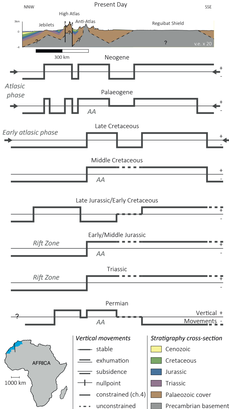
Figure 6.7. Highly schematic NNW-SSE evolution of vertical movements as evidenced by LTT and t-T modelling (see chapter 4).
