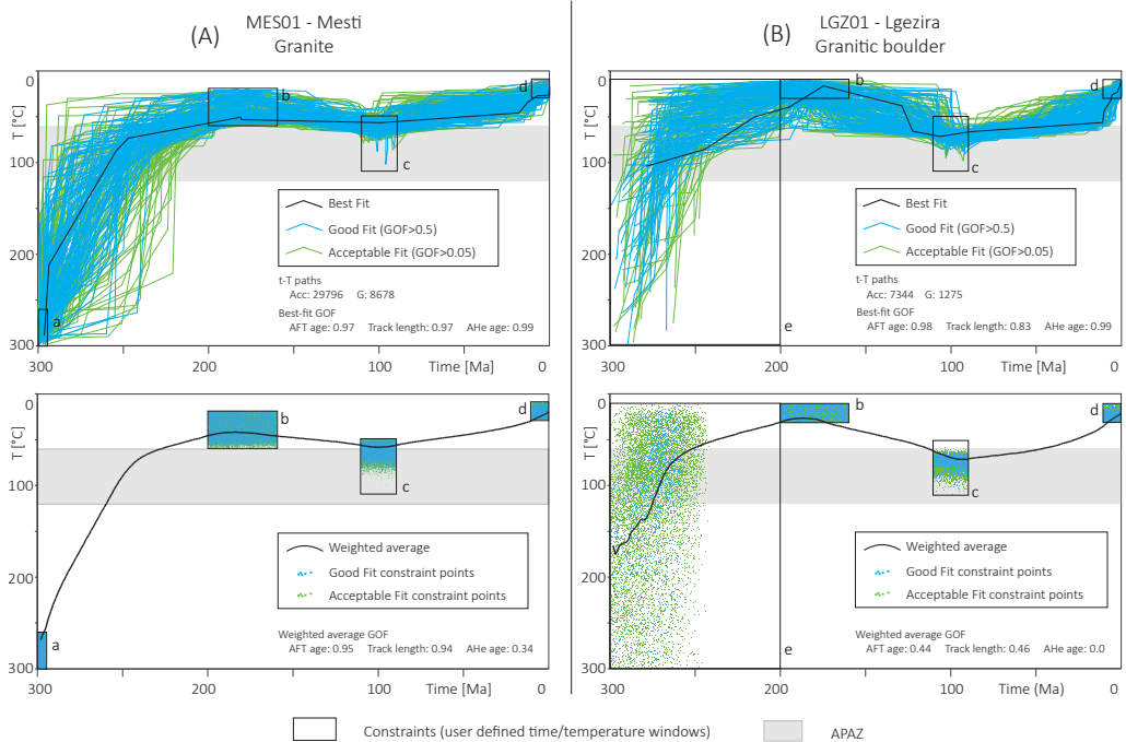
Figure 2.5. Results of t-T modelling for A) MES01 and B) LGZ01. Results are displayed with up to 200 curves for both good and acceptable goodness of fit (GOF) and the best-fit t-T path (upper panels) or with the constraint points and the weighted average (lower panels). Forward modelling was used to reproduce the weighted average curves in order to obtain their GOF values. See modelling parameters in table 2.3. Acc : Acceptable paths; G : Good paths. APAZ : Apatite Partial Annealing Zone.
