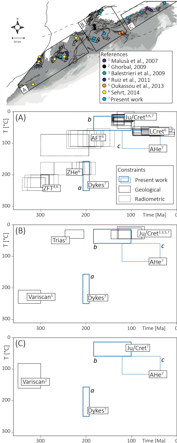
Figure 3.8. Constraints used in t-T modelling from literature (see references in the figure) and from our modelling (blue constraints). A), B), and C) Western, central, and eastern Anti-Atlas, respectively. Variscan: Compression, metamorphism and the load of Palaeozoic sediments; Ju/Cret: Presence close to the surface of the sampled basement rocks during the Late Jurassic to the Early Cretaceous; LCret: Late Cretaceous to Palaeogene overburden in the western Anti-Atlas; Trias: Presence at/close to the surface of the basement rocks in the Siroua during the Triassic; Dykes: See text.
