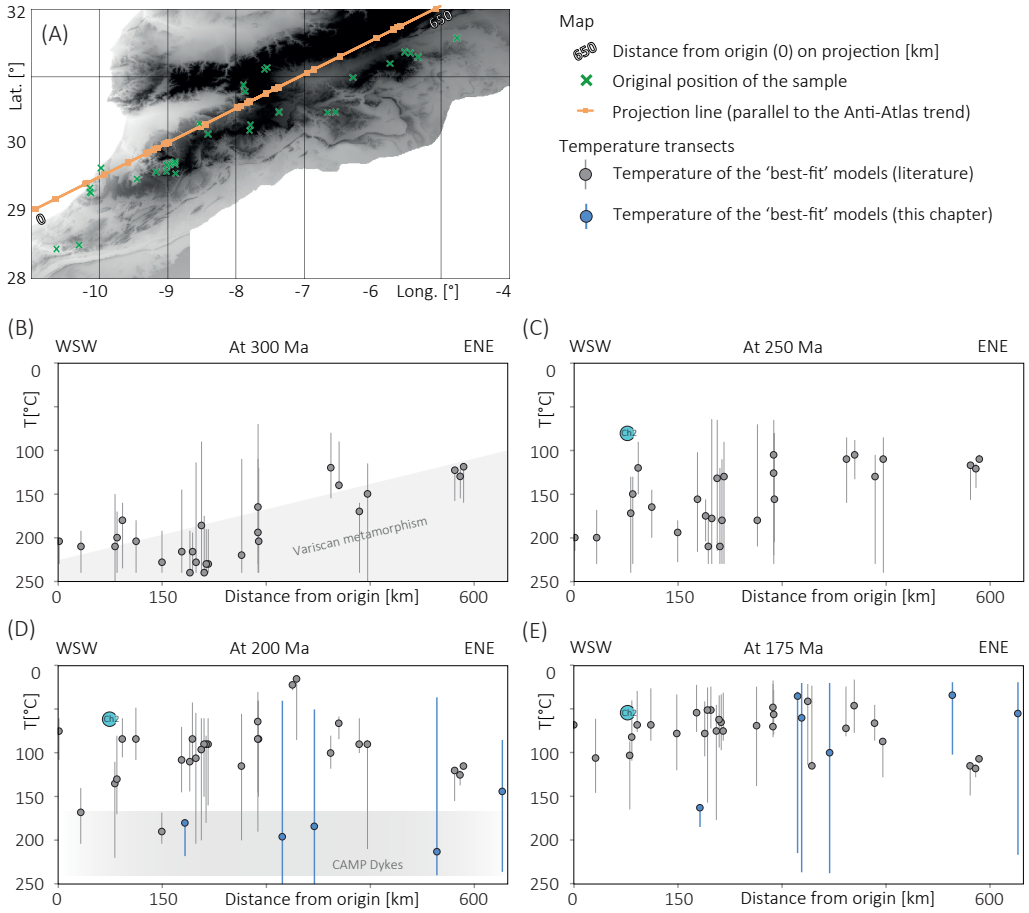
Figure 3.12. Palaeo-temperature transects of the presently outcropping rocks from the Precambrian Anti-Atlas. A) DEM (SRTM 90m, NASA) map with the projection line; B-K) 300-20 Ma temperature transects. The error bars were provided by the envelopes of the realisations with a good GOF.
