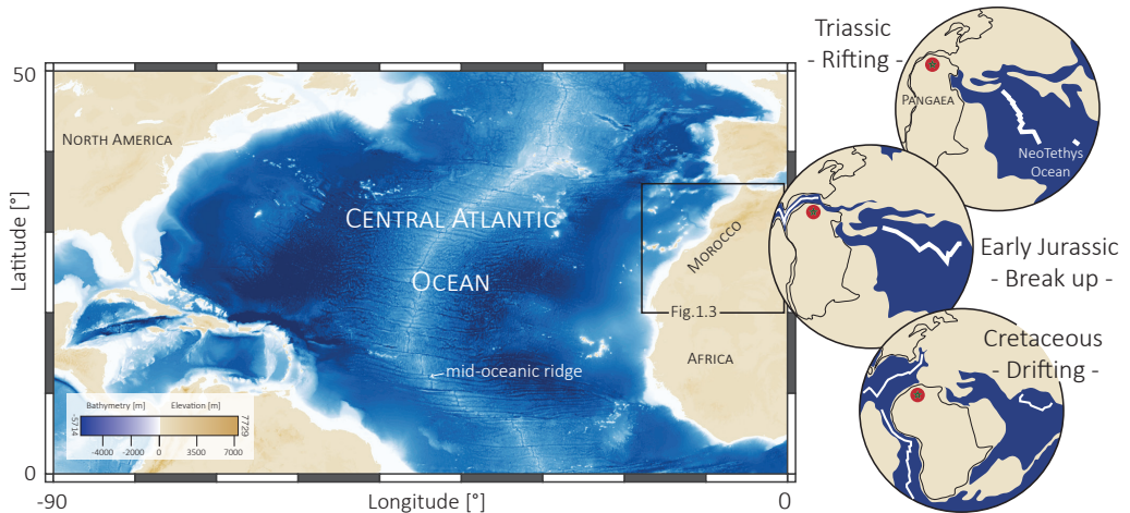
Figure 1.1. Morphology of the Central Atlantic seafloor and conjugate margins (data: GEBCO_2014_1D). The simplified plate tectonic evolution is after Stampfli and Borel (2002).
