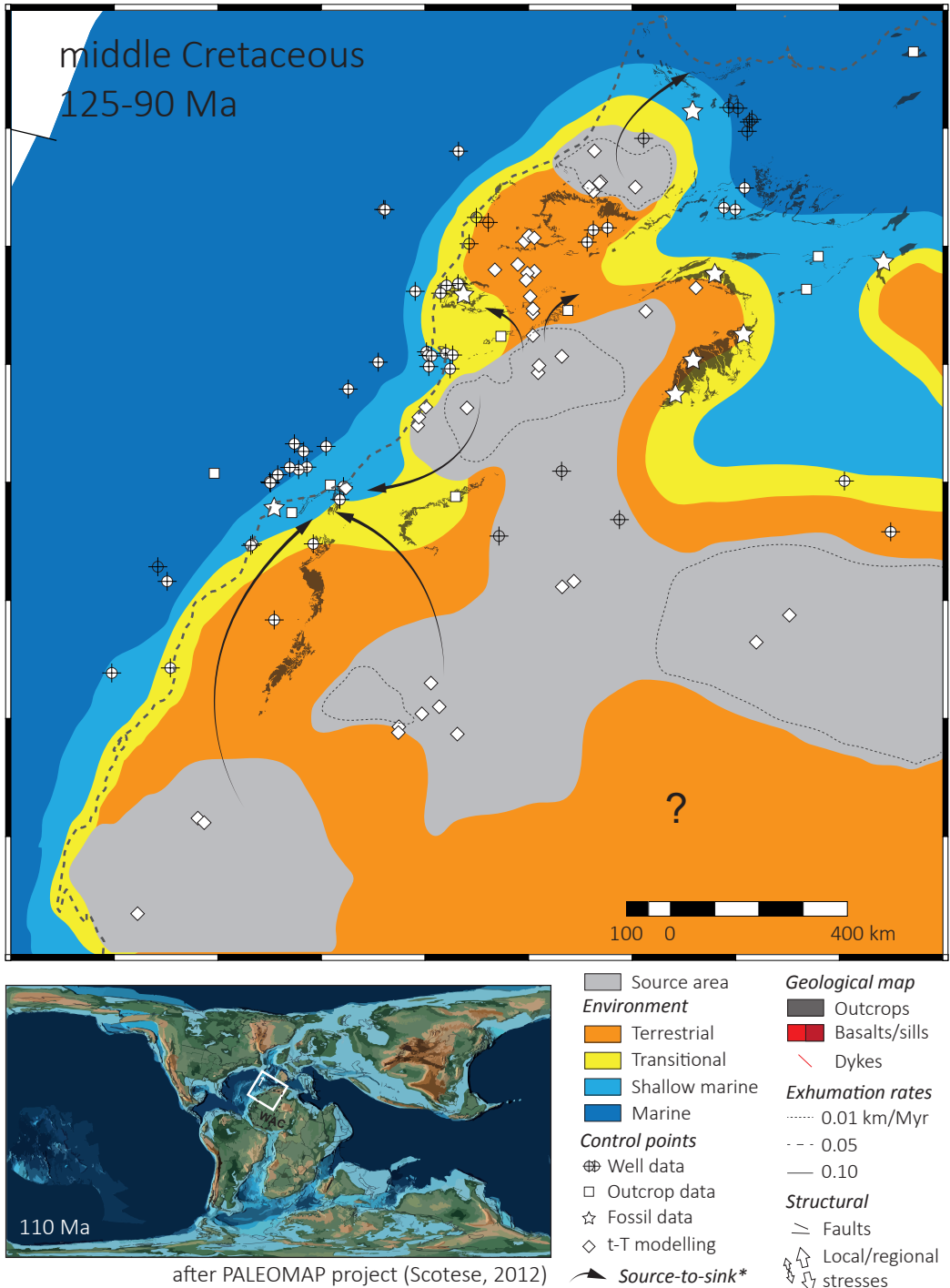
Figure 5.8. Middle Cretaceous map. * Simplified source-to-sink systems evidenced with provenance study or paleo-currents.
