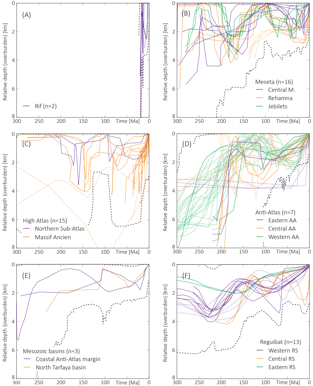
Figure 4.4. Time-depth curves converted from t - T curves shown in figure 4.2, assuming the geothermal gradient evolving as on figure 4.3 and assuming a surface temperature of 20°C. The bold lines are used for vertical movement rates calculations; non-selected curves in the background were also converted to depth; conditions for selection are in table 4.2. The upper and lower limits (thick dashed lines) are calculated with a geotherm of 40 and 20°C/km, respectively.
