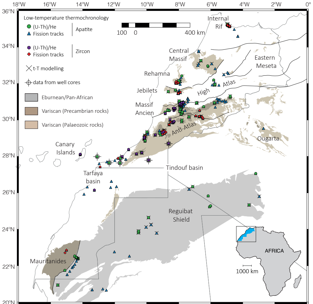
Figure 4.1. Location of LTT samples and t-T modelling (see references in table 4.1).
