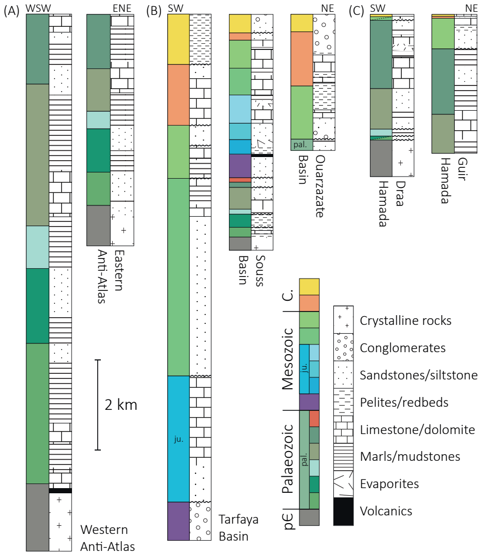
Figure 3.3. Simplified stratigraphic columns and dominant lithologies of the different regions of the Anti-Atlas and surrounding the belt, modified from the following studies. A) Anti-Atlas after Michard et al. (2008). B) Tarfaya basin after Ranke et al. (1982); Souss basin after Samaka and Bouhaddioui (2003); Ouarzazate basin after Ellero et al. (2012). C) Draa Hamada after Leprêtre et al. (2015) and Guerrak (1989); Guir Hamada after El Youssi (1993) and Robert-Charrue and Burkhard (2008).
