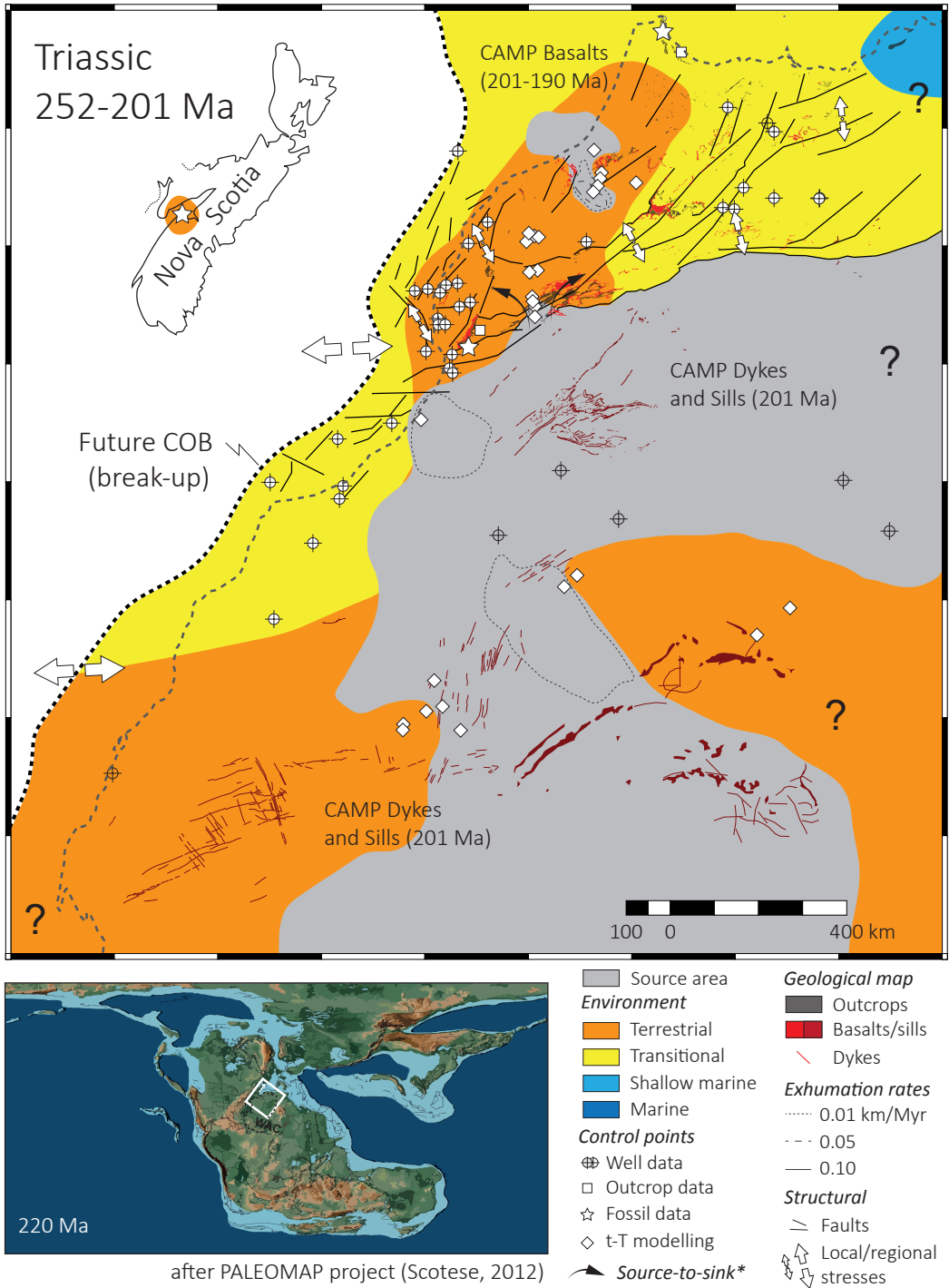
Figure 5.3. Triassic map. * Simplified source-to-sink systems evidenced with provenance study or paleo-currents. CAMP : Central Atlantic Magmatic province.
