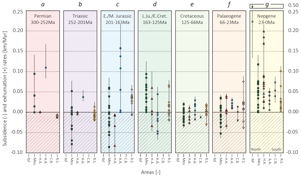
Figure 4.5. Exhumation and subsidence rates calculated from the 56 selected depth converted curves of figure 4.4 using the variable geotherms shown in figure 4.3. The seven defined periods a to g span between 300 and 0 Ma. The combined error bars are extracted from the results of rate calculations using a constant geotherm of 20°C/km and a surface temperature of 20°C. Mes : Meseta; HA : High Atlas; AA : Anti-Atlas; CB : Coastal Mesozoic basins; RS : Reguibat Shield. North and South are only marked for period g because Morocco has been significantly rotated since the Permian (e.g. Scotese, 2012).
