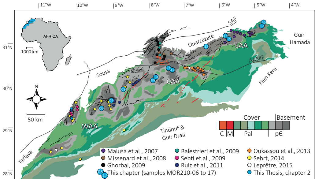
Figure 3.1. Geological map of the Anti-Atlas (modified and simplified from Hollard et al., 1985; Soulaïmani et al., 2014) with LTT sample location with references therein. WAA , CAA , and EAA : Western, Central, and Eastern Anti-Atlas, respectively; C : Cenozoic (Siroua Volcanism; ca. 10-5 Ma); M : Mesozoic (CAMP related Dykes; ca. 200-195 Ma); Pal : Palaeozoic; pE : Precambrian.
