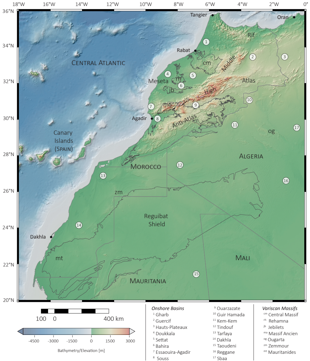
Figure 1.4. Geography of Morocco and its surroundings (data: GEBCO_2014_1D) with main geological domains, sedimentary basins, and Variscan Massifs superimposed.
