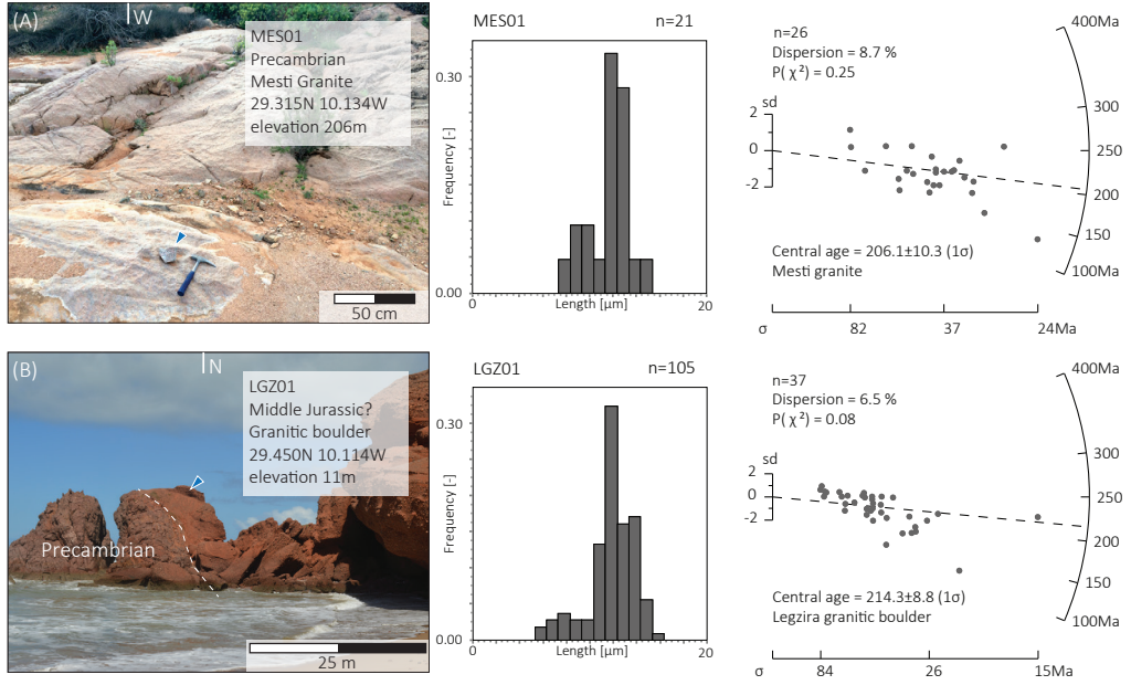
Figure 2.4. Sampled outcrops (left panel), track length distribution (central panel), and radial plots (bivariate scatterplots; right panel). Radial plots were made with RadialPlotter with Linear Transformation (Vermeesch, 2009). sd : Standard deviation; \sigma : Error with 1\sigma (Ma) (with precision given by 1/\sigma ); \chi^2 : Chi-square probability. A) Precambrian granite of the Sidi Ifni area exposed in a riverbed close to the city of Mesti, where MES01 was sampled. B) Middle Jurassic red beds (or older; Arantegui, 2018) lying unconformably on the Proterozoic basement, located north of the Lgizra village, and where LGZ01 was sampled.
