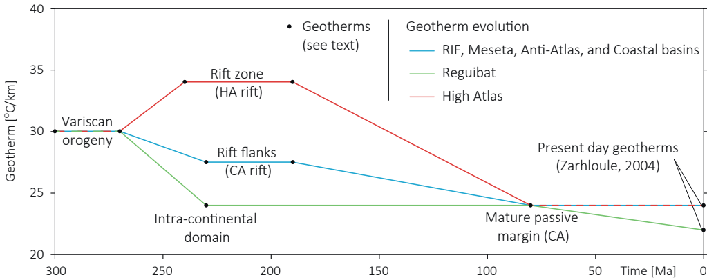
Figure 4.3. Geothermal gradients used for the depth conversion of the t - T curves. Geotherms: Geothermal gradients documented in literature, from present-day or recent settings similar to ones in Moroccan geological past. See description of the geotherms considered as analogues in the text.
