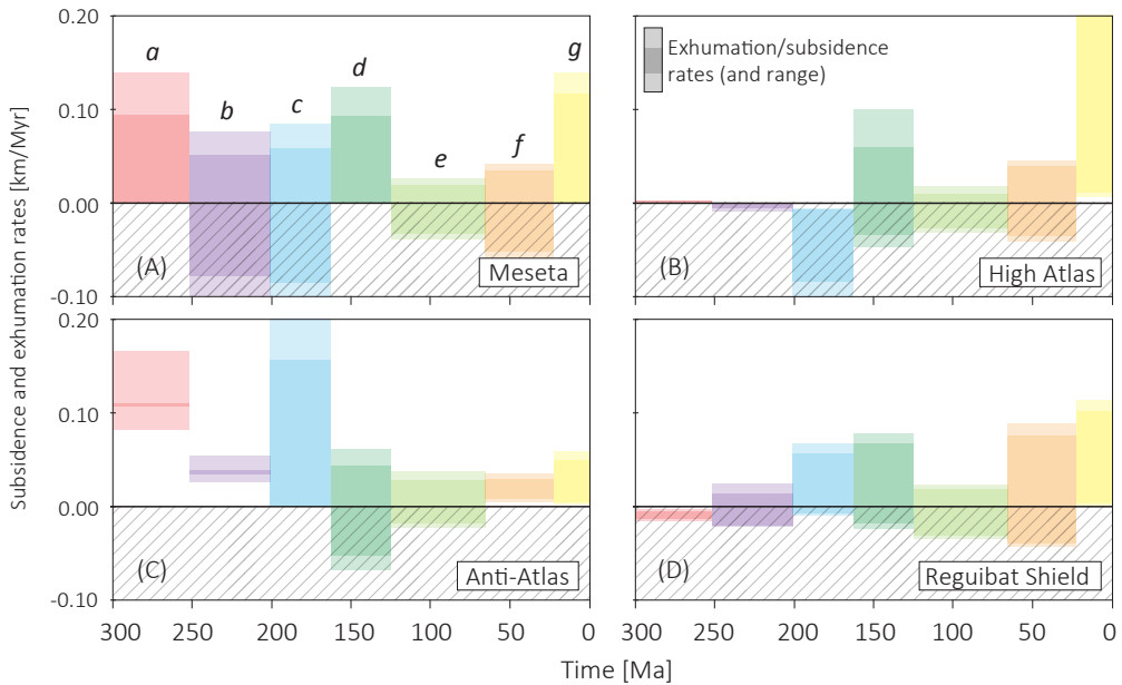
Figure 4.6. Evolution of the calculated exhumation and subsidence rates of basement rocks for the last 300 Ma in the A) Meseta, B) High Atlas, C) Anti-Atlas, and D) Reguibat Shield. Periods as defined in the text and rates as presented in figure 4.5.
