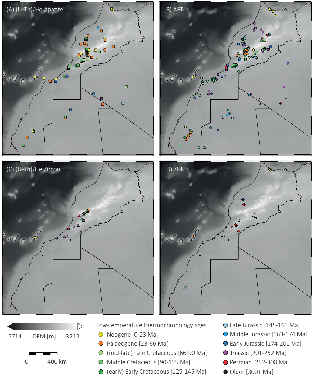
Figure 6.3. LTT cooling ages spatial pattern superimposed to the DEM (data: GEBCO_2014_1D). See complete list of references in chapter 4, table 4.1.
