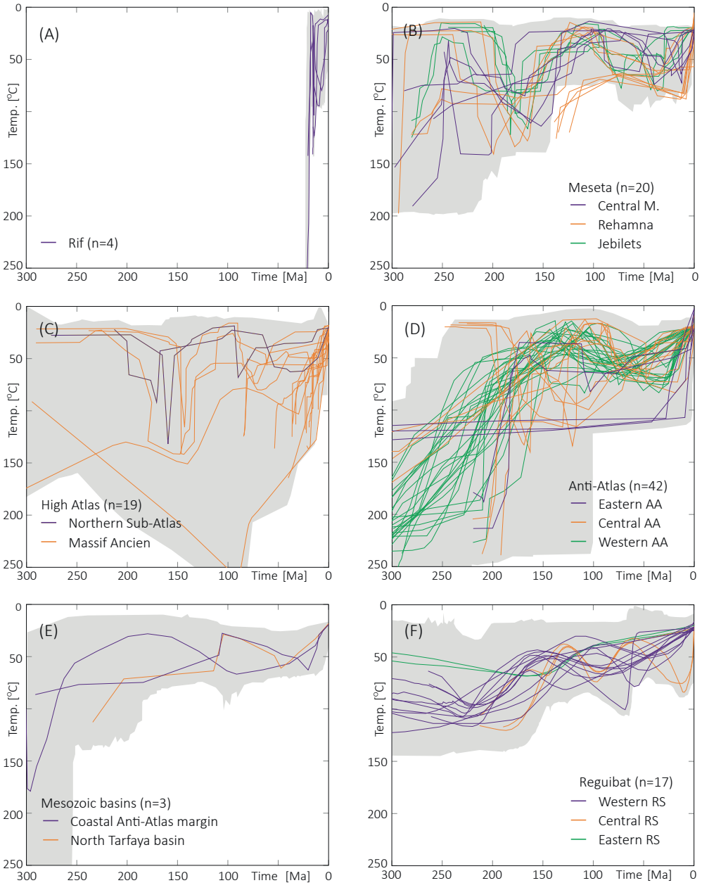
Figure 4.2. Digitized t - T modelling weighted averages, best-fit curves, and acceptable envelopes (grey area) for HeFTy results or expected curves, maximum likelihood curves and limits of 2\sigma confidence level (grey area) for QTQt results (see references in table 4.1). t - T results for borehole samples from Sehr (2014), as well as results from El Haimer (2014) and Barbero et al. (2007), for which only envelopes were published, are not digitized.
