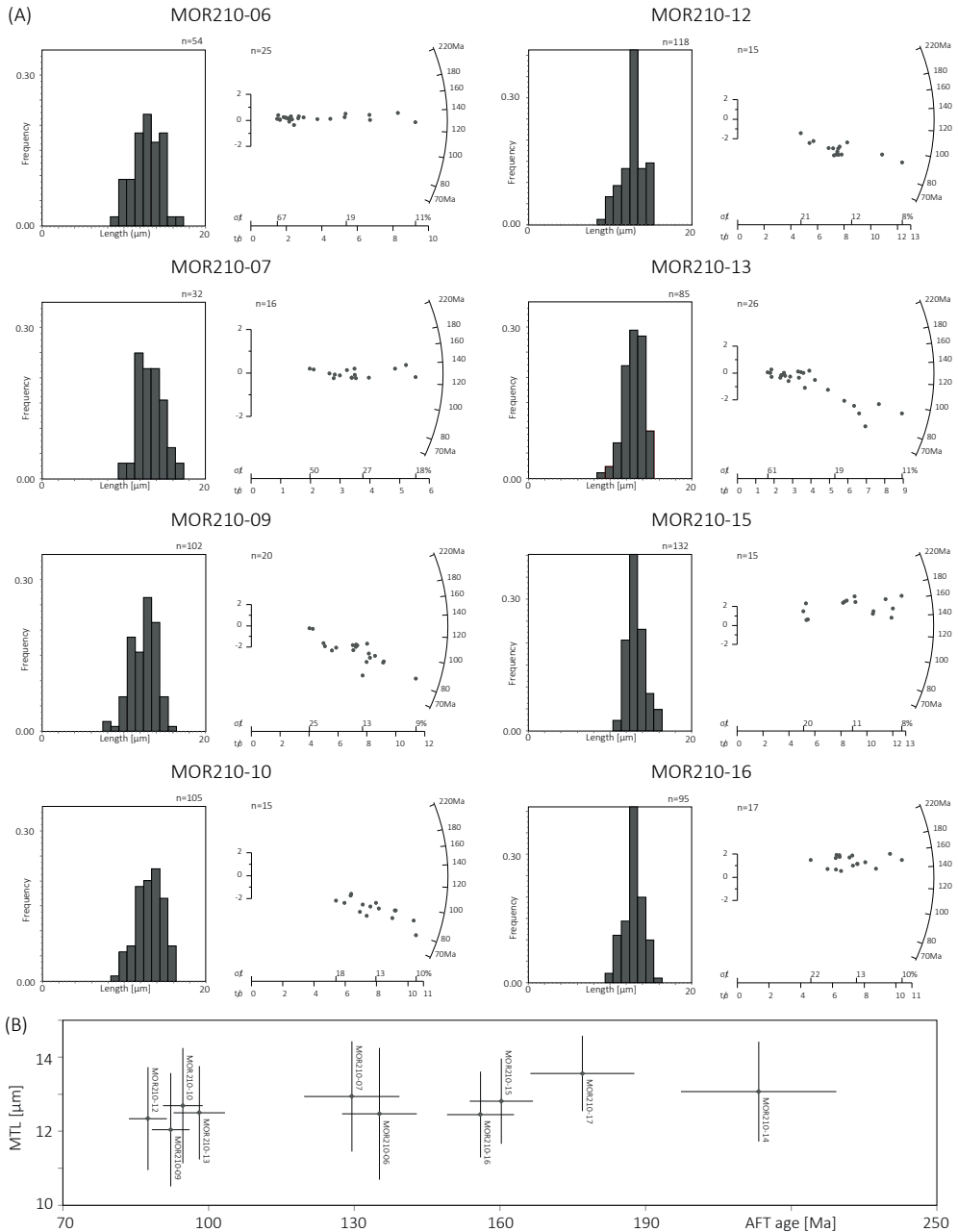
Figure 3.5. A) Track length distribution (left panel) and radial plot (right panel) for 8 out of 12 samples; B) Mean track length (MTL) as a function of apatite fission tracks ages (AFT).
