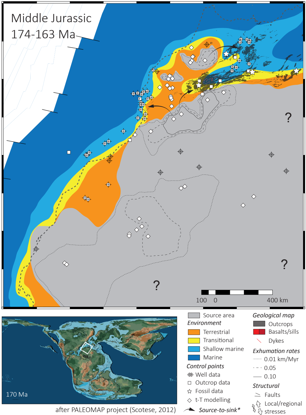
Figure 5.5. Middle Jurassic map. * Simplified source-to-sink systems evidenced with provenance study or paleo-currents.
