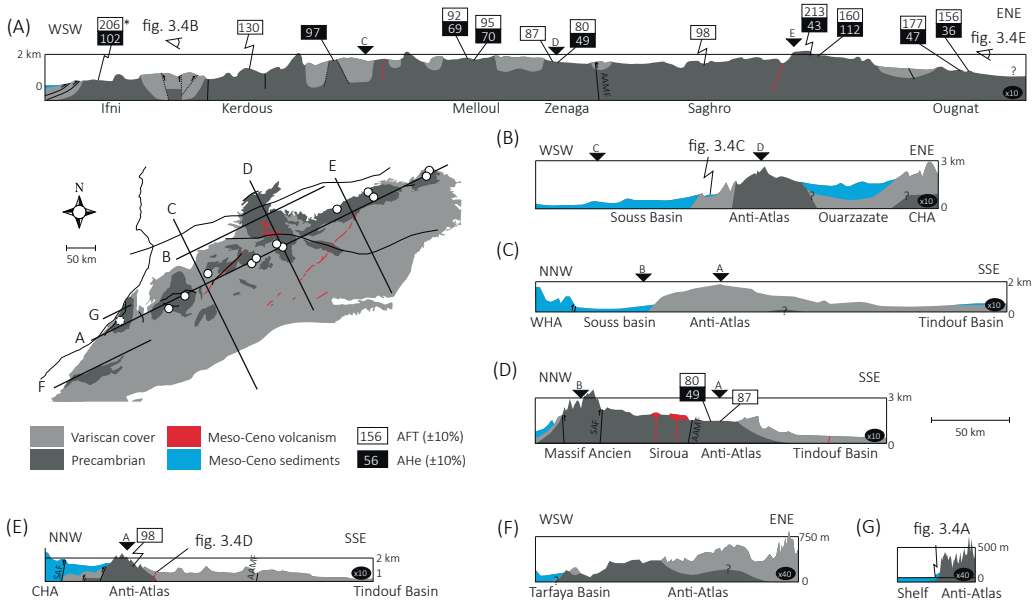
Figure 3.2. Geological cross-sections of the Anti-Atlas built from the geological map (including cross-sections; Hollard et al., 1985) and published cross-sections (see references thereafter). The position of the cross-sections and the LTT ages are shown on the map. Elevation profiles extracted from Google Earth; vertically exaggerated 10 times for A to E and 40 times for F and G. Cross-sections A, B, F, and G are parallel to the trend of the belt; Cross-sections C, D, and E are perpendicular to the trend of the belt. A) Cross-section from the Ifni inlier to the Ougnat inlier (after Soulaïmani et al., 2008; Raddi et al., 2007). *LTT ages from chapter 2. B) Cross-section between the Souss and Ouarzazate basins; CHA: Central High Atlas. C) Cross-section along the western Anti-Atlas; WHA: Western High Atlas (after Soulaïmani et al., 2008). D) Cross-section along the central Anti-Atlas (after Missenard et al. 2008; Balestrieri et al., 2009). E) Cross-section along the eastern Anti-Atlas (after Jossen and Filali Moutei, 1988; Robert-Charrue 2006; Malusà et al., 2007; Soulaïmani et al., 2008; Raddi et al., 2007). F) Cross-section along Tarfaya Basin and Bas Braa (after Soulaïmani et al., 2014). G) Cross-section along the Sidi Ifni continental shelf and the Ifni inlier (after Sebti, 2011).
