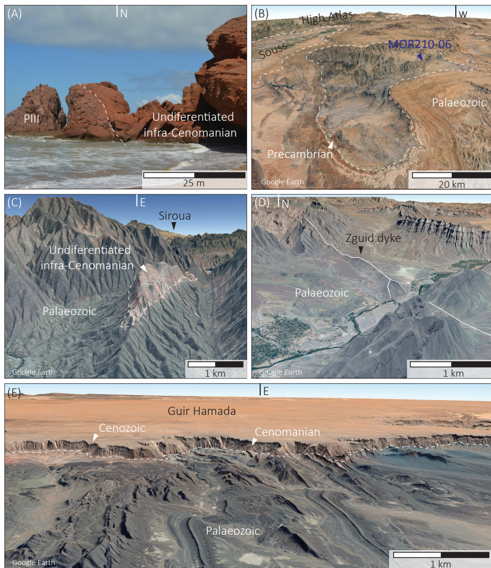
Figure 3.4. A) Undifferentiated infra-Cenomanian (Yazidi et al., 1991) lying with unconformity on the Precambrian basement (Pill: Proterozoic), located north of the Lgezira village (see the previous chapter for re-dating of these redbeds to the Jurassic) B) Precambrian outcrops of the Anti-Atlas (Kerdous inlier) in which MOR210-06 was sampled. C) Undifferentiated clastic infra-Cenomanian overlying the Variscan Palaeozoic sediments. D) CAMP Zguid dyke, south of the Saghro Precambrian dome (or inlier), crosscutting a syncline of the Anti-Atlas Palaeozoic. E) Eastern termination of the belt, plunging under the Cenomanian to Cenozoic Guir Hamada. B-E) Google Earth scenes with vertical exaggeration of 3 (positions on cross-sections in figure 3.2).
