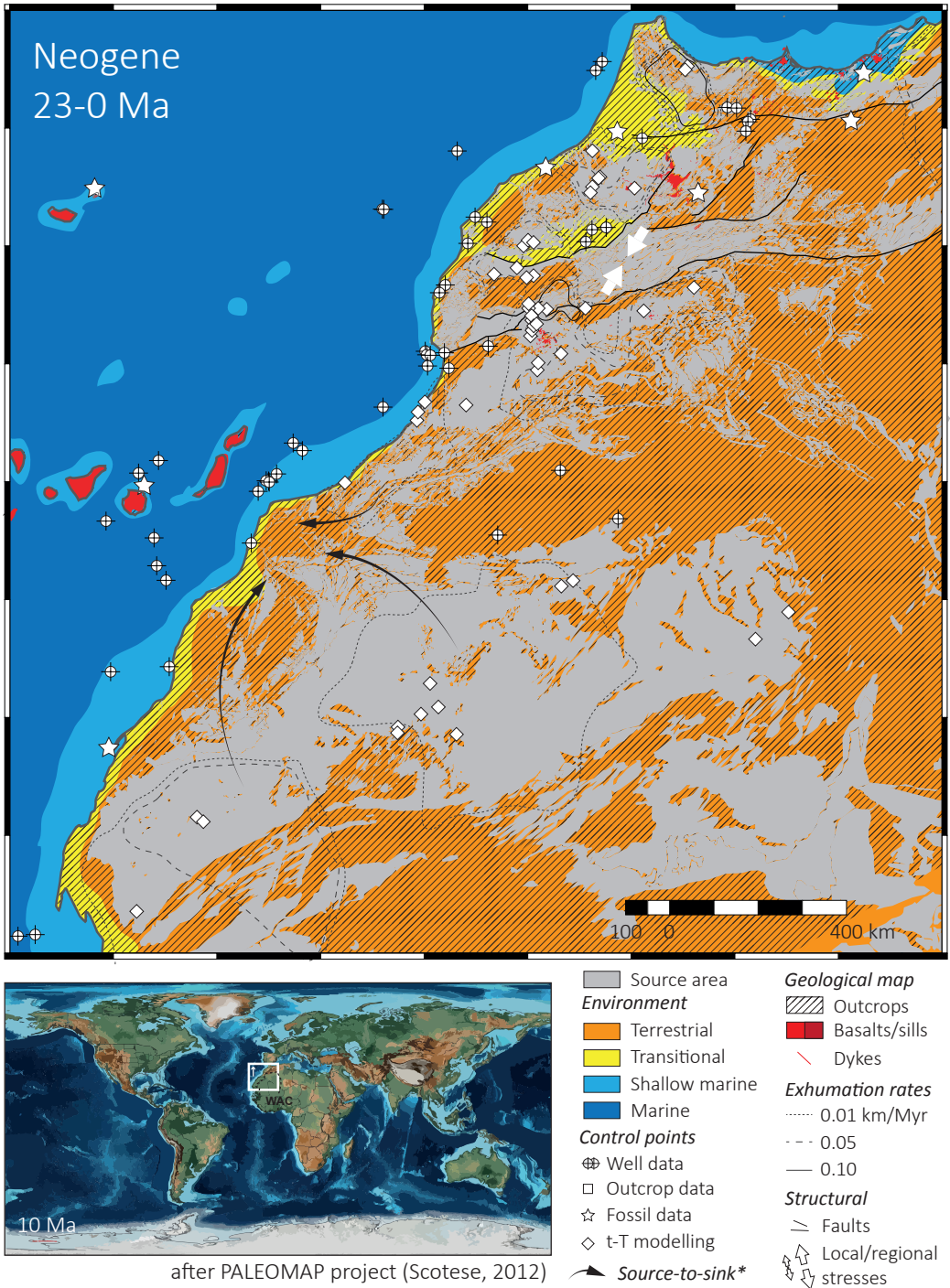
Figure 5.11. Neogene map. * Simplified source-to-sink systems evidenced with provenance study or paleo-currents.
