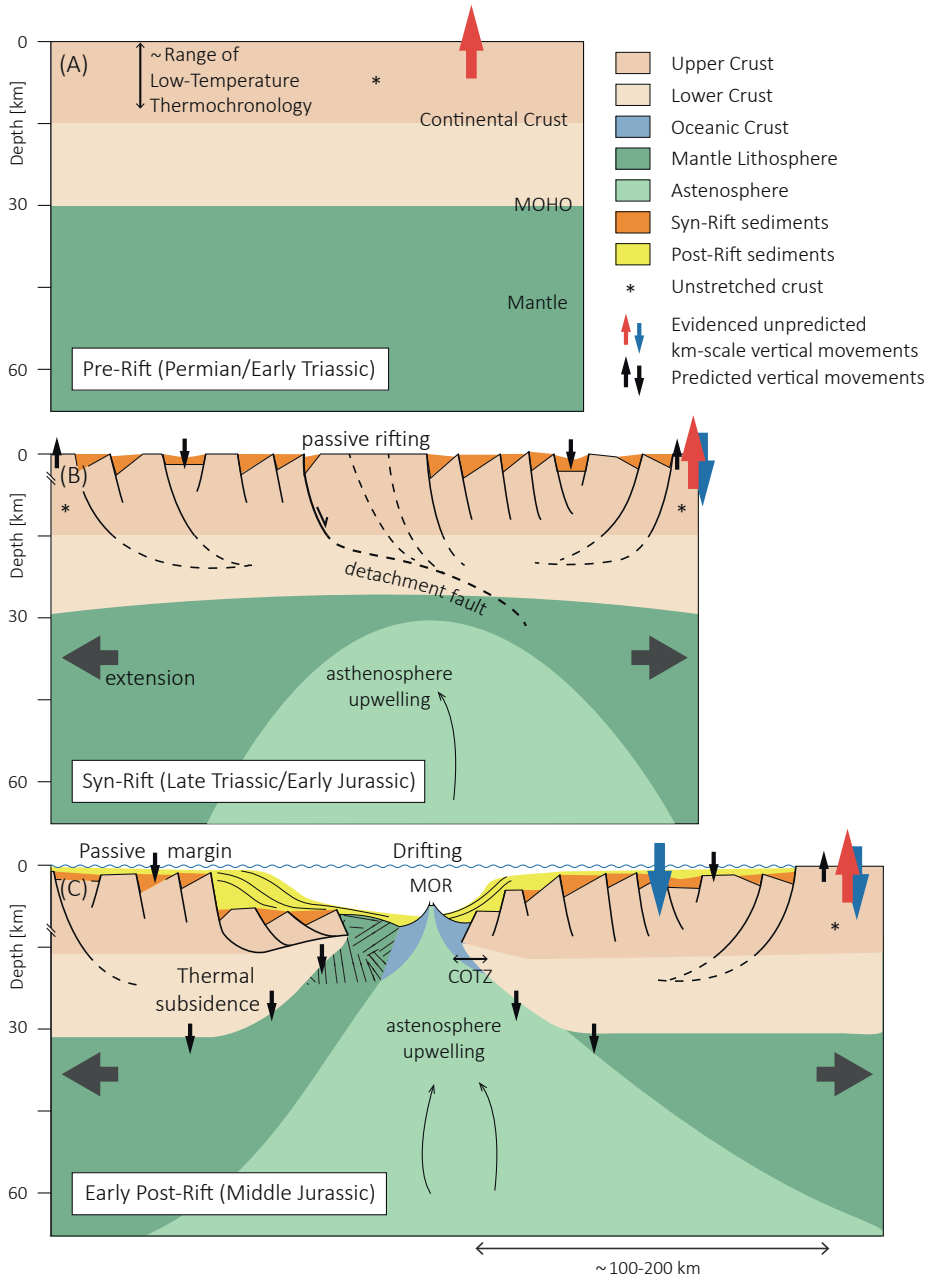
Figure 1.2. Summary of the unexpected km-scale vertical movements observed in the Central Atlantic margins and their adjacent continental crusts (after Gouiza et al., 2010). A), B), and C) Pre-, Syn- and post-rift situations, respectively. MOR : Mid-Oceanic Ridge (spreading centre); COTZ : Continent-Ocean Transition Zone.
