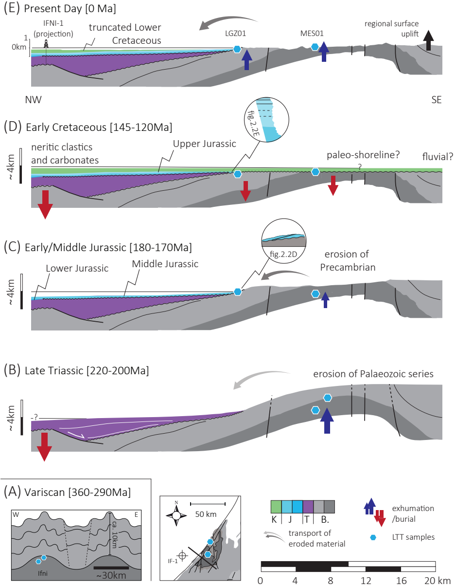
Figure 2.7. Conceptual model of the geological evolution of the Sidi Ifni transect; A) Situation at the end of the Variscan orogeny to E) present-day architecture of the Sidi Ifni margin simplified from figure 2.3. Vertical movements estimated from t-T modelling results of MES01 and LGZ01 and backstripping of the Ifni-1 well (in Gouiza, 2011). The description of each stage is in the text. Horizontal scale is for B) to E) (no vertical exaggeration). B: Undifferentiated basement offshore and Precambrian/Palaeozoic basement onshore; T: Triassic/Permian; J: Lower, Middle, and Upper Jurassic; K: Cretaceous. Thickness in the offshore domain is here estimated from Ifni-1 well, hence no Early Jurassic at the well position was considered.
