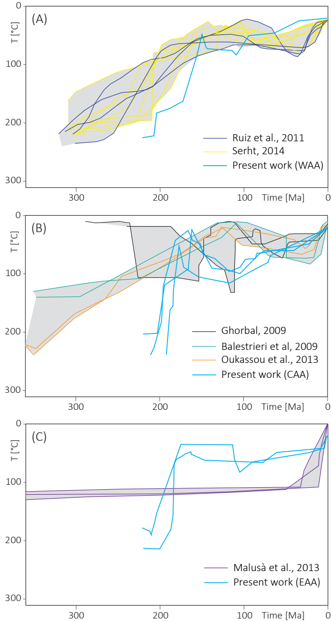
Figure 3.11. Best fit curves of t - T models from the literature (thin lines) and our simulations (thick blue lines) for the regions investigated in the present work: A) Western Anti-Atlas; B) Central Anti-Atlas; C) Eastern Anti-Atlas. Grey envelopes are framing the best-fit models from the literature (see references in the figure).
