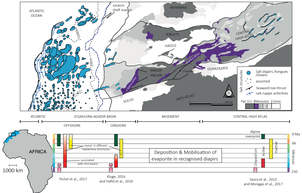
Figure 7.1. Comparison of salt activities in the salt basins of Morocco. Pal. (+) : Palaeozoic and older, T : Triassic, J : Jurassic, C : Cretaceous, and Ceno : Cenozoic. The Jurassic shelf margin is after Hafid et al., 2010. Salt bodies distribution in the offshore domain is after Pichel (in preparation).
