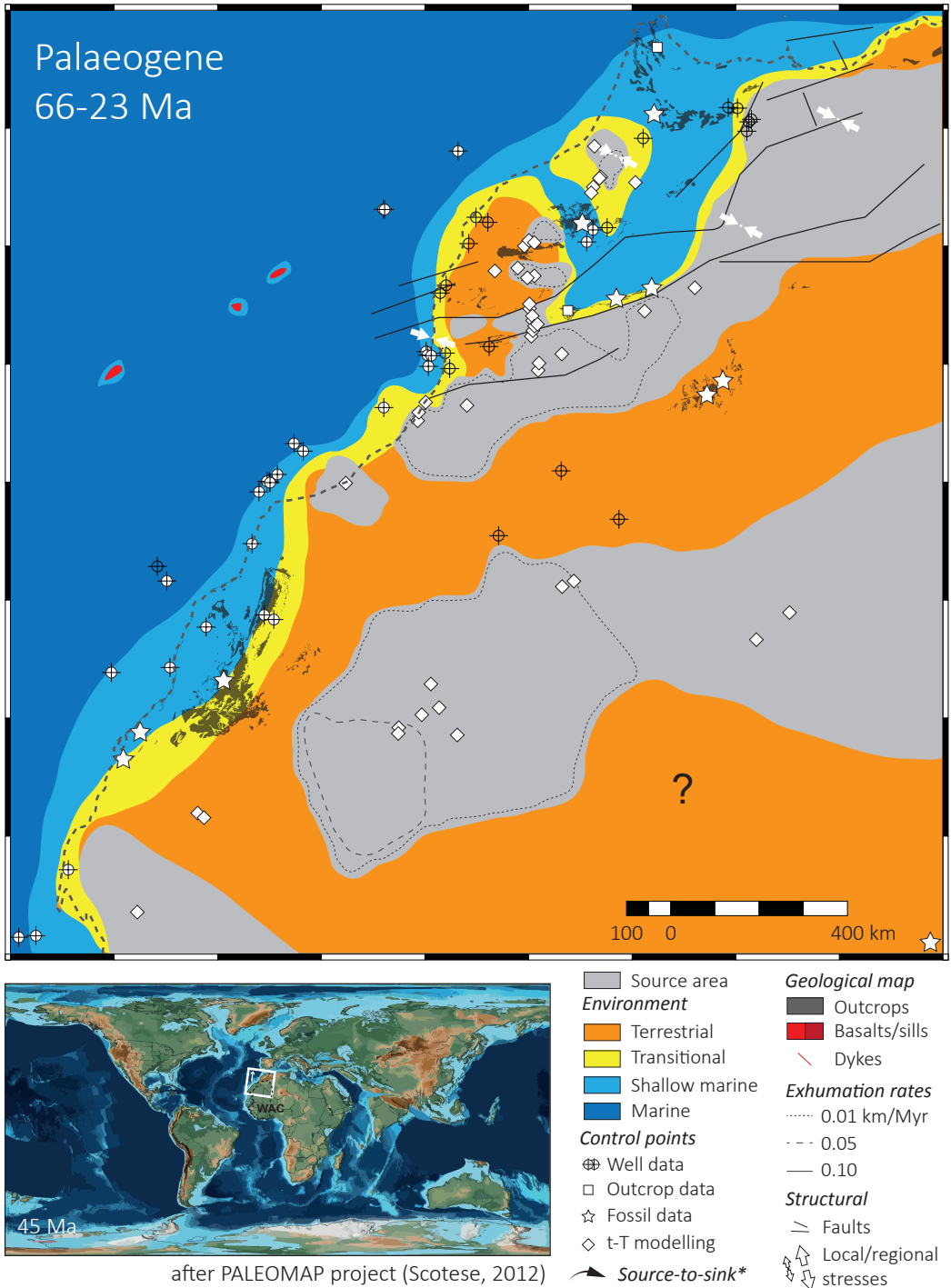
Figure 5.10. Palaeogene map. * Simplified source-to-sink systems evidenced with provenance study or paleo-currents.
