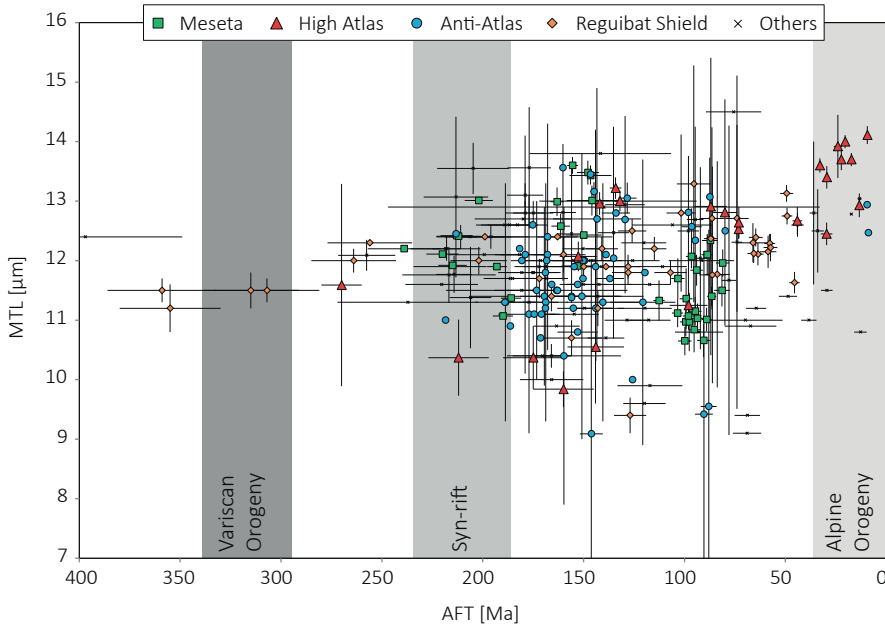
Figure 6.5. MTL vs AFT age plot for Morocco and its surroundings.
