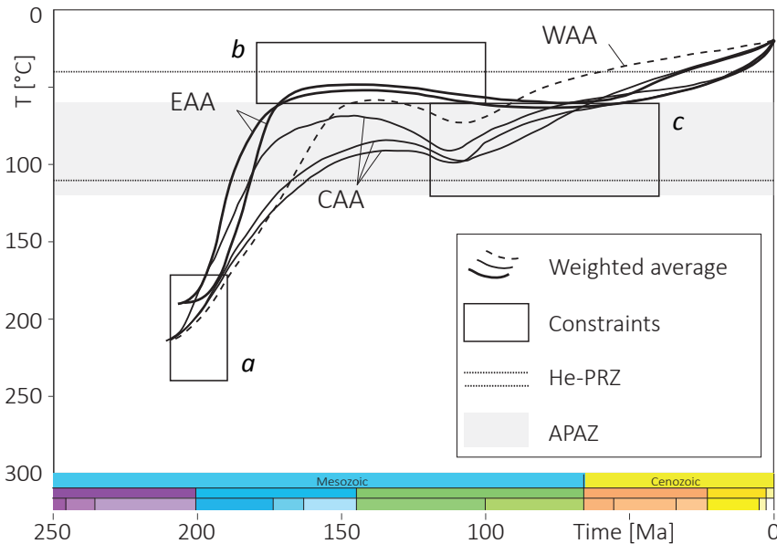
Figure 3.10. Weighted average curve from t - T modelling results shown in fig. 3.9; WAA, CAA, and EAA: Western, Central, and Eastern Anti-Atlas. See modelling parameters in table 3.4.
