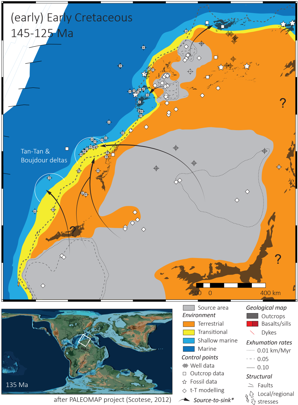
Figure 5.7. (Early) Early Cretaceous map. * Simplified source-to-sink systems evidenced with provenance study or paleo-currents.
