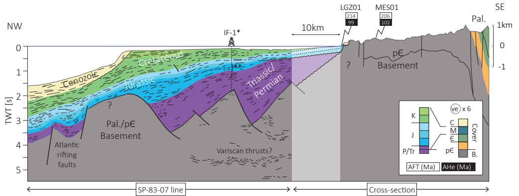
Figure 2.3. The Sidi Ifni transect: Composite cross-section running through the Sidi Ifni area, based on the interpretation of the 2D seismic line SP-83-07 from Gouiza (2011) and from the geological map from Hollard et al. (1985). The seismic line ends ca. 10 km before the shoreline. The gap (dashed line in figure 2.1A) was interpolated from the seismic interpretation and the geological map; the LTT ages are projected. * IF-1 is projected on the basement high at 2 second (TWT). ** The well report does not document Lower Jurassic sediments but only Triassic and Middle Jurassic. C: Cenozoic; M: Mesozoic (K: Cretaceous; J: Jurassic; Tr: Triassic); P: Permian; E: Cambrian; pE: Precambrian.
