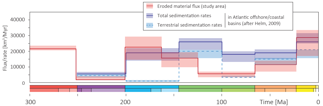
Figure 4.10. Comparison of the total eroded material flux to sedimentation rates in Moroccan offshore and coastal basins (after Helm, 2009).
