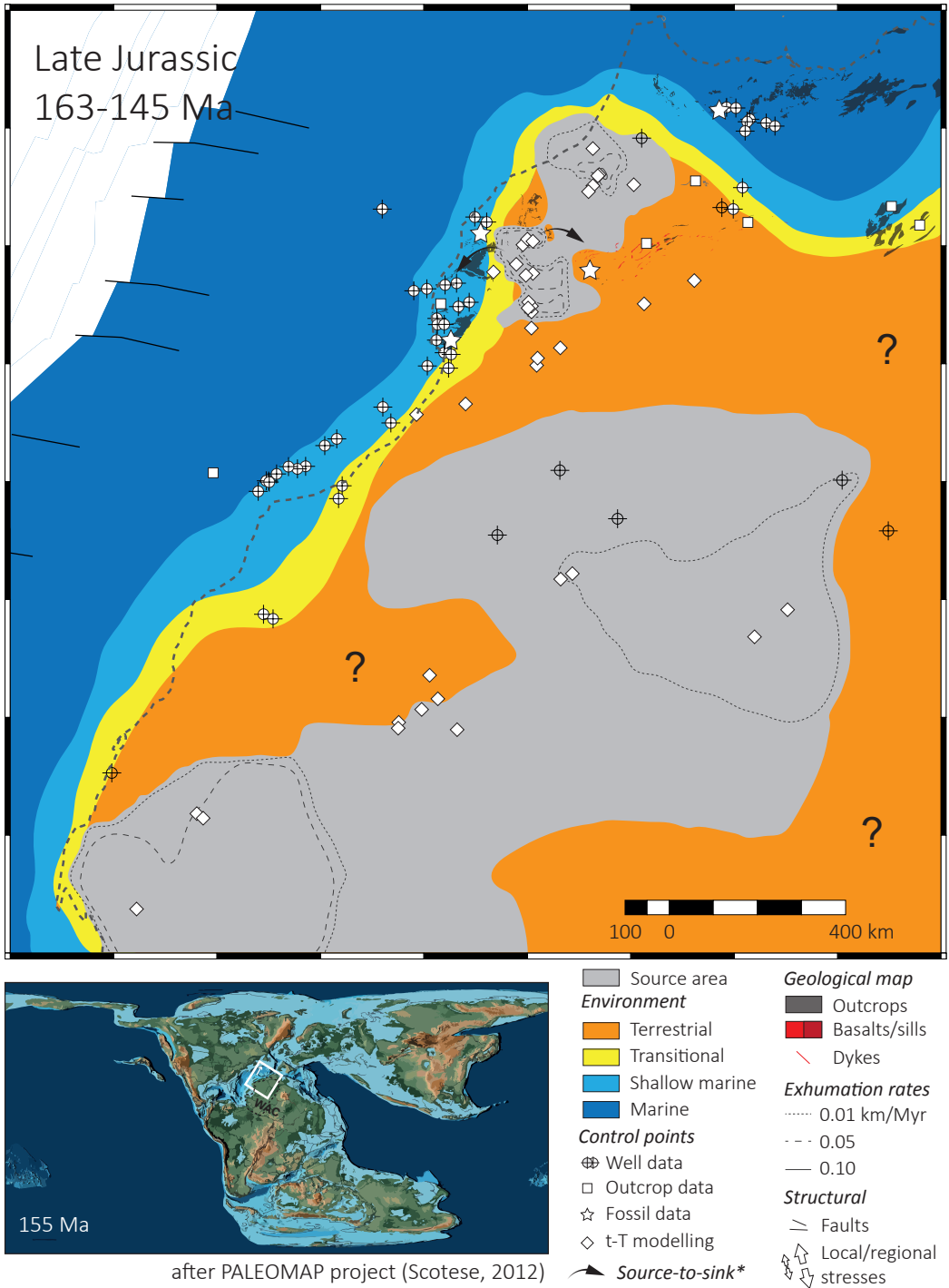
Figure 5.6. Late Jurassic map. * Simplified source-to-sink systems evidenced with provenance study or paleo-currents.
