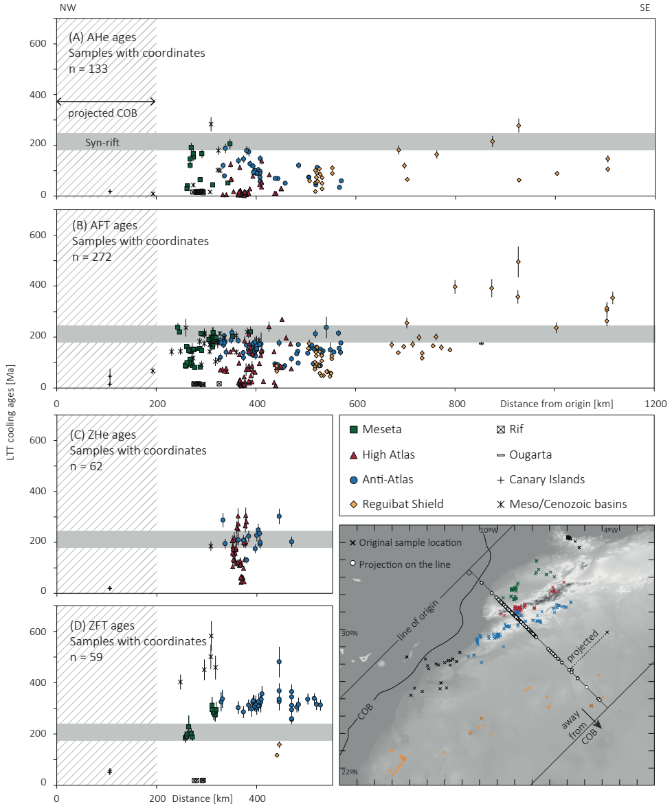
Figure 6.4. LTT ages orthogonally projected along a NW/SE trending line. The line runs perpendicular to the COB (orientation of a trend line offshore Morocco is ca. 47^\circ\text{N} ). The position of the COB is after Miles et al., 2012. The location of the projection line on the map is for illustration purpose only. Median ages are used for AHe and ZHe. Only the produced ages of shallowest samples from boreholes were plotted.
