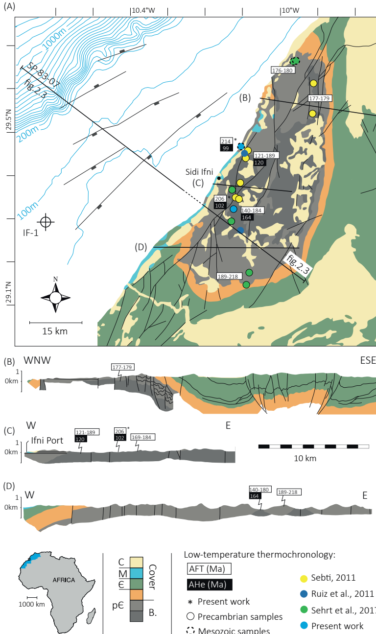
Figure 2.1. A) Simplified geological map of the Sidi Ifni area (after Hollard et al., 1985) and LTT data localisation (Sebti, 2011; Ruiz et al., 2011; Sehrt et al., 2017; present study). Bathymetry contour lines are every 50 m. Syn-rift offshore normal faults are from Le Roy and Piqué (2001). C: Cenozoic; M: Mesozoic; E: Cambrian; pE: Precambrian; AFT: Apatite fission track ages; AHe: (U-Th)/He dating on apatites. B-D) Geological cross-section of the Sidi Ifni area (after Yazidi et al., 1986; 1991) onto which we projected LTT ages.
