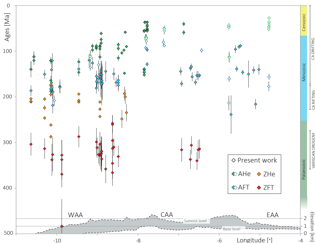
Figure 3.7. LTT data from the Anti-Atlas (references in figure 3.1). The elevation plot (bottom plot) is made from the point extraction from a DEM (SRTM 90m, NASA) of the Anti-Atlas reliefs. Timing of the geological events (right panel) are from Michard et al. (2008). CA : Central Atlantic; CAMP : Central Atlantic Magmatic Province.
