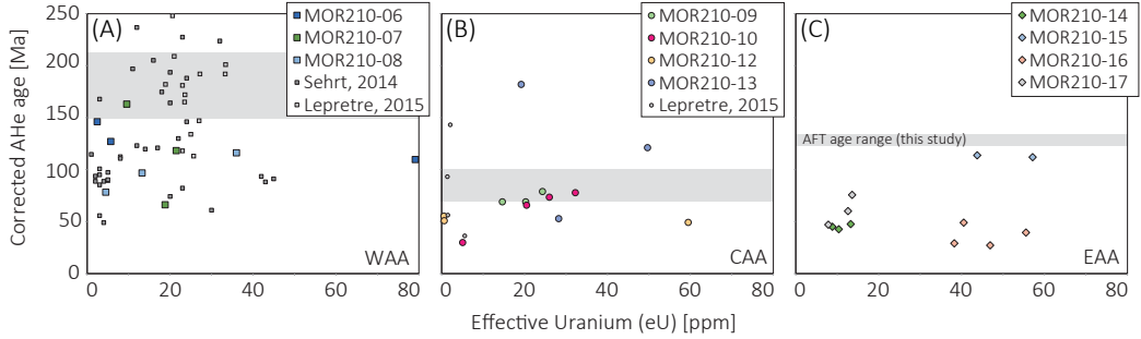
Figure 3.6. Corrected AHe ages v. effective uranium concentration plots for the A) Western, B) Central, and C) Eastern Anti-Atlas.
