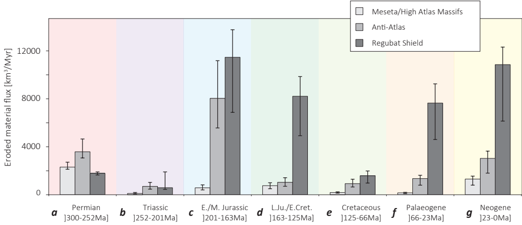
Figure 4.9. Estimated eroded material flux for the three main sediment sources (Meseta/High Atlas, Anti-Atlas, and Reguibat Shield) for the seven defined periods (a-g). The eroded material flux is obtained with variable geotherms (fig. 4.3), while the ranges are given by calculations done with two constant geotherms of 20 and 40°C/km. See the text for a estimation of the error bar associated to our workflow.
