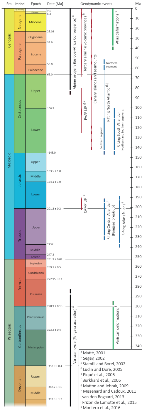
Figure 1.6. Tectonic chart of the Atlantic realm and Morocco, see references therein (ages after ICS 2016/12). LIP : Large Igneous Province; CAMP : Central Atlantic Magmatic Province; PAAP : Peri-Atlantic Alkaline Pulse.
