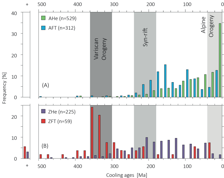
Figure 6.2. Temporal distribution of LTT ages produced in Morocco and surrounding (plotted in bins of 20 Myr). See all references in table 4.1. Results of thermochronology on A) apatite and B) zircon crystals.
