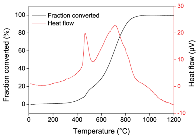
Figure 3.1: Heat flow and mass gained signals for the 5 \mu\text{m} powder oxidized at 5 °C/min in dry synthetic air.
