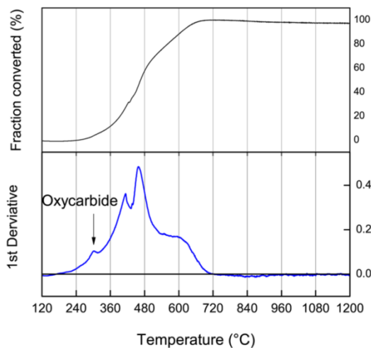
Figure 3.6: Differentiated mass gain signal ( d\Delta m/dt ) of 0.8 µm TiC powder recorded with 5 °C/min in dry synthetic air.
