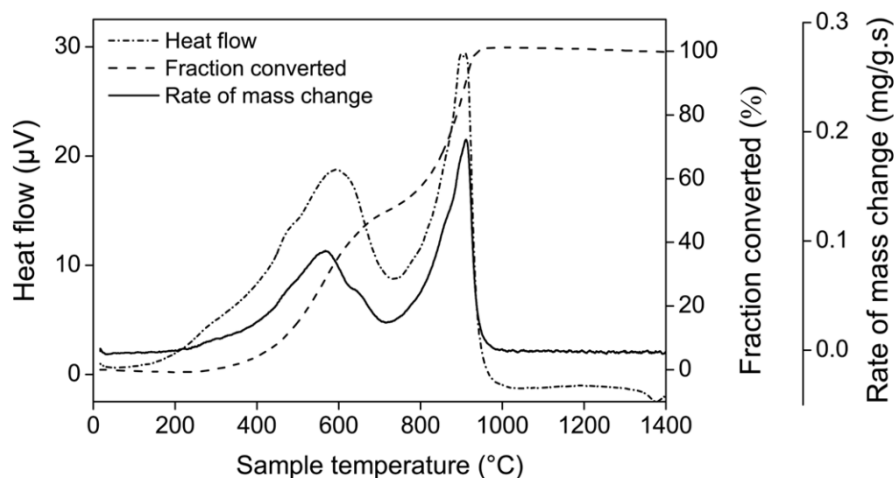
Figure 6.4: Oxidation kinetics of \text{Ti}_2\text{AlC} powder in air at 4 °C/min: heat flow, fraction converted and rate of mass change (recorded mass change differentiated) versus temperature.
