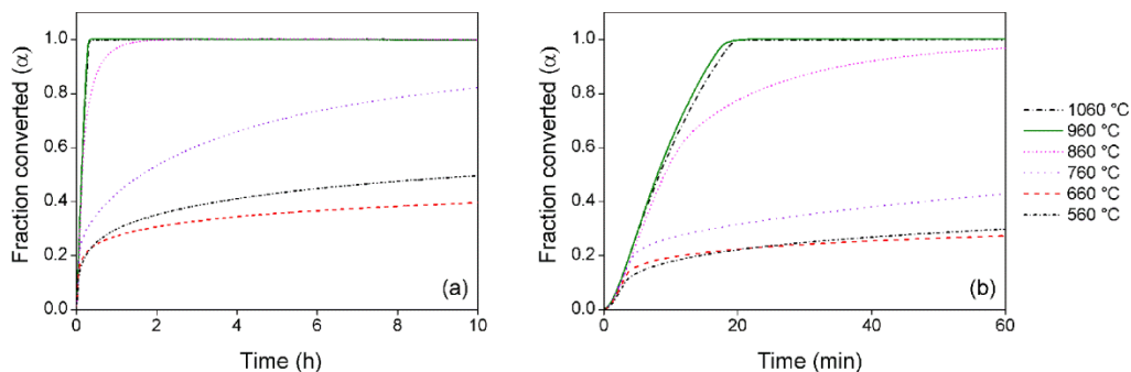
Figure 6.5: (a) Isothermal conversion of \text{Ti}_2\text{AlC} at different oxidation temperatures for 10 h in dry synthetic air as determined from thermogravimetric analysis, (b) enlargement showing the first hour.
