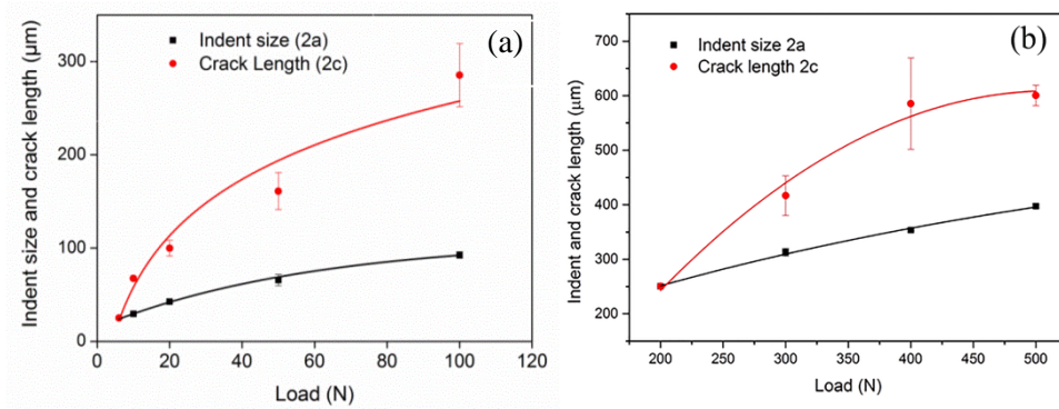
Figure 7.1: Vicker's indent size and crack length versus applied load of (a) \text{Al}_2\text{O}_3 with 20 vol. % TiC composite and (b) Fine grained \text{Cr}_2\text{AlC} .
