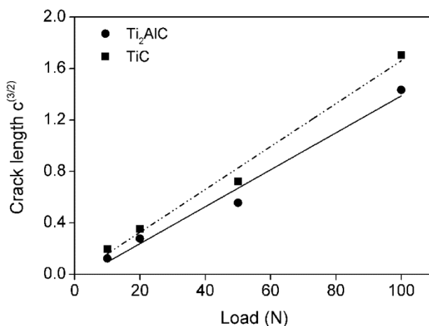
Figure 6.7: Comparison of the length of Vickers' indentation induced cracks with length c generated in \text{Al}_2\text{O}_3/\text{Ti}_2\text{AlC} and \text{Al}_2\text{O}_3/\text{TiC} composite [23].
