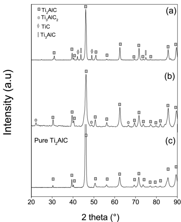
Figure 6.2: Diffractograms showing purity levels of the sintered material (a) \text{Ti}_2\text{AlC} with \text{TiC} and \text{Ti}_3\text{AlC} impurities (b) \text{Ti}_2\text{AlC} having \text{Ti}_3\text{AlC}_2 impurities and (c) pure \text{Ti}_2\text{AlC} .
