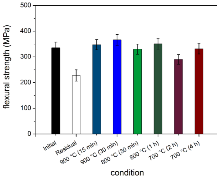
Figure 4.16: Room temperature flexural strength values of the \text{Al}_2\text{O}_3 -Ti composites before, after indentation damage and after healing at the indicated temperature-time combinations.
