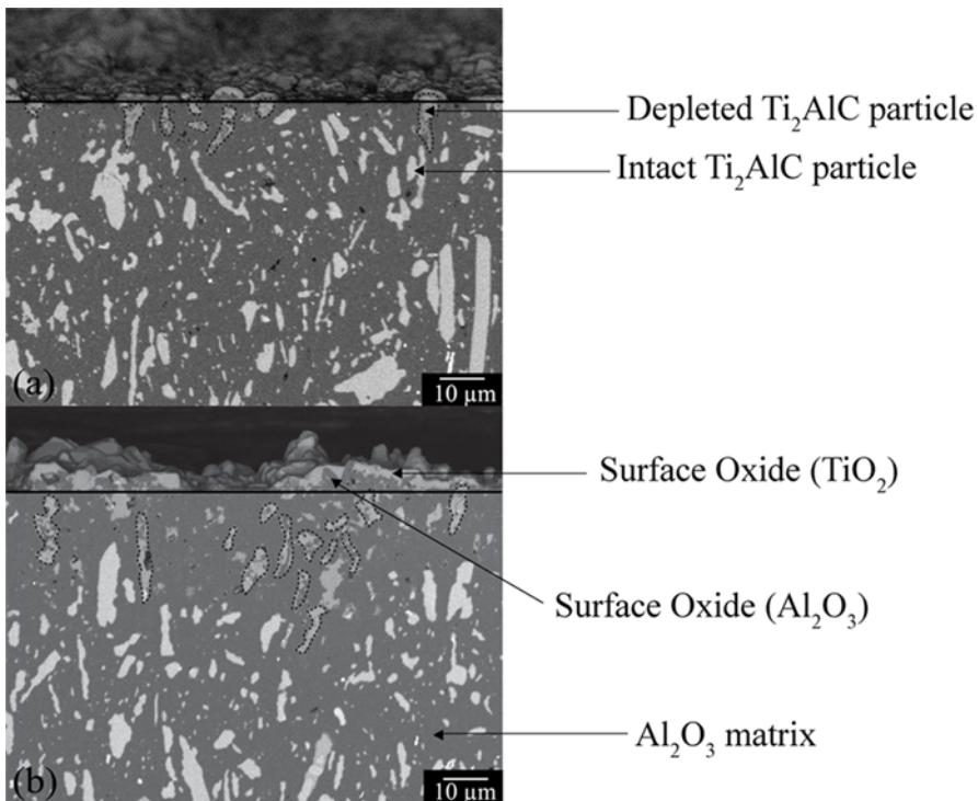
Figure 6.12: SEM cross sectional view of the composite at 1000\text{ }^\circ\text{C} in air for (a) 64 and (b) 256 h showing the depletion of Ti and Al from the \text{Ti}_2\text{AlC} particles close to the sample surface.
