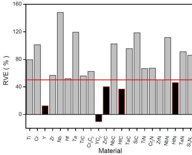
Figure 2.4: Relative volume expansion upon oxidation of viable healing particles.
