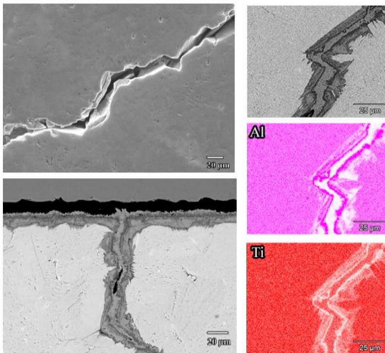
Figure 7.6: (a) Cracks in \text{Ti}_2\text{AlC} -a after quenching in water from 850 °C; (b) Cross-section of healed crack after exposure to combustion conditions for 4 h; (c) Close up of healed crack; (d) Al X-ray map; (e) Ti X-ray map.
