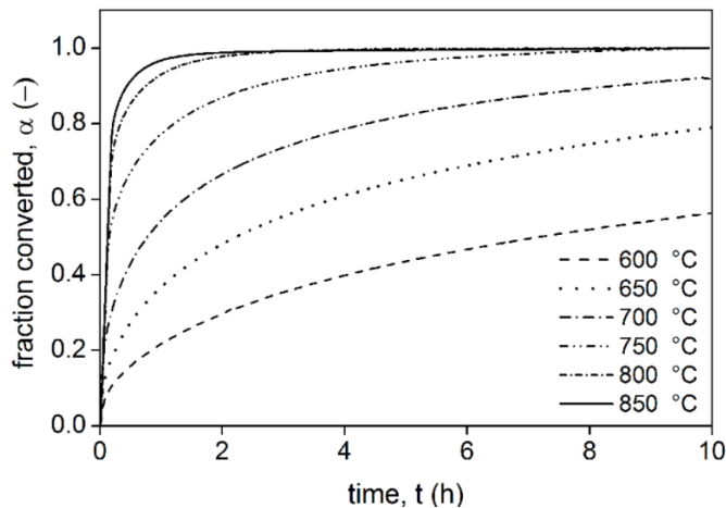
Figure 4.3: Fraction of Ti powder converted to \text{TiO}_2 \alpha , in dry synthetic air as a function of time for different annealing temperatures.
