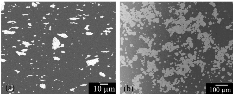
Figure 4.2: Microstructure of the \text{Al}_2\text{O}_3 -Ti composite showing the distribution of Ti (white phase) in alumina produced with (a) and without (b) adding the surfactant Dolapix.
