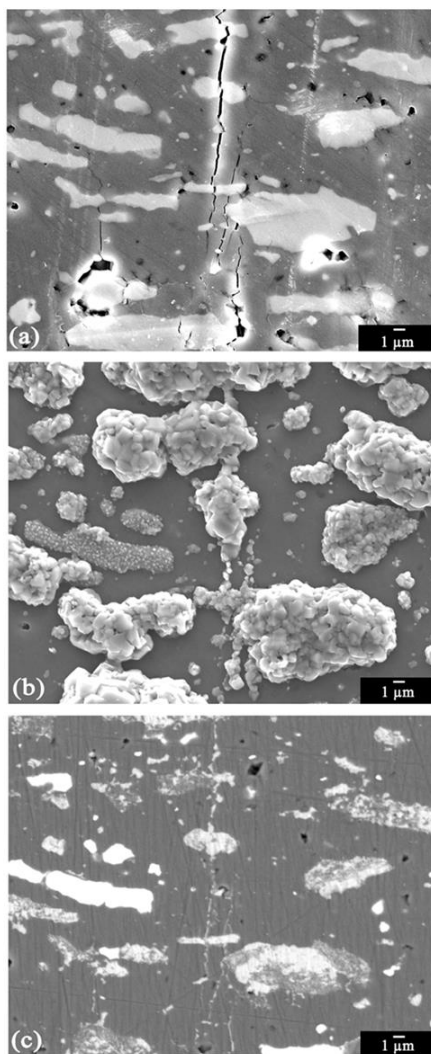
Figure 6.11: SEM images of the same crack area before and after healing at 1000 °C for 1 h in air. (a) Before oxidation (b) After oxidation before polishing (c) Polished surface showing fully filled cracks.
